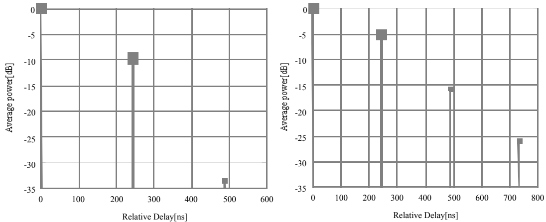
(a) Indoor office Channel A
