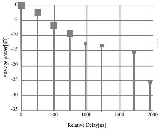
(e) Vehicular Channel A
