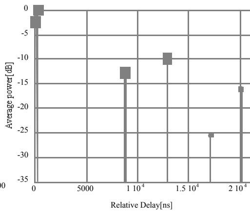
(f) Vehicular Channel B
