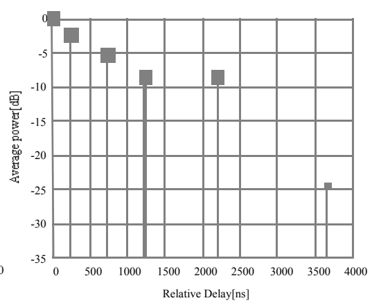
(d) Outdoor to indoor and pedestrian Channel B
