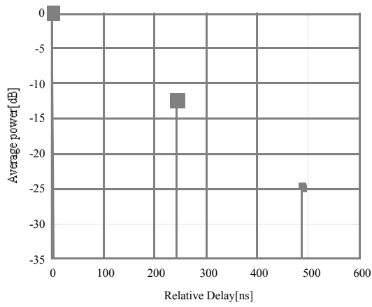
(c) Outdoor to indoor and pedestrian Channel A
