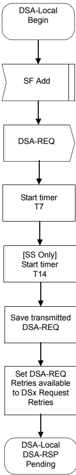
Figure 118—DSA—Locally Initiated Transaction Begin state flow diagram
