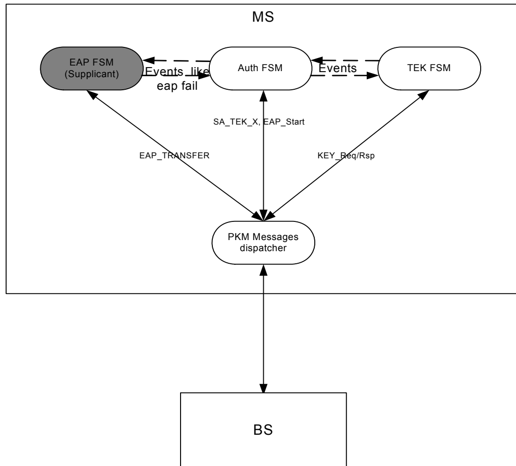
Figure 164—System relationships in security related FSM
