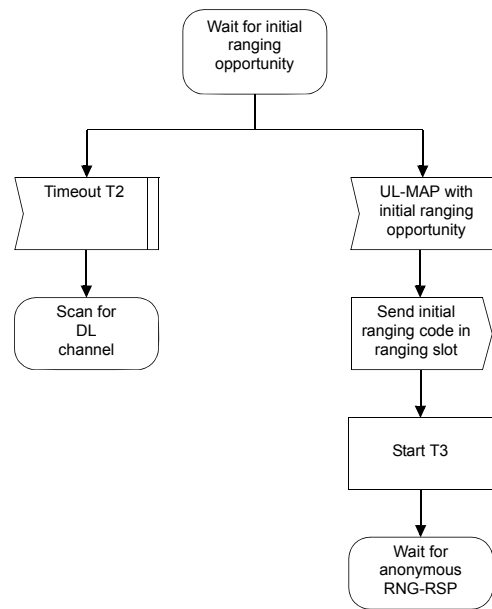
Figure 93—CDMA initial ranging—SS (part 1)
