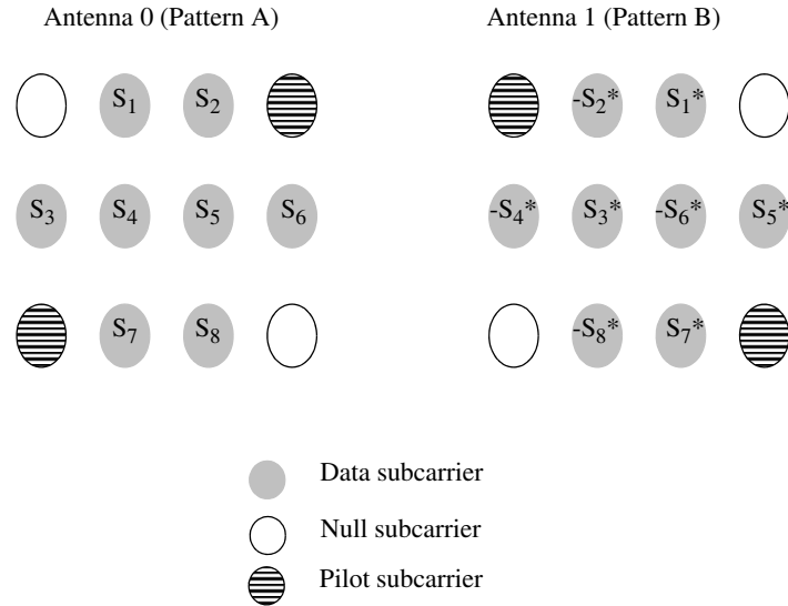
Figure 263—Mapping of data subcarriers in STTD mode
