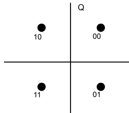
Figure 190—QPSK constellation
