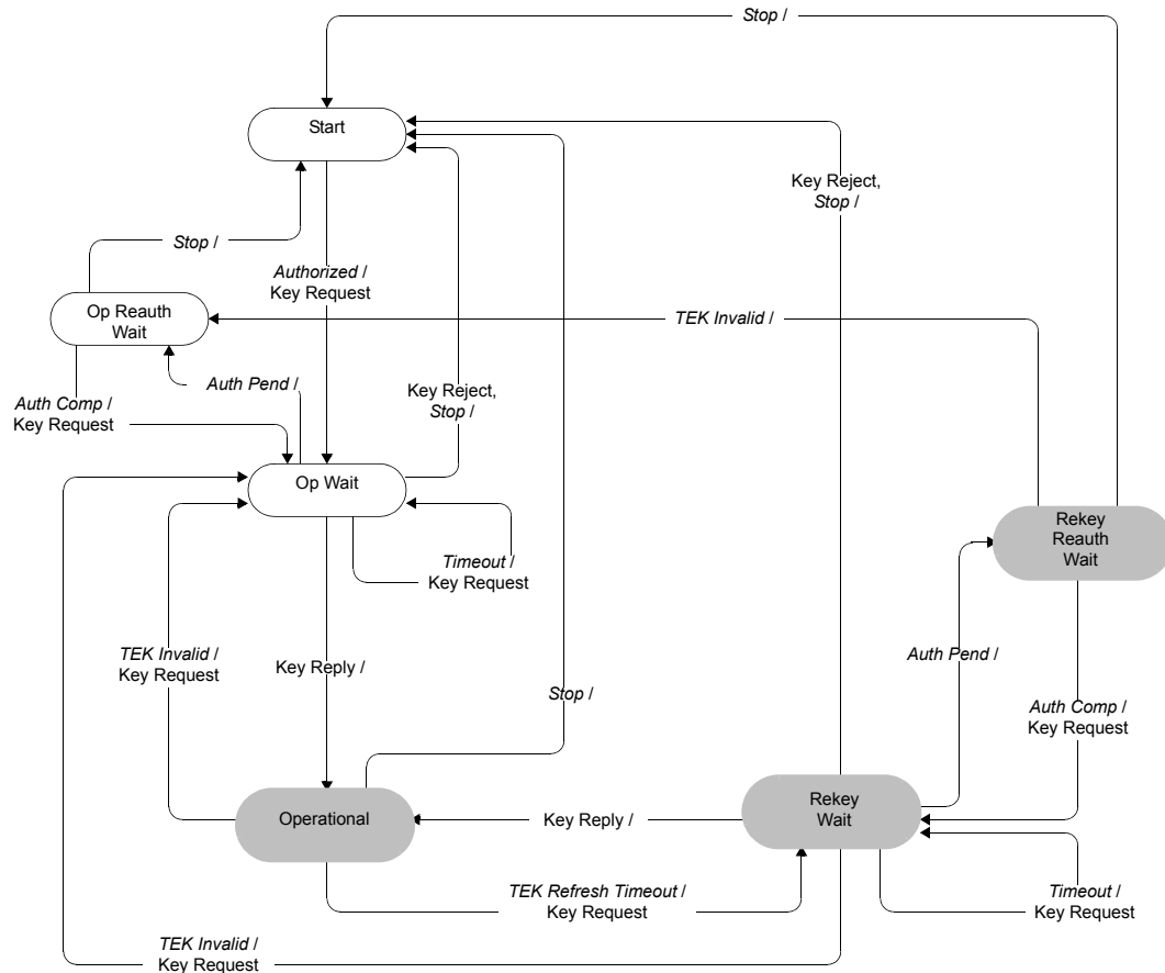
Figure 158—TEK state machine flow diagram
