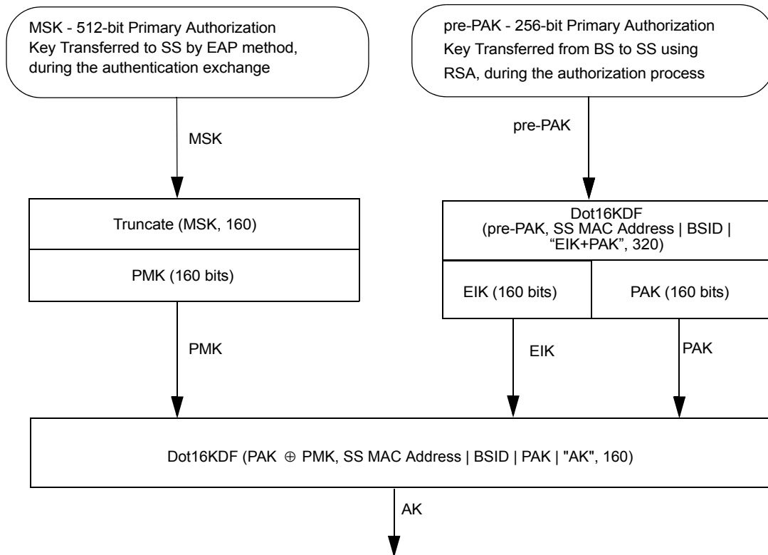
Figure 160—AK from PAK and PMK (RSA-based and EAP-based authorization)
