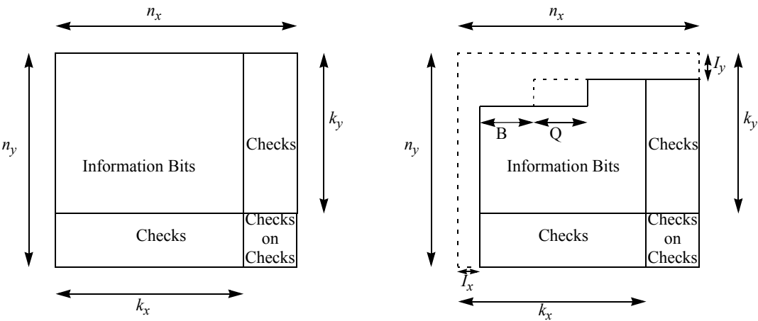
Figure 288—BTC and shortened BTC structure
