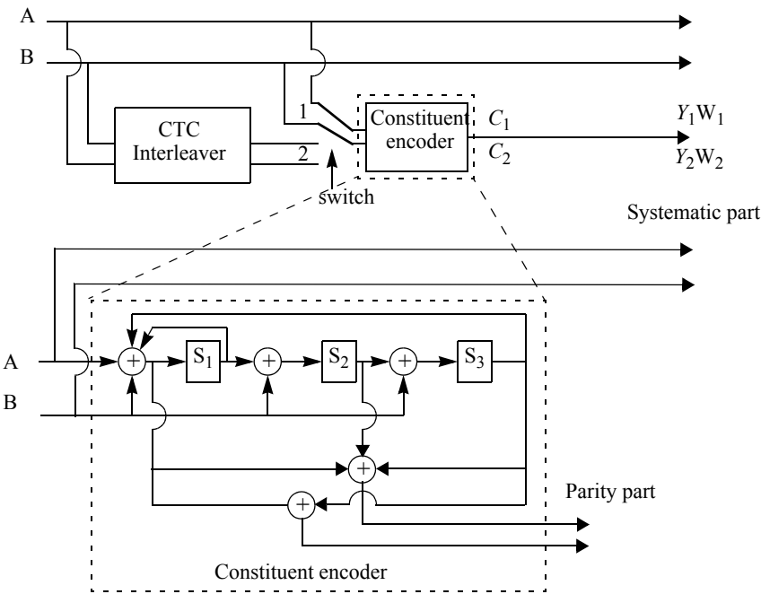
Figure 289—CTC encoder
