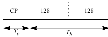
Figure 208— P_{\text{EVEN}} time domain structure
