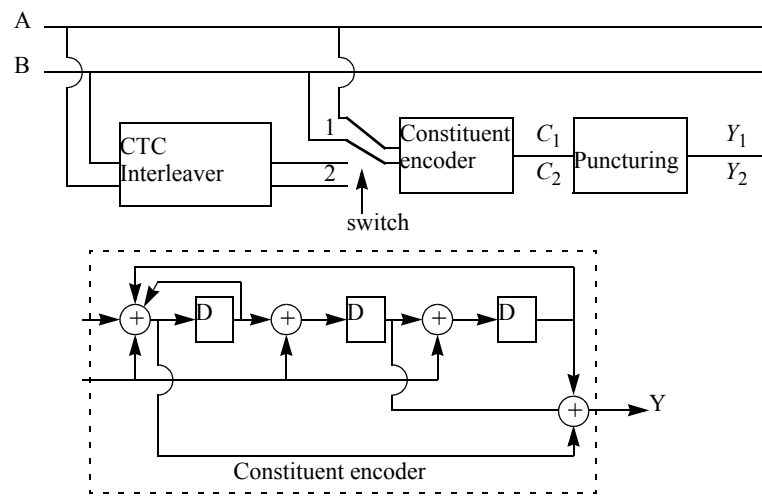
Figure 204—CTC encoder
