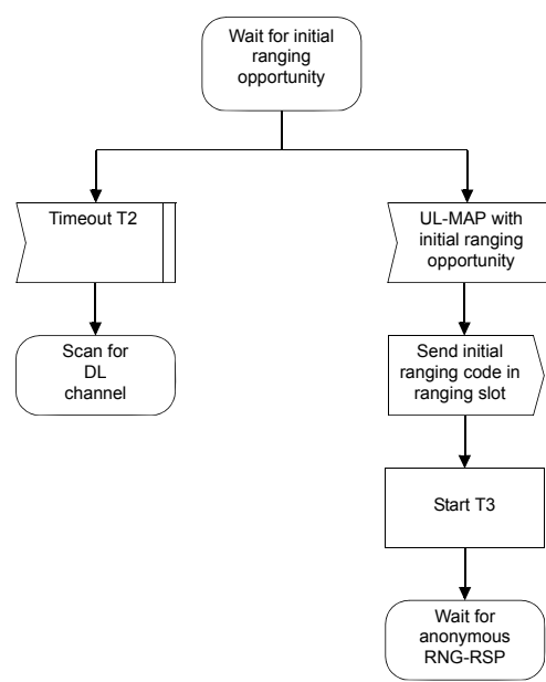
Figure 93—CDMA initial ranging—SS (part 1)
