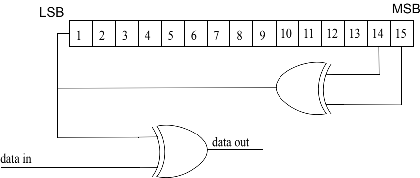
Figure 285—PRBS generator for data randomization
