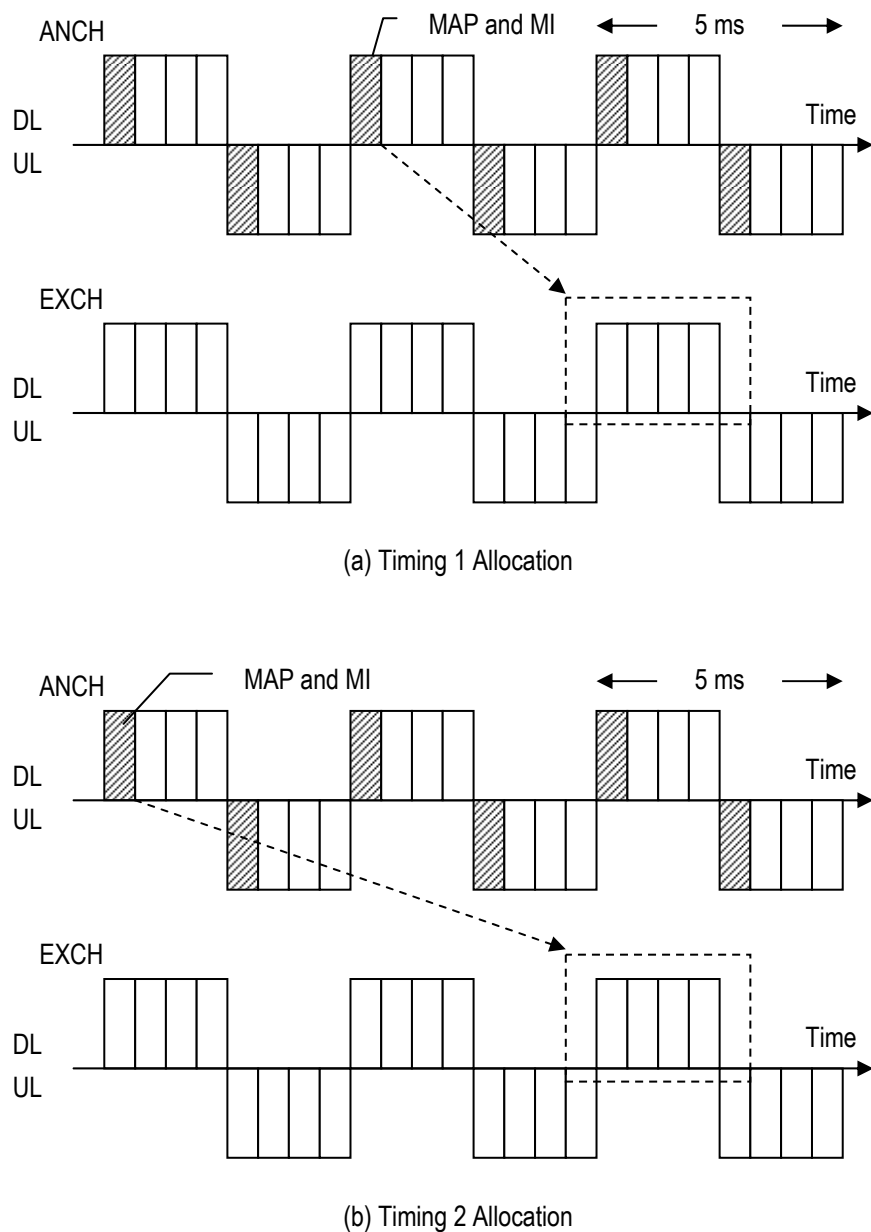
Figure 4.35 Example of DL MI Indication Timing in ECCH on 5 ms frame
