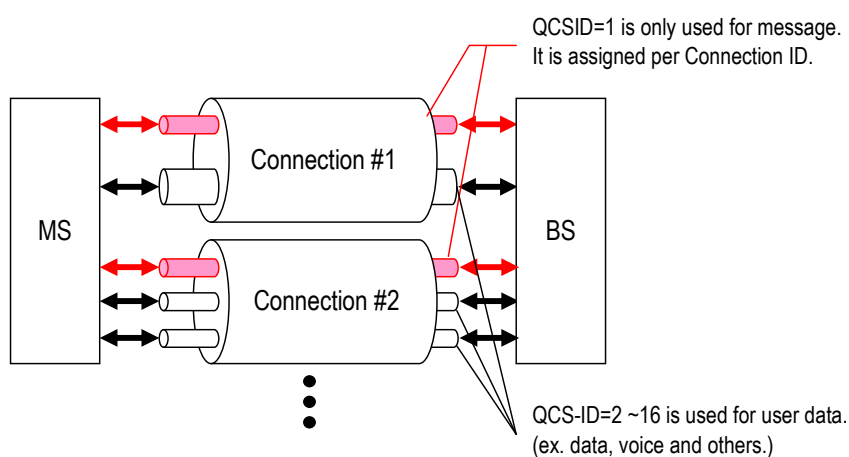
Figure 9.21 Connection and QCS
