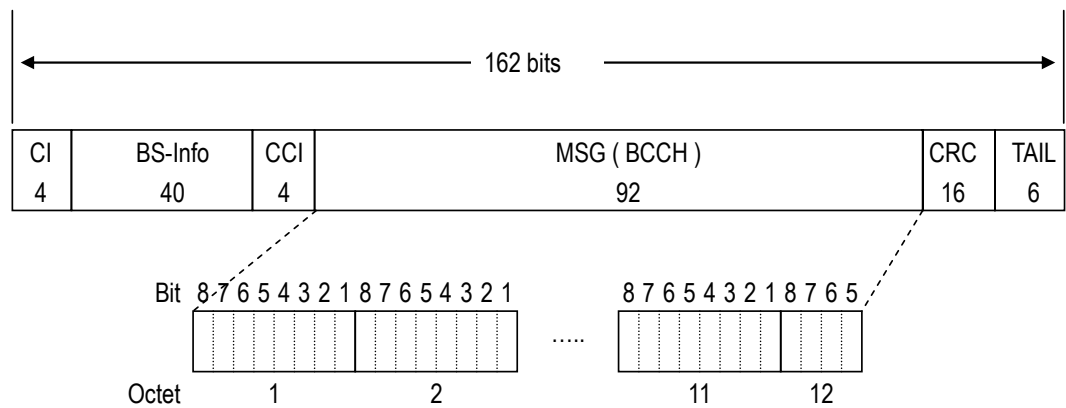
Figure 5.10 BCCH Format
