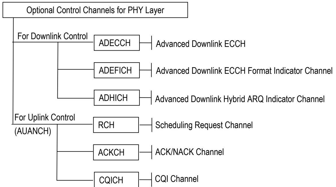
Figure 4.10 Composition of Optional Control Channels
