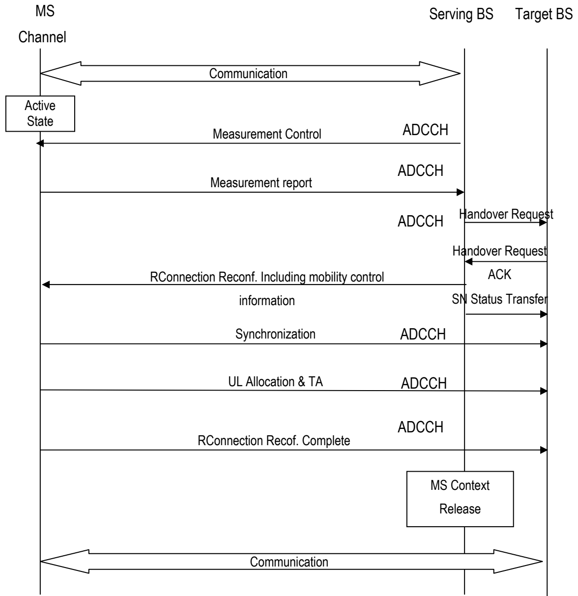
Figure 8.34 BS HO
