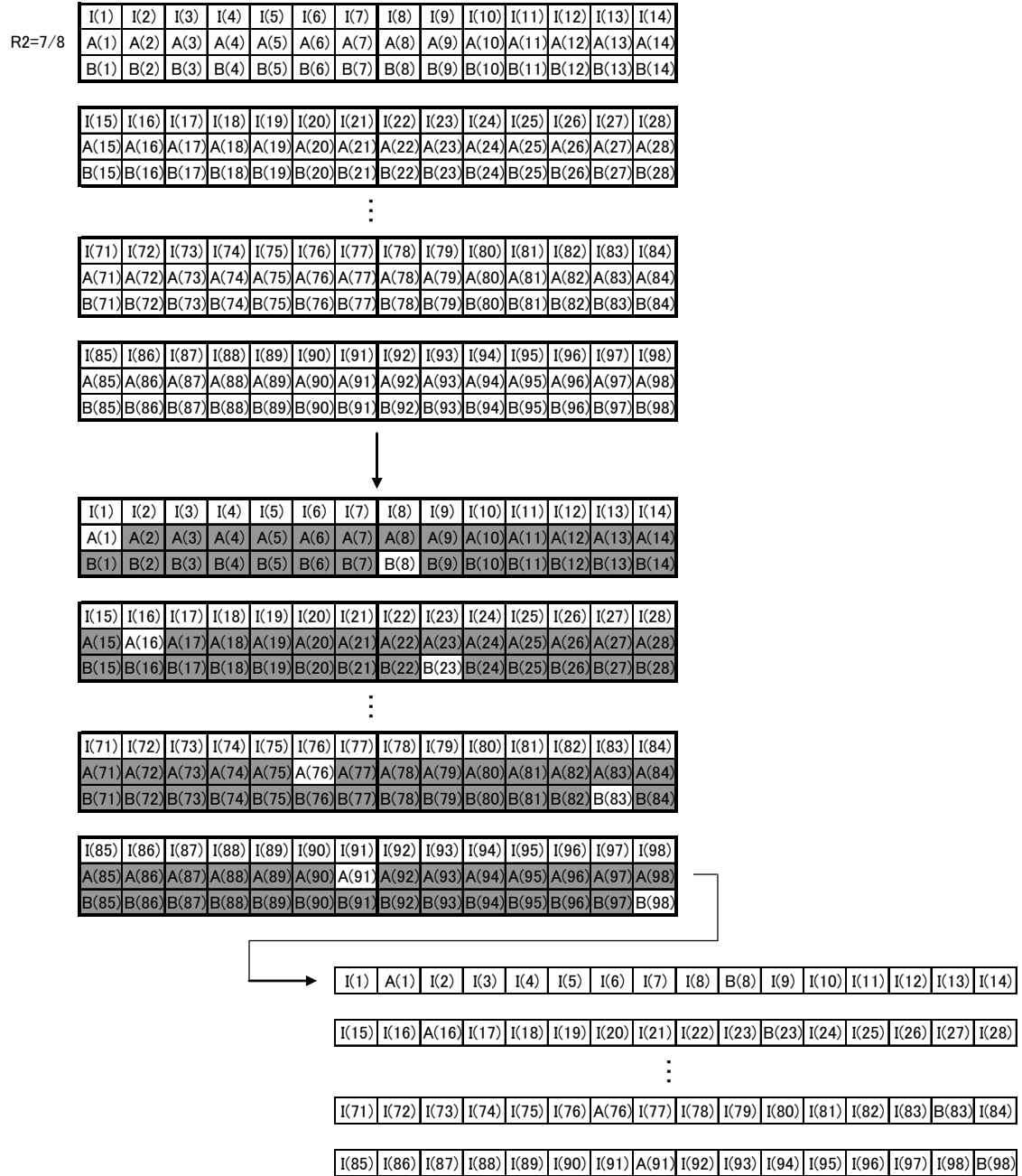
Figure 3.27 Puncturing Procedure while R2 is 7/8
