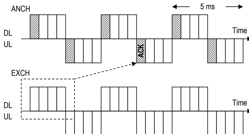
Figure 4.41 UL ACK Response Timing
