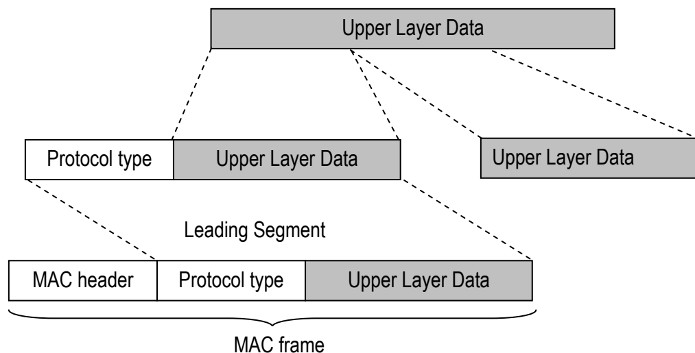
Figure 4.81 Relation between MAC Frame and Upper Layer Data with Protocol Type
