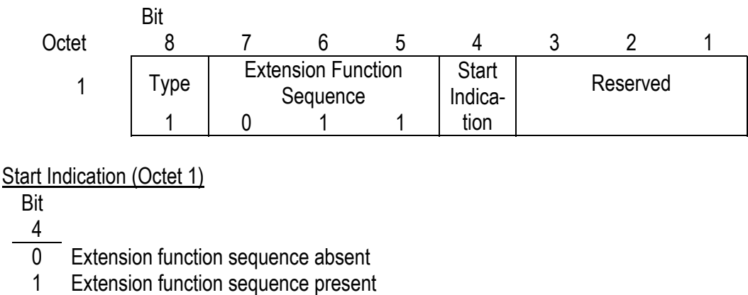
Figure 7.6 Extension Function Sequence
