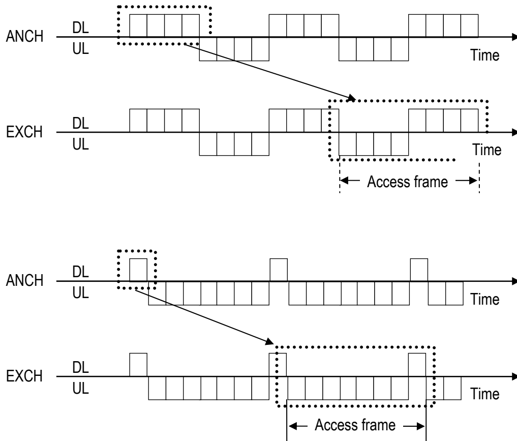
Figure 6.8 Timing 2 for 5ms frame
