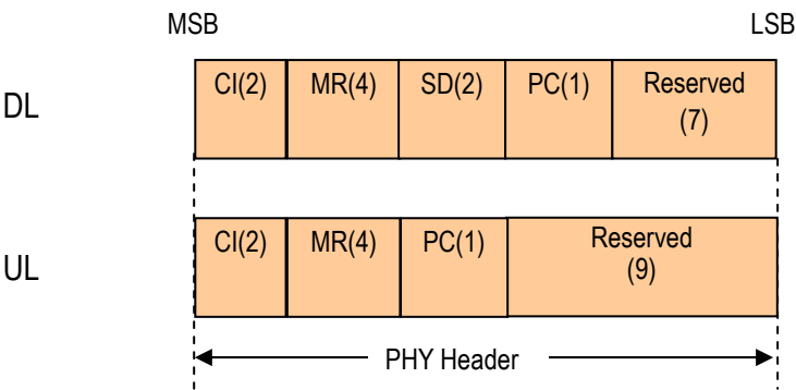
Figure 4.30 PHY Header Structure of CSCH/TCH
