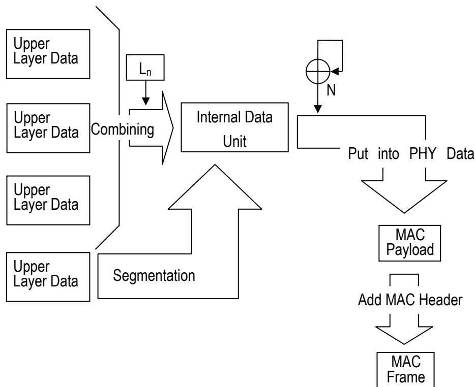
Figure 4.68 Procedure to Construct MAC Frame
