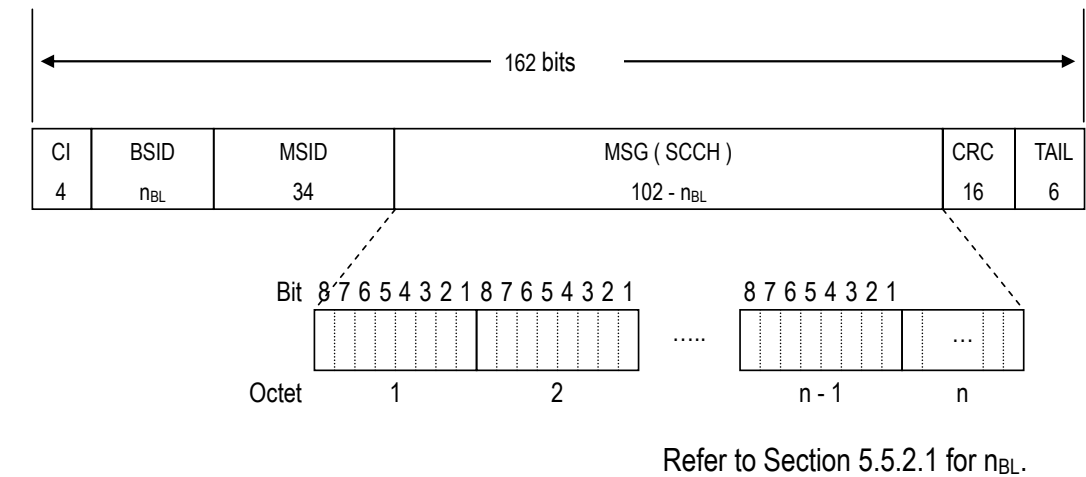
Figure 5.13 UL SCCH Format for OFDMA
