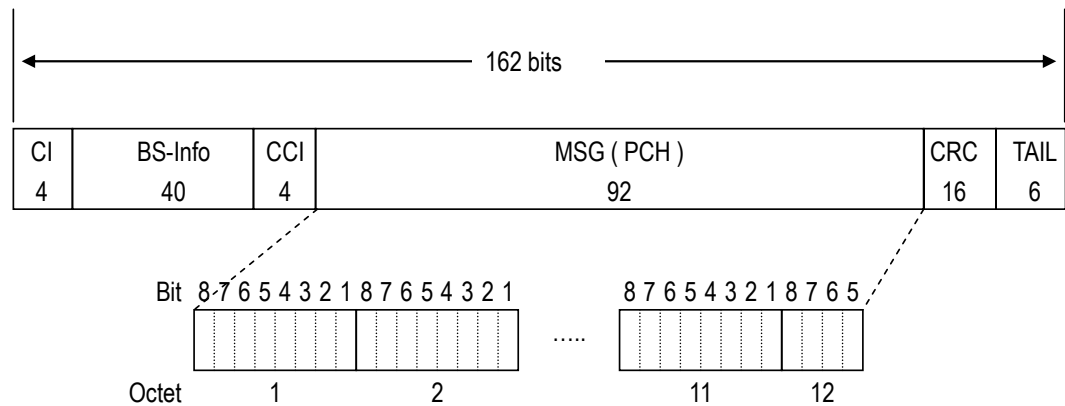
Figure 5.11 PCH Format
