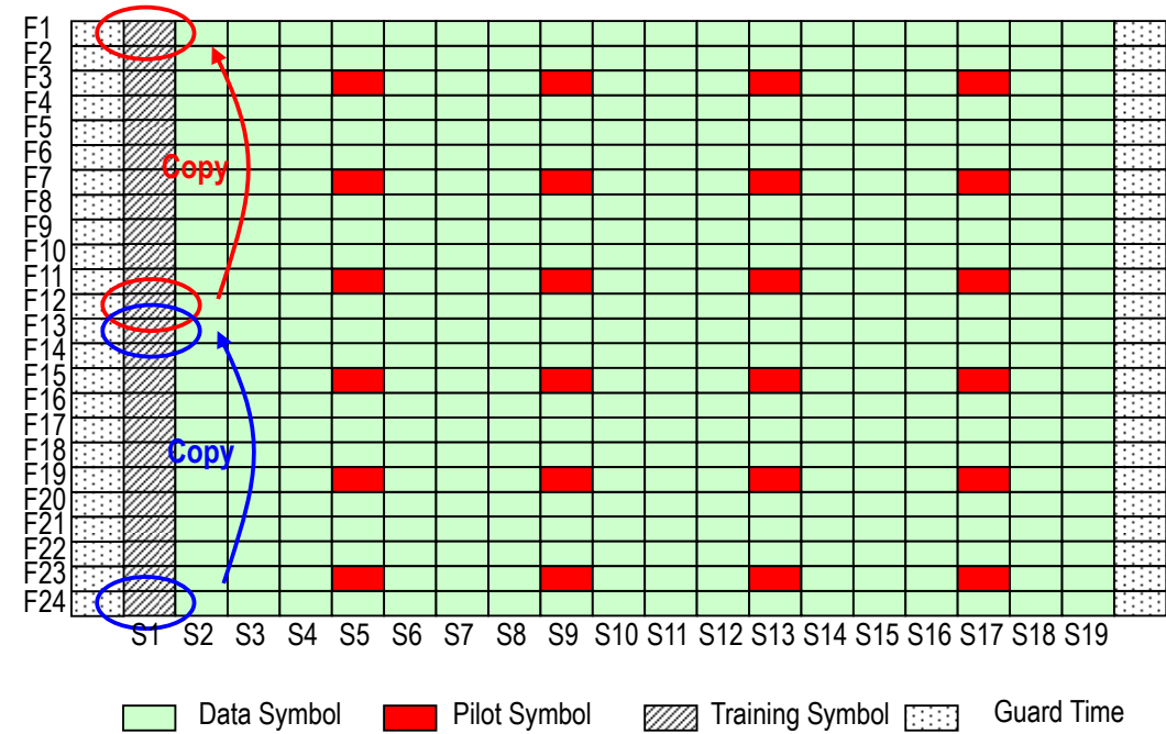
Figure 3.75 OFDM PRU Structure for EXCH format (b)
