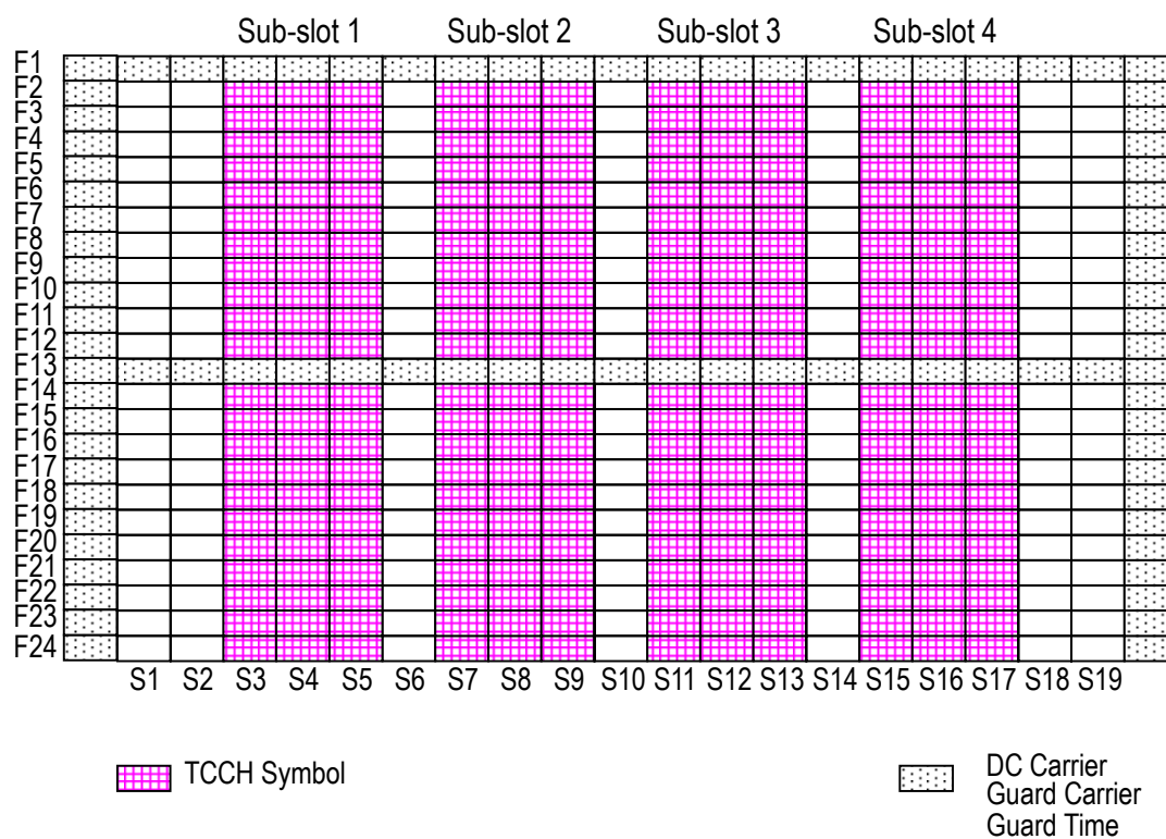
Figure 3.82 OFDM PRU Structure for TCCH
