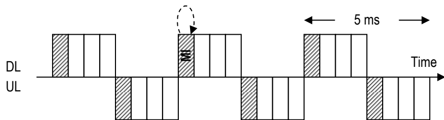
Figure 4.37 DL MI Indication Timing in CSCH
