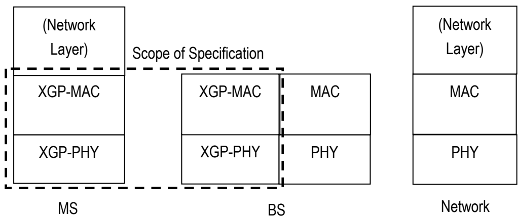
Figure 4.6 Protocol Stack for XGP
