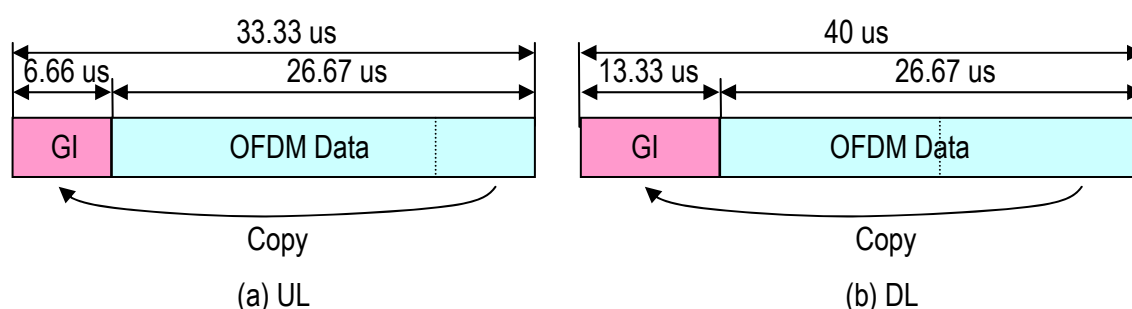
Figure 3.2 Guard Interval (S1)
