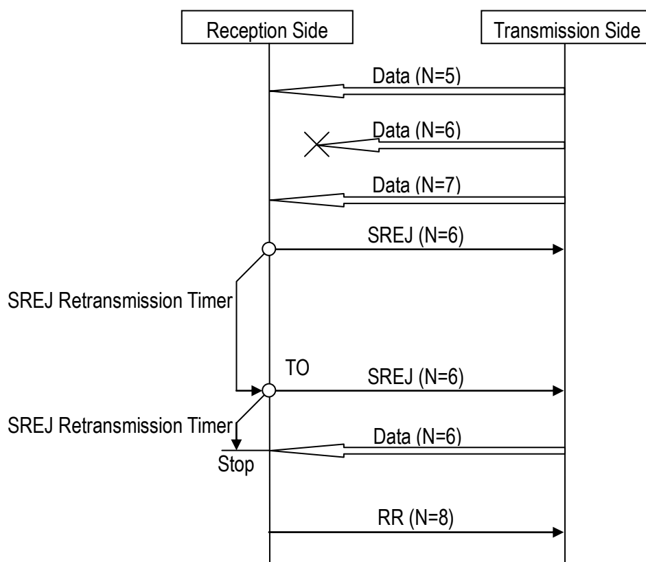
Figure 9.43 ARQ Succession
