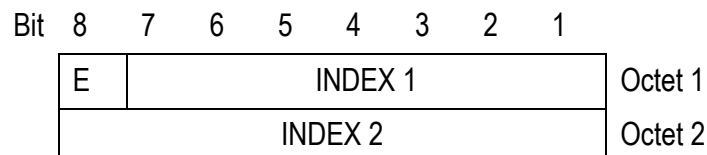
Figure 4.79 Format of Index Field
