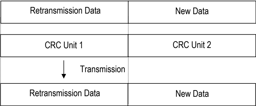
Figure 3.104 The case when Retransmission CRC Unit Size equals to available CRC Unit Size
