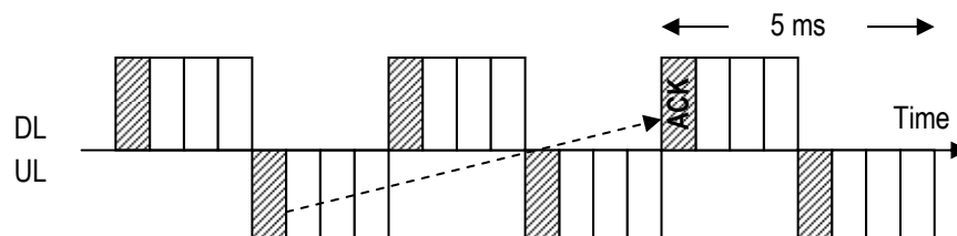
Figure 4.42 DL ACK Response Timing
