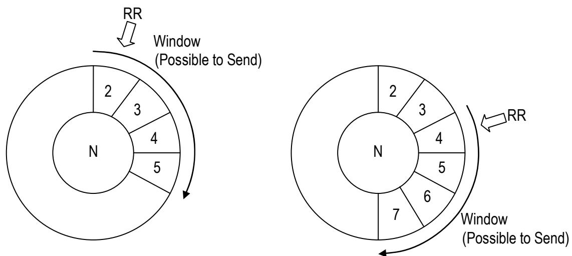
Figure 9.37 Window Control
