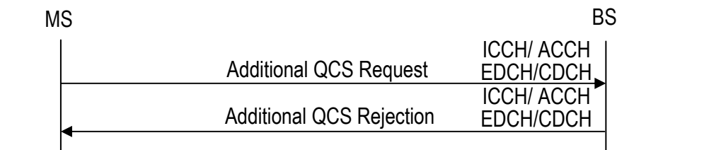
Figure 8.22 Additional QCS Sequence
