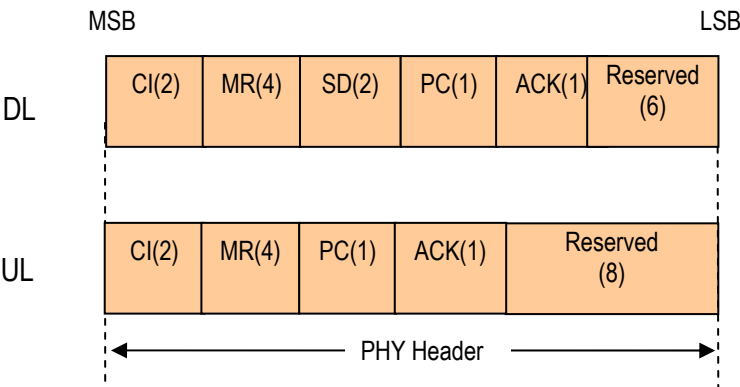
Figure 4.29 PHY Header Structure of CSCH/CDCH
