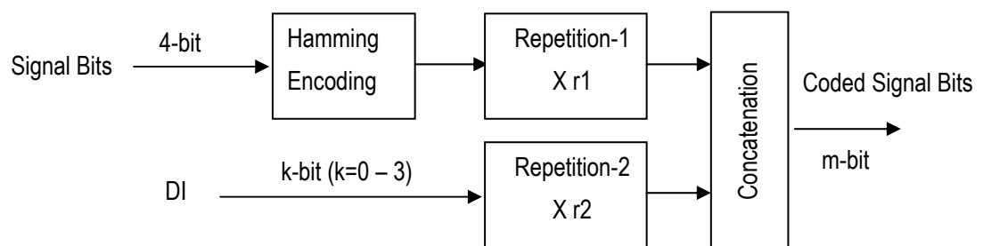
Figure 3.111 Signal Encoding for SC
