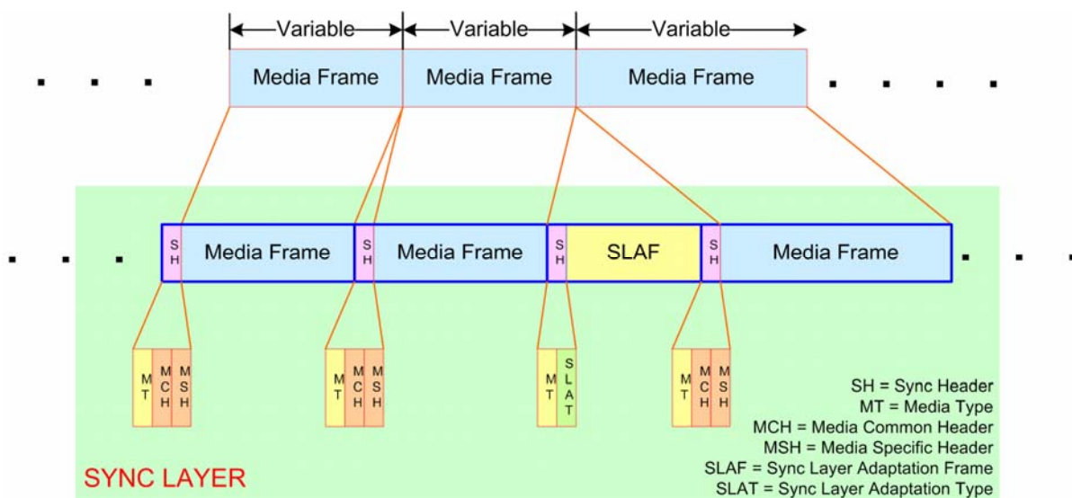
31 Figure 5: Relationship between Media Frames and Sync Layer Packets
