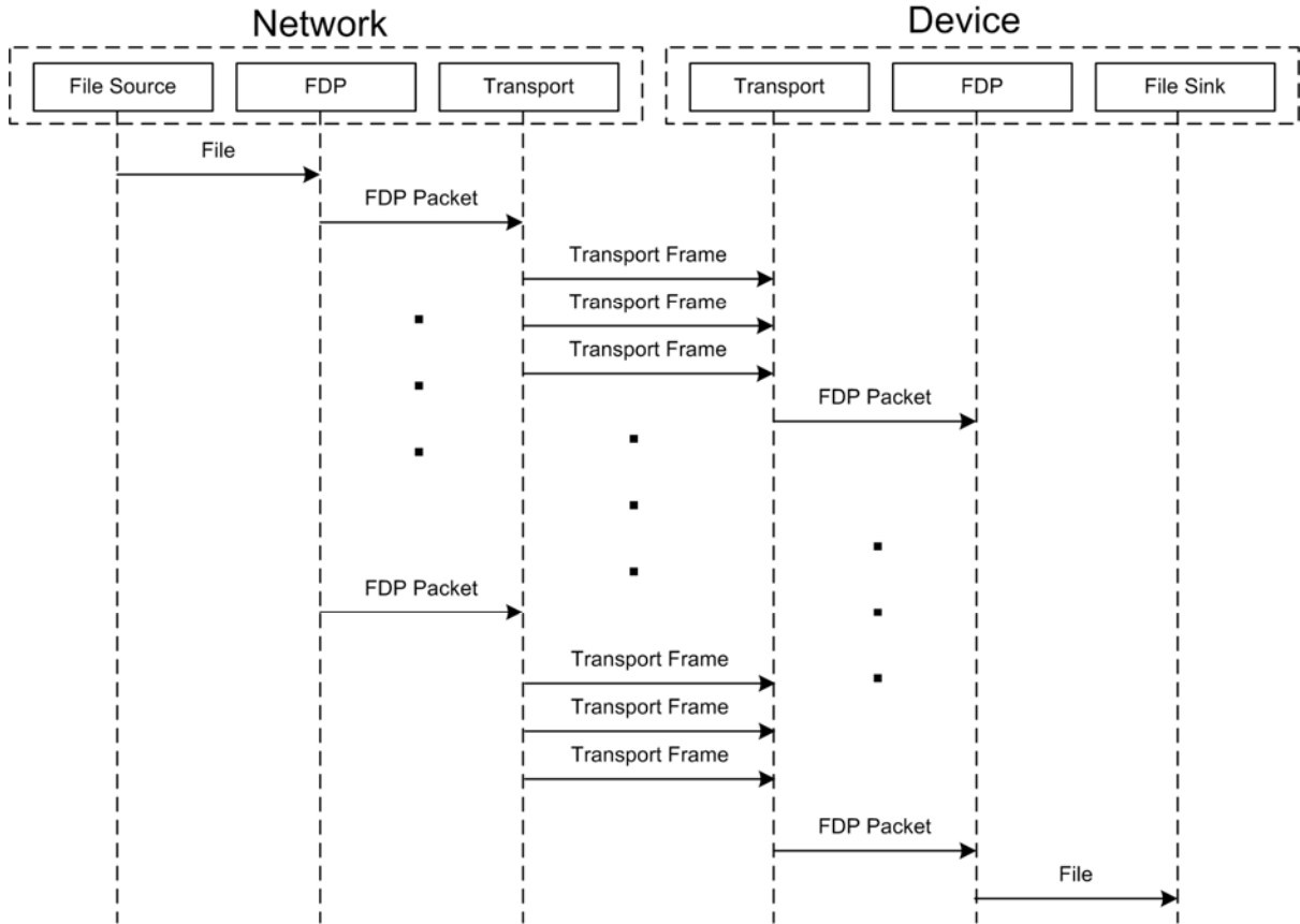
Figure 9: File Delivery Message Flow
