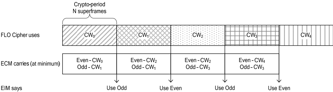
8 Figure 9: Even/odd scrambler-descrambler synchronization mechanism.
