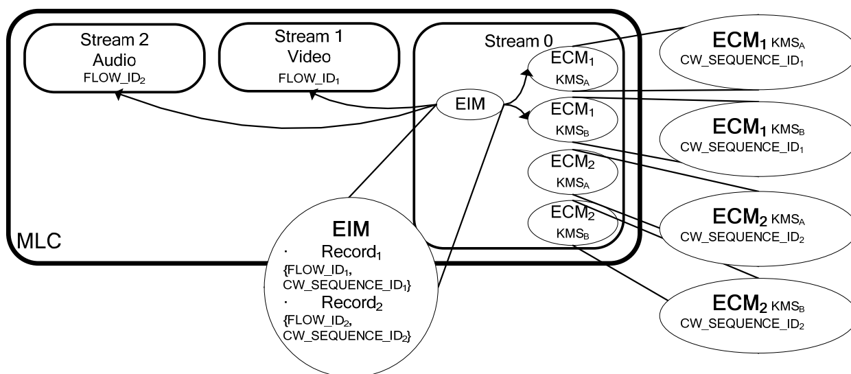
7 Figure 4: Example of a MLC with one audio and one video scrambled with different CWs 8 (multiple KMS case).
