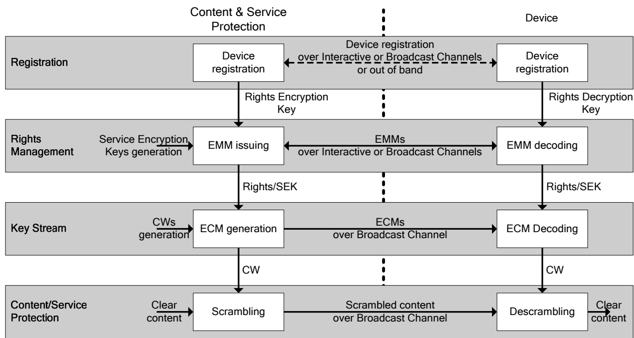
Figure 8: Hierarchical Model for Content & Service Protection.
