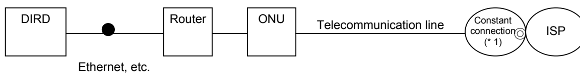
Fig. 9.5.2 Router connection
