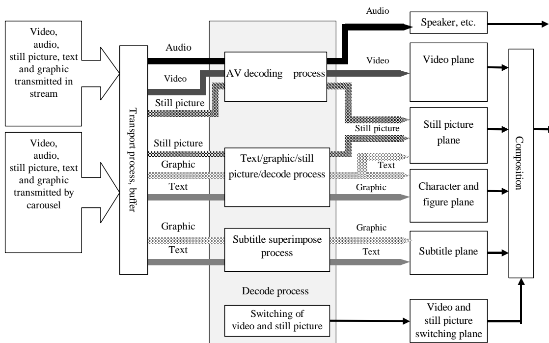
Figure 6-2 Model decoder in receiver showed with data processing flow
