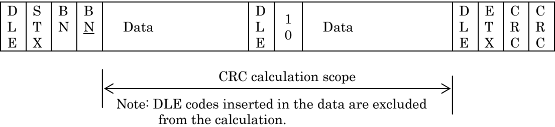
Figure 4-41 CRC Calculation Scope
