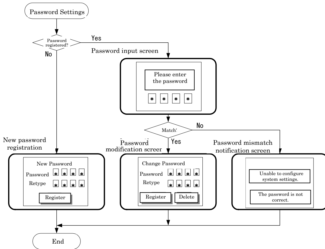
Figure 4-10 Password Setting Flow
