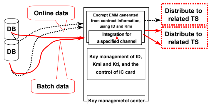
Figure A3-1. Key management center (Common and secret keys)
