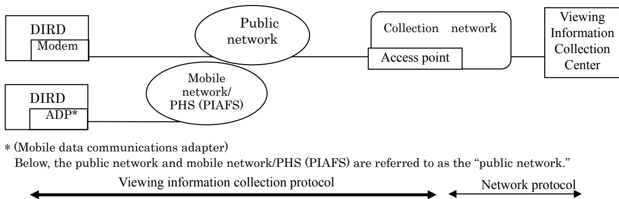
Figure 4-29 Viewing Information Collection System
