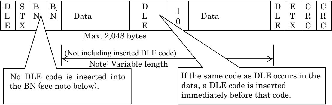
Figure 4-40 Text Transmission Format
