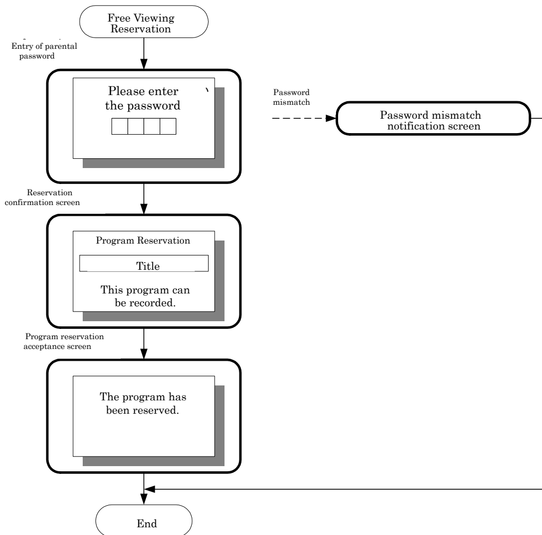
Figure 4-7 Free Viewing Reservation Processing Flow
