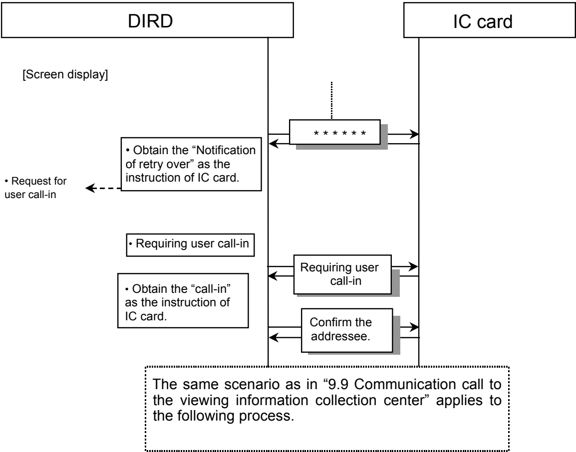
Figure A1-21. User call-in
