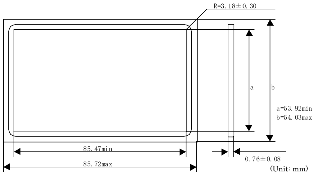
Figure 4-15 IC Card Dimensions
