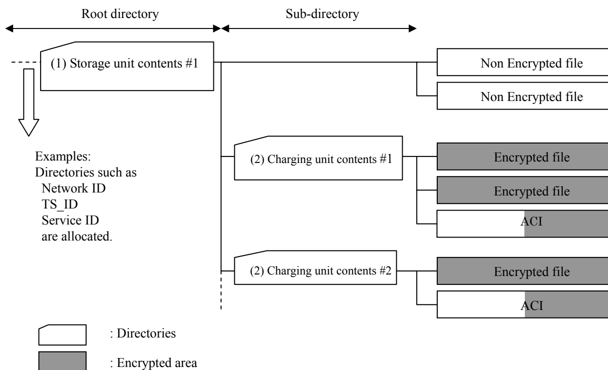
Figure A1-9 Example of Storage Administration Model
