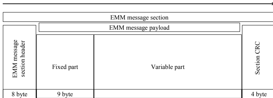
Figure 2-7 EMM Common Message Section Architecture
