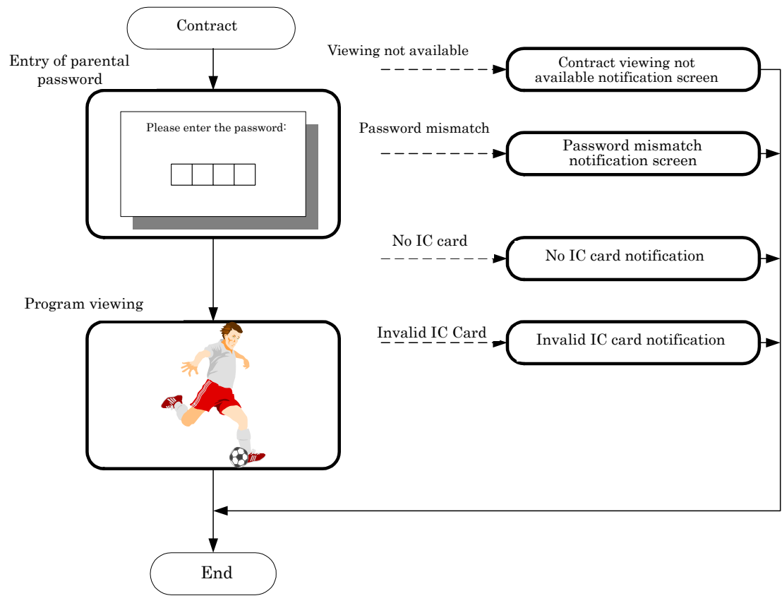
Figure 4-4 Contract Viewing Processing Flow
