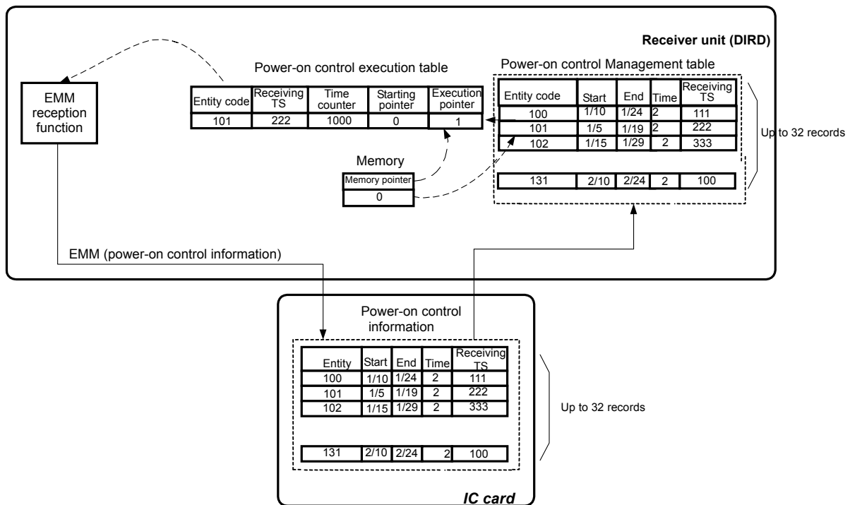
Figure A2-7. Example of the schedule management for power-on control
