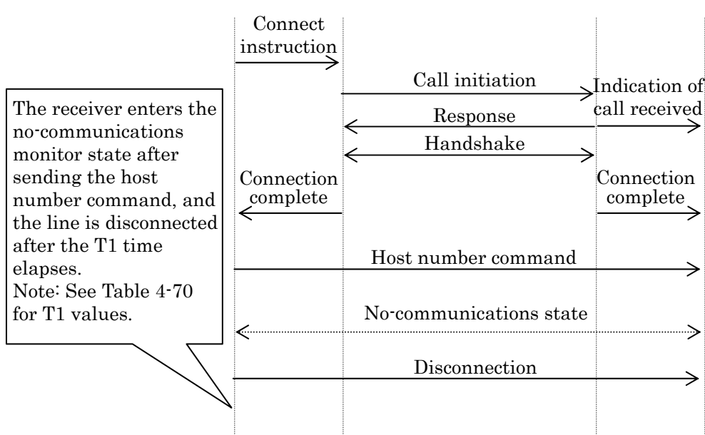
Figure 4-35 Error Sequence (DIRD Timeout While Waiting for Remote Echo)
