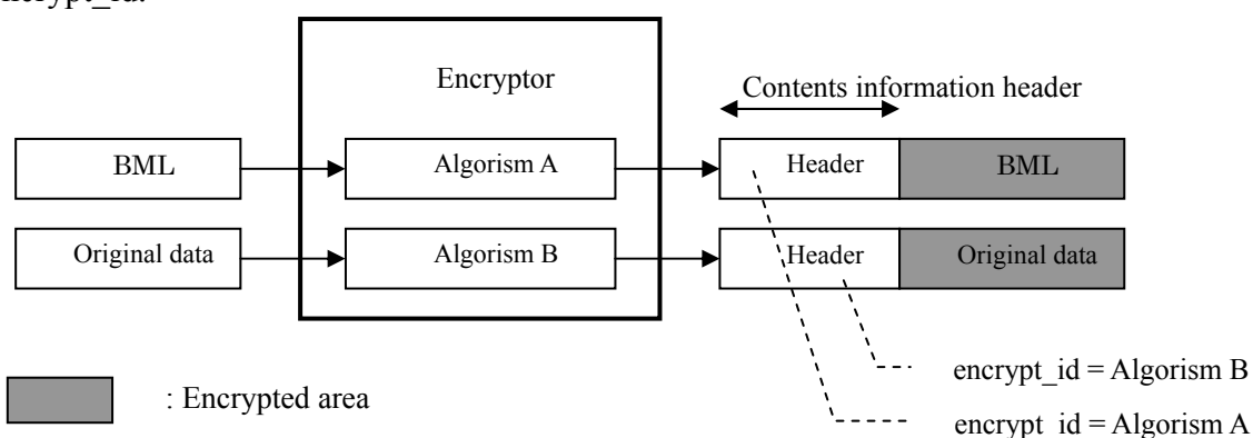
Figure A1-8 Identification of Encryption Method
