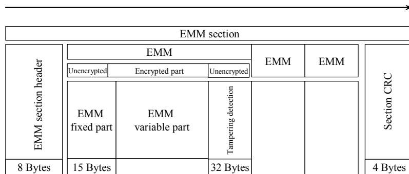
Figure 2-6 EMM Section Architecture
