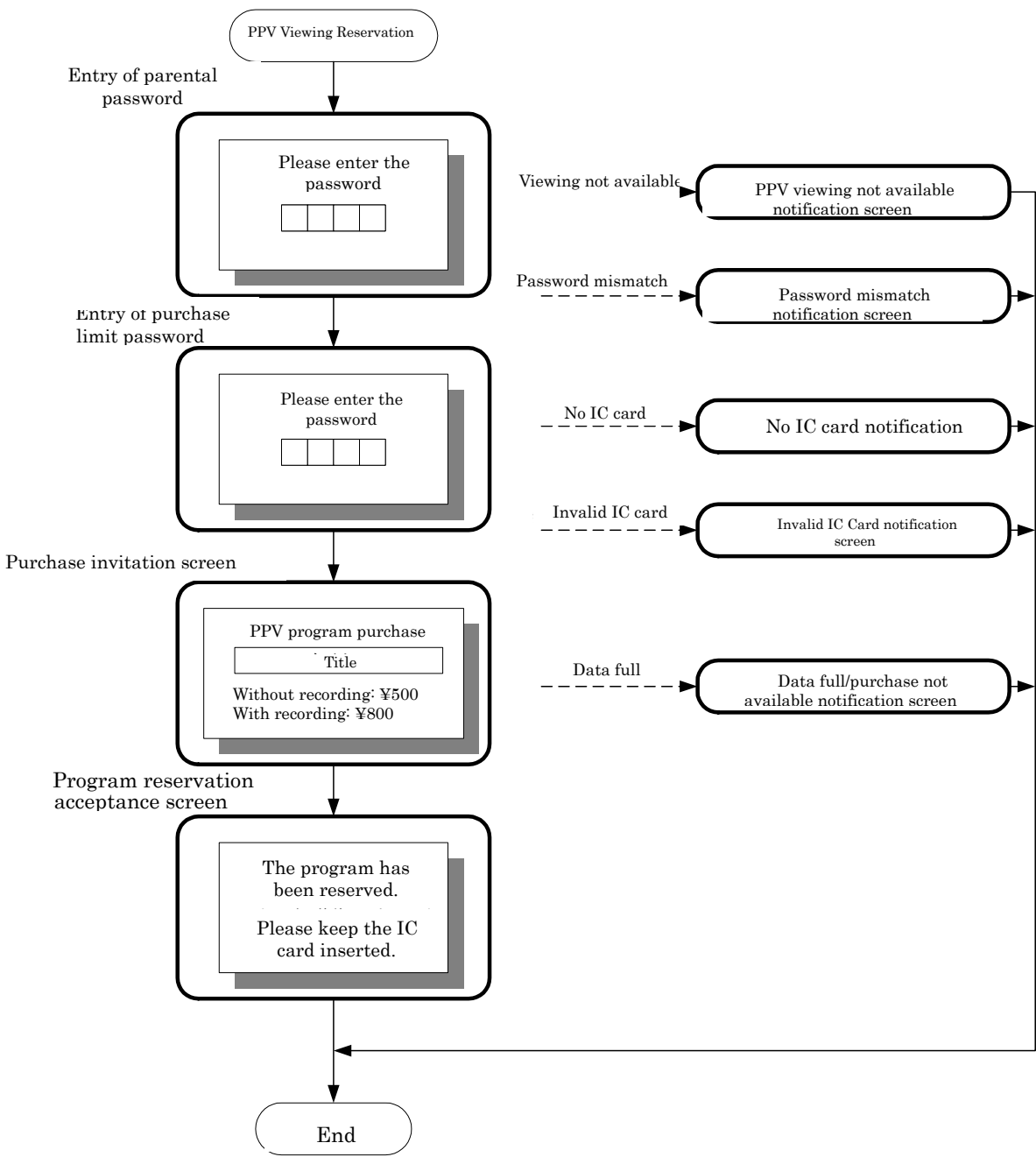
Figure 4-9 PPV Viewing Reservation Processing Flow
