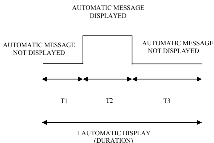
Figure 2-8 Automatic Display Duration and the direction of displaying the message
