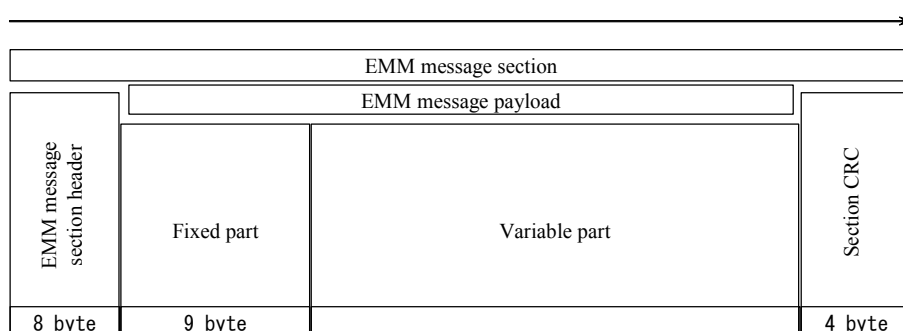
Figure 3-6 EMM Shared Message Section Architecture
