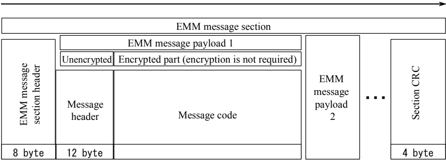
Figure 3-8 EMM Individual Message Section Architecture
