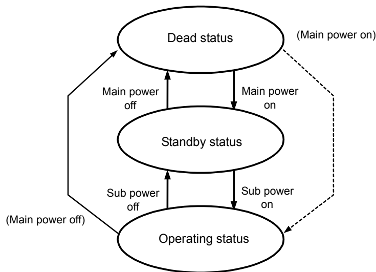
Figure A2-2. Statuses of the receiver unit
