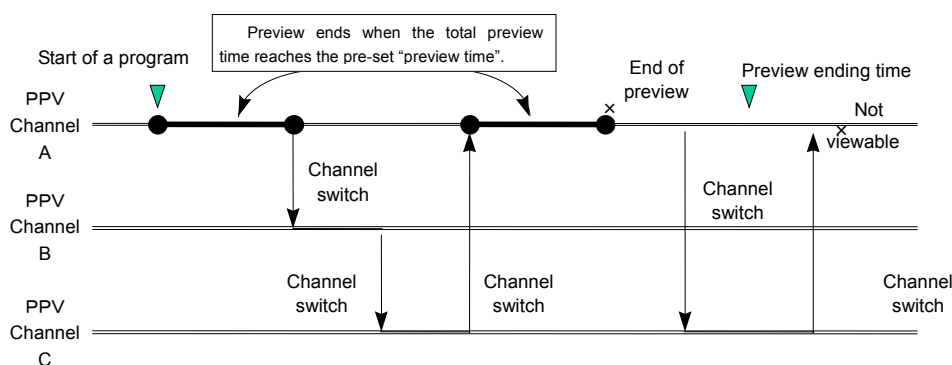
Figure A1-5. Example of preview patterns
