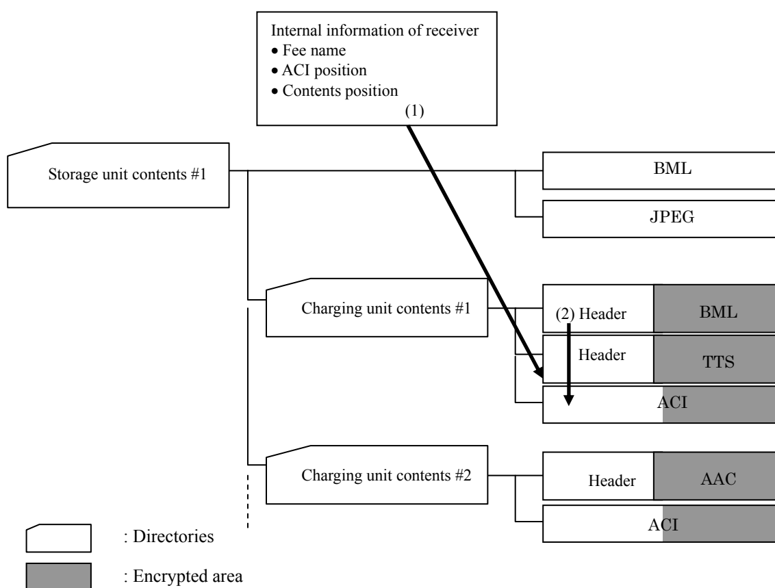
Figure A1-10 ACI Reference Method
