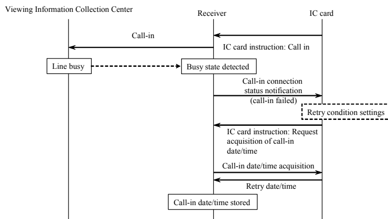
Figure 4-47 Failed Call-in Processing Flow
