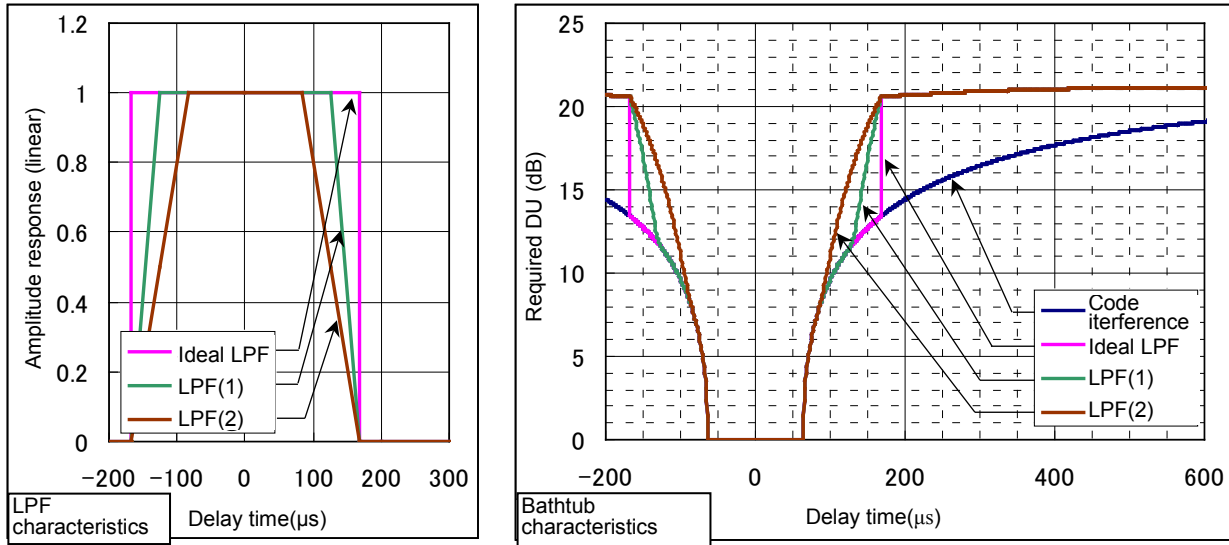
Figure A-24 Interpolation LPF characteristic and required DU characteristic(For 64QAM-3/4, N_{amp}=-35\text{dB} in expression (25))
