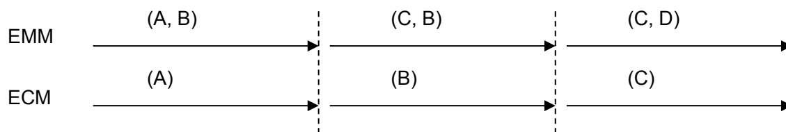
Figure 4-10 Example of an operation flow to update a work key for disabling a specific work key
