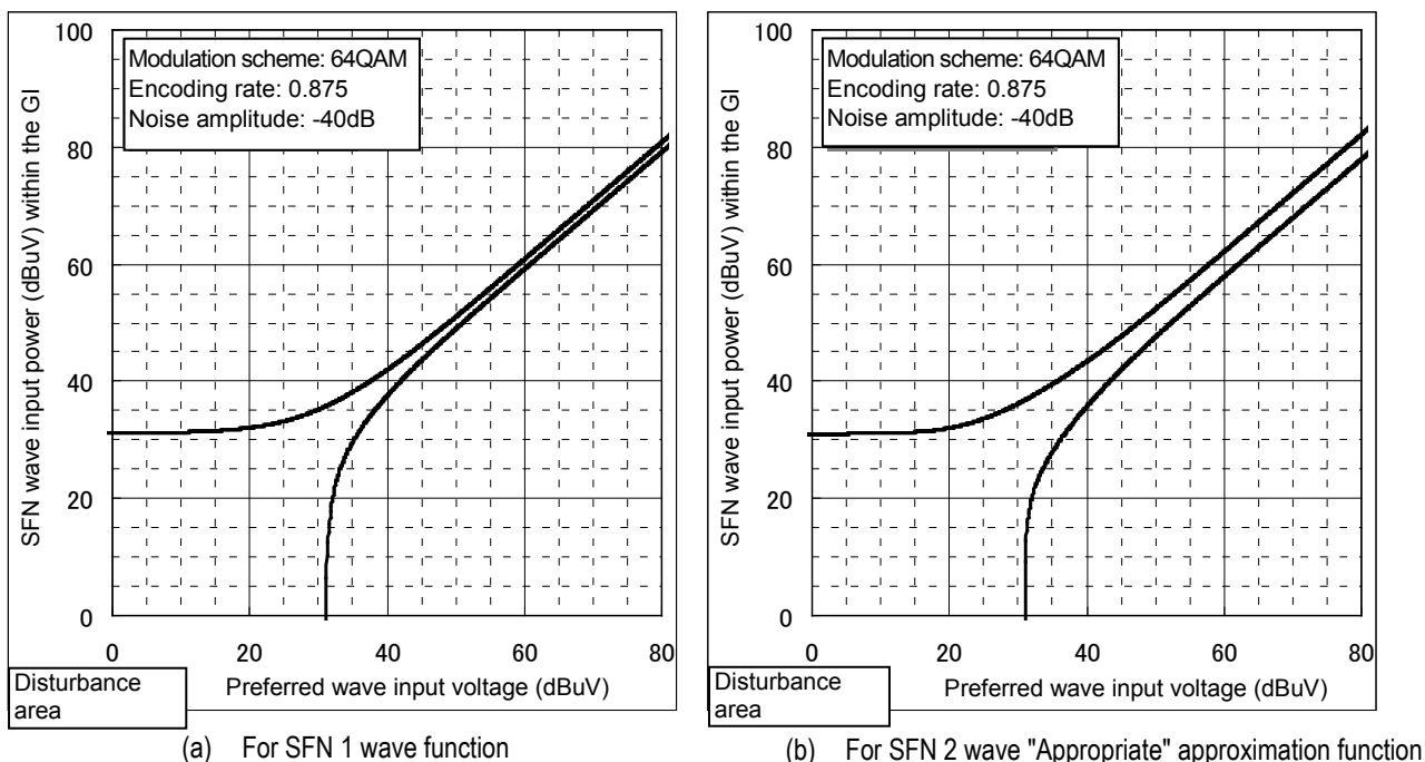
Figure A-15(2/2) Comparison of SFN reception disturbance areas for 64QAM-7/8
