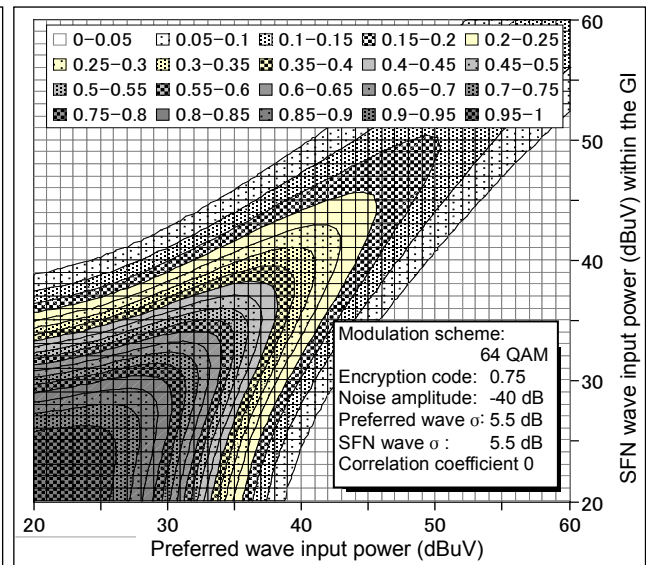
Figure A-8 SFN reception disturbance generation probability example(64QAM-7/8)
