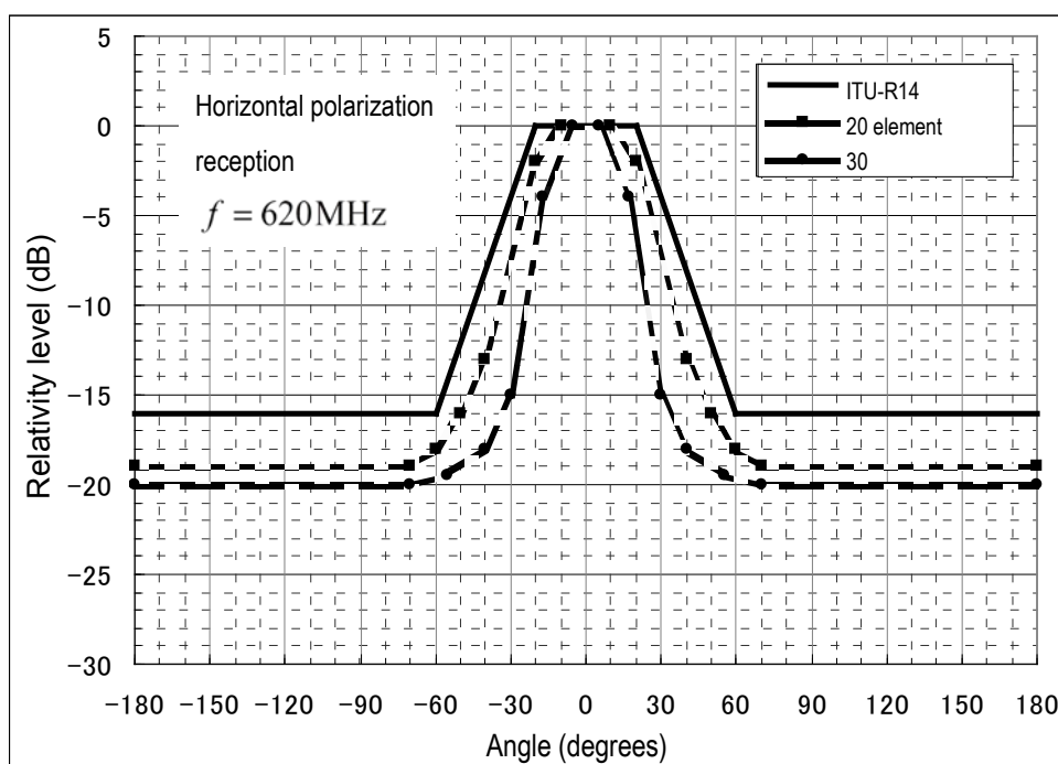
Reference figure 1 Model characteristic of reception antennas (Horizontal direction characteristics)
