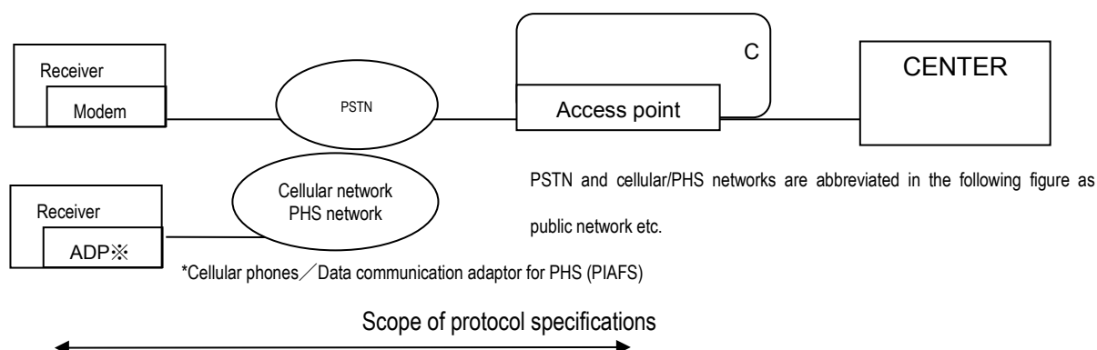
Figure 5-2 Bi-directional data broadcasting service system
