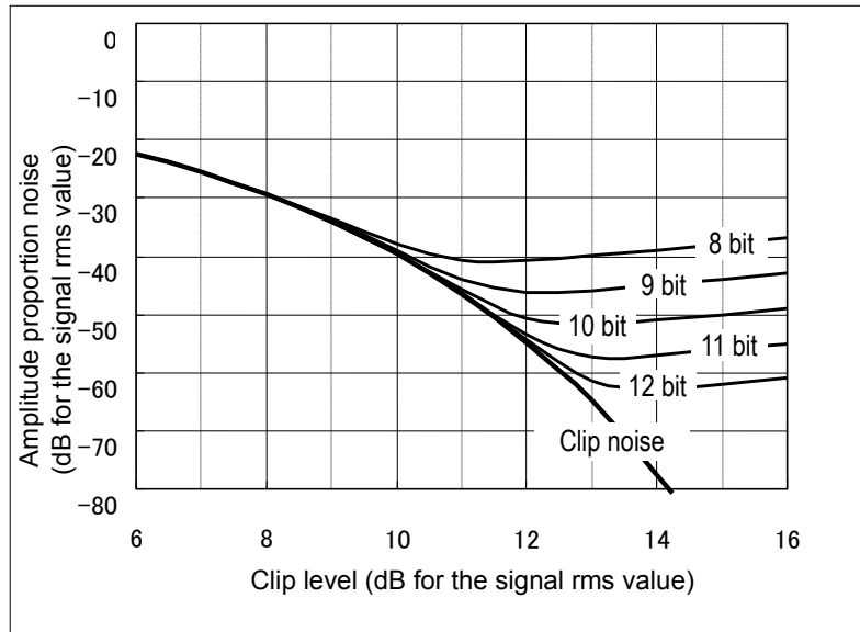
Figure A-4 Amplitude proportion noise example
