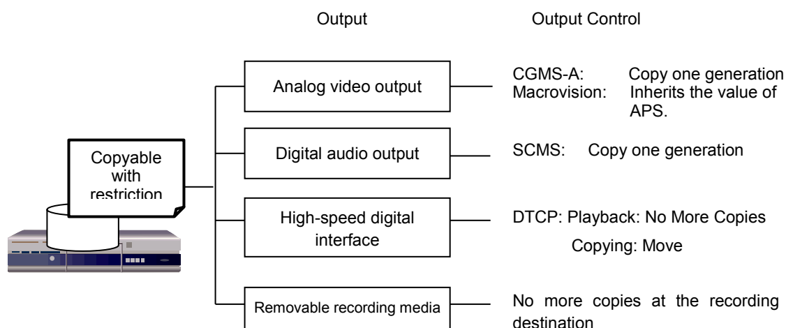
Figure 7-2 Output destinations and control of content recorded with "copyable with restriction"
