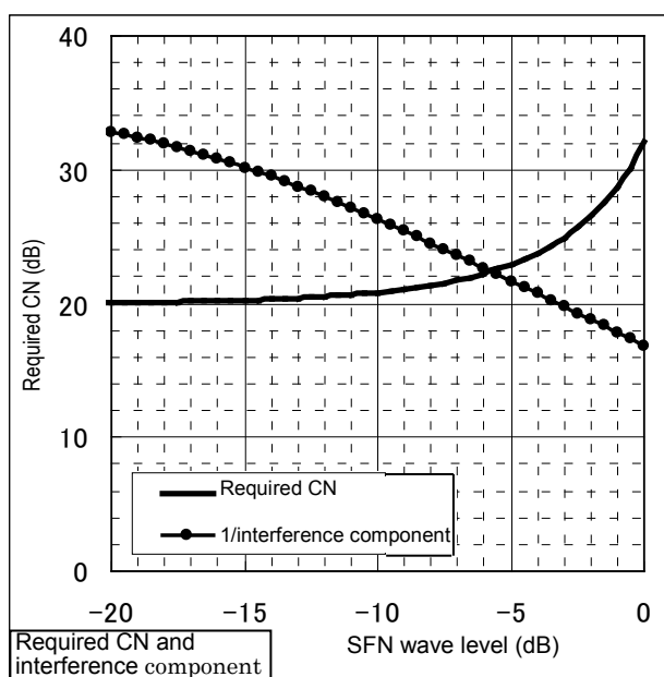
Figure A-19 Required CN of SFN wave exceeding GI and Interference component
