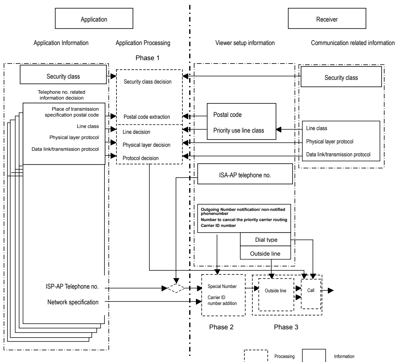
Figure 7-5 Call processing details
