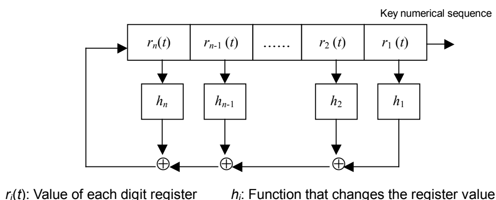
Appended figure 1-2 Simple encryption device using the linear feedback register
