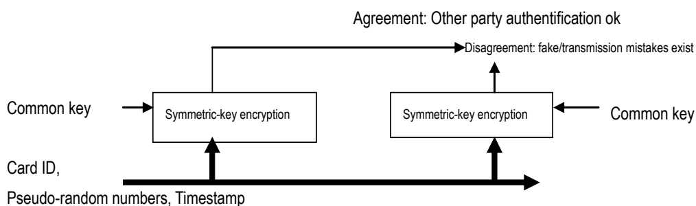
Figure 8-1 Other party authentication using the message restoration method
