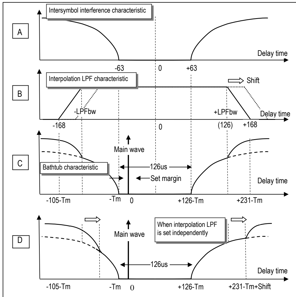
Figure 4-2 Assumed bathtub characteristic(For GI = 126 \mu s )
