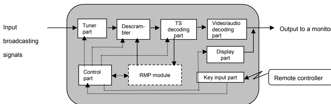
Figure 5-1 Basic receiver structure
