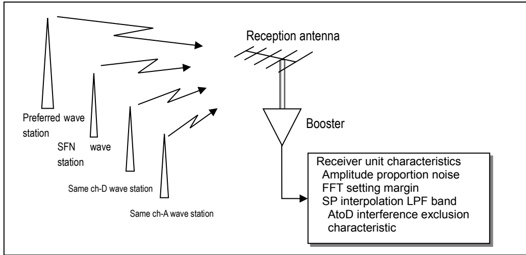
Figure 4-1 Reception system model in the design of transmission stations
