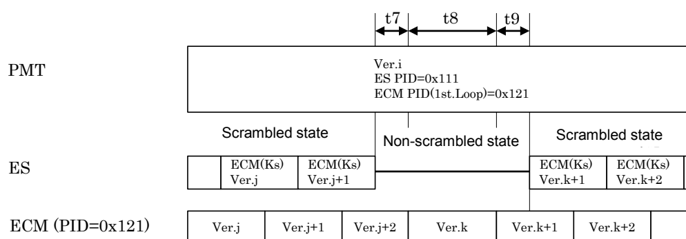
Figure 4-6 Updating a work key
