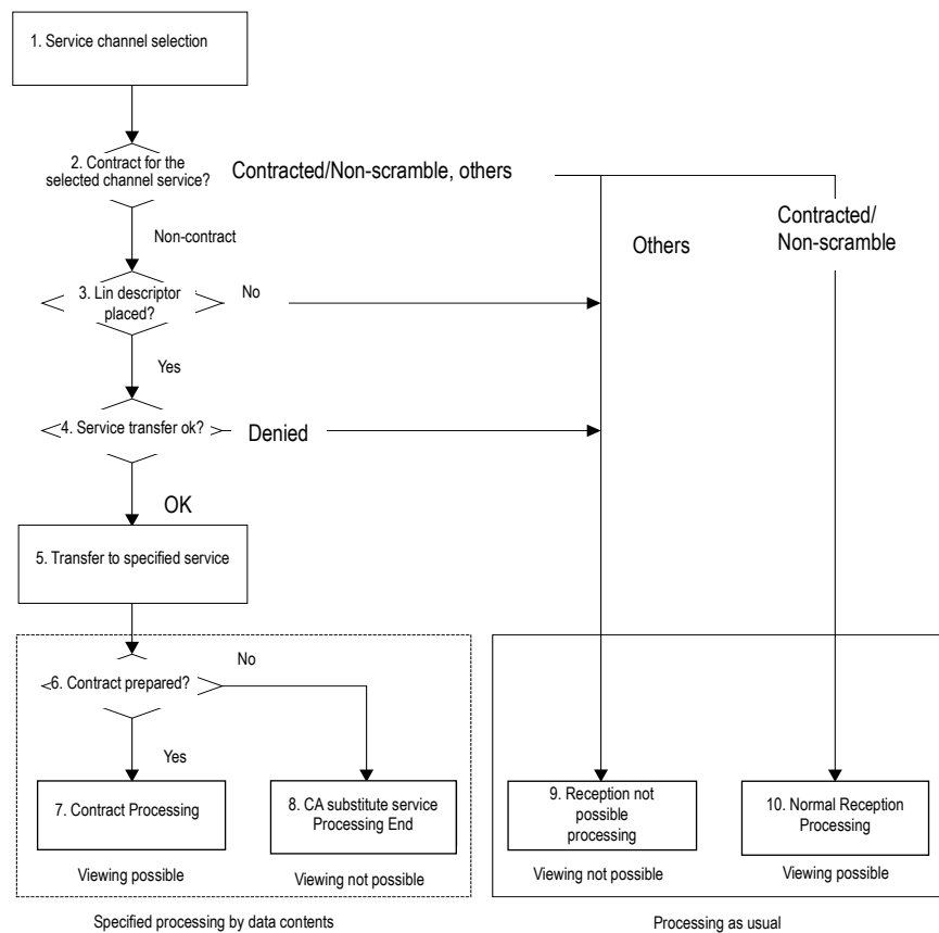
Figure 5-2 CA substitute service processing flow example
