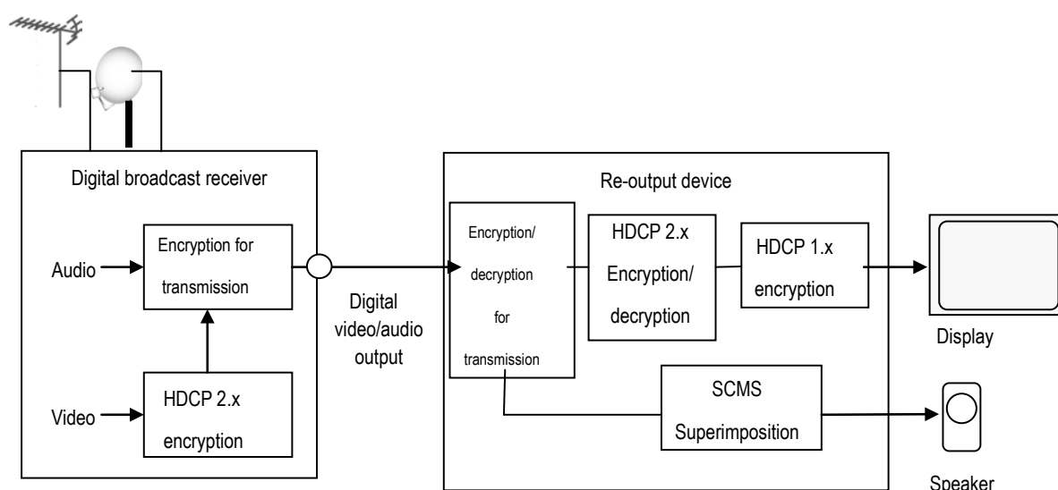
Figure 7-3 Example of digital video/audio output assumed in 7.12
