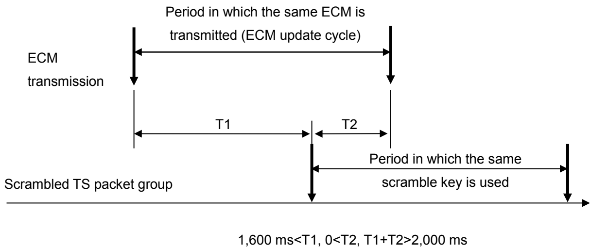
Figure 4-7 Updating an ECM and changing a scramble key
