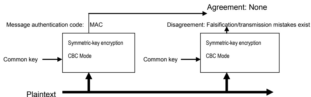
Appended figure 1-3 Data integrity using the message authentication code
