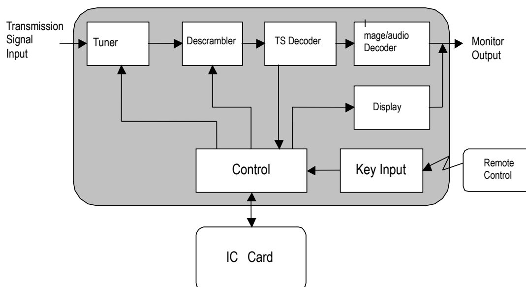
Figure 5.1 Basic configuration of receiver units
