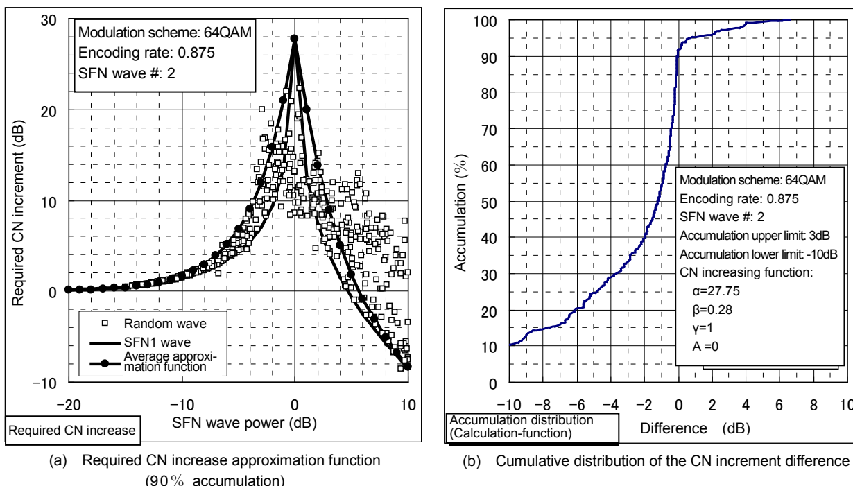
FigureA-15(1/2) "Appropriate" approximation function for 64QAM-7/8 ( \gamma=1 type function)
