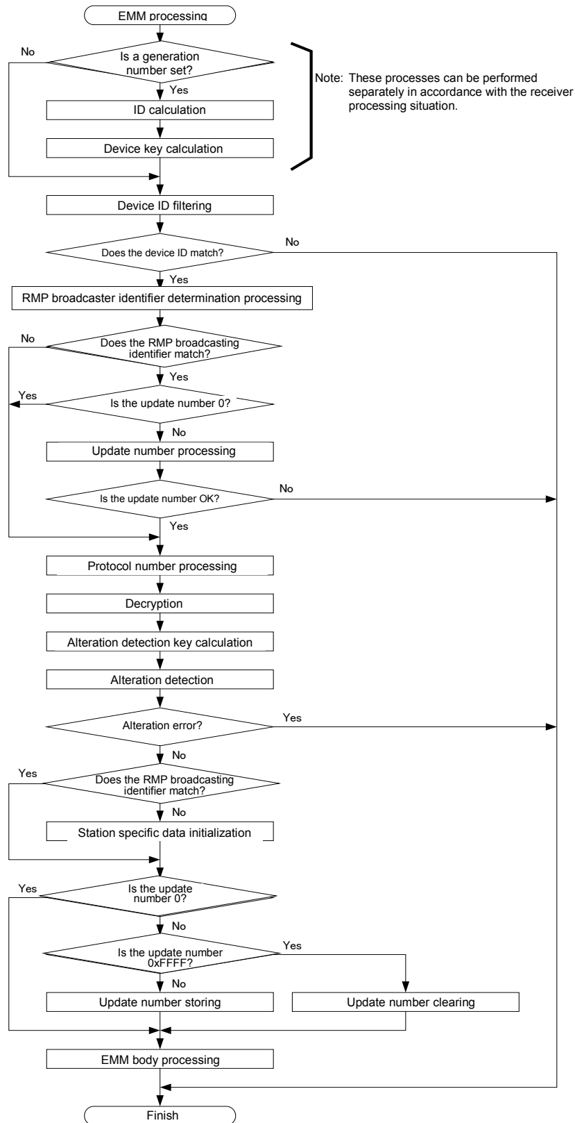
Figure 5-4 EMM process flow
