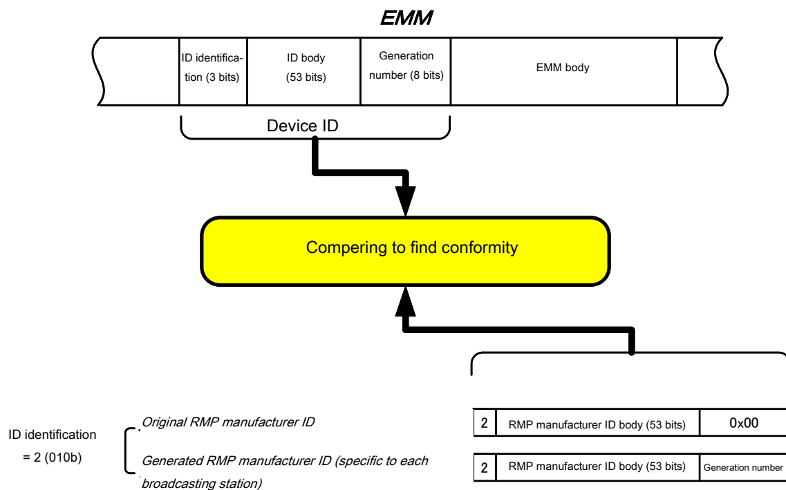
Figure 5-5 Filtering of device IDs
