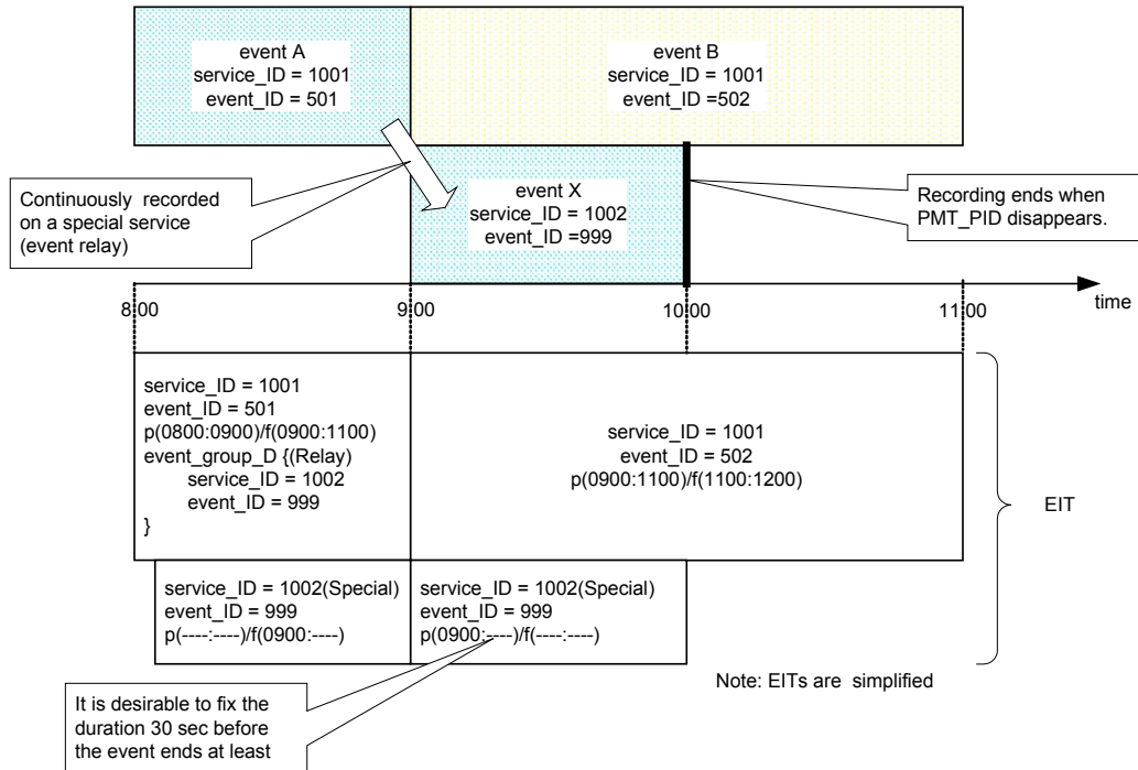
Figure 8-5 Event Relays Using the Special Service
