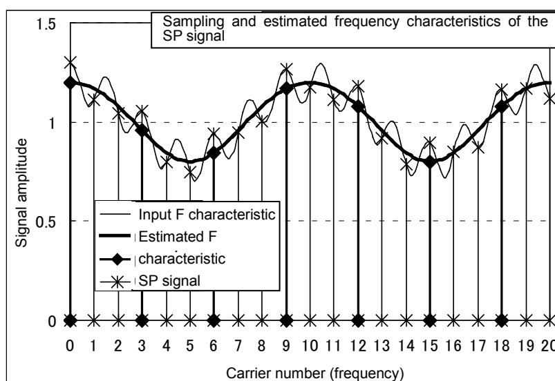
Figure A-21 Frequency characteristic assumed from the SP signal
