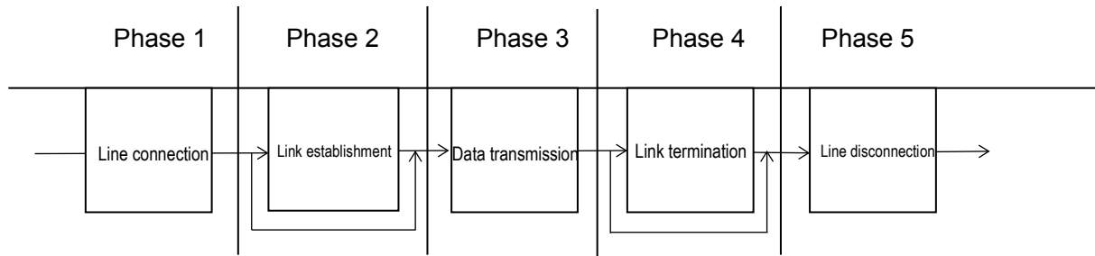
Figure 5-1 Transmission phases
