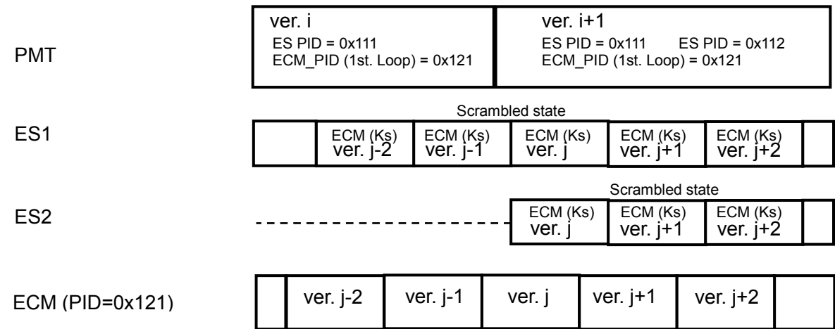
Figure 4-5 When ECM_PID is not changed
