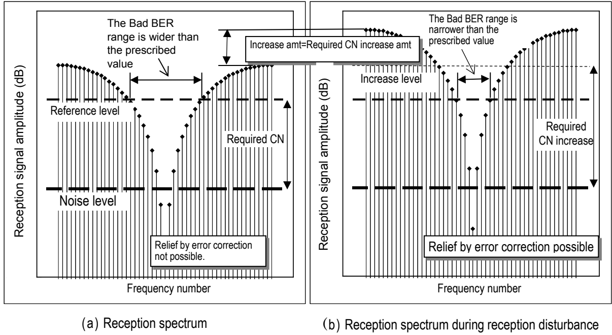
Figure A-1 Example of a reception spectrum when there are SFN waves
