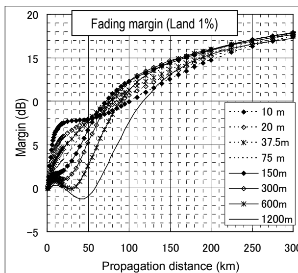
Figure A-30 Fading margin example
