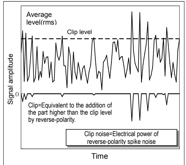
Figure A-3 Clip noise
