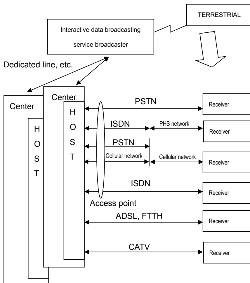
Figure 4-1 Interactive data broadcasting service format conceptual diagram
