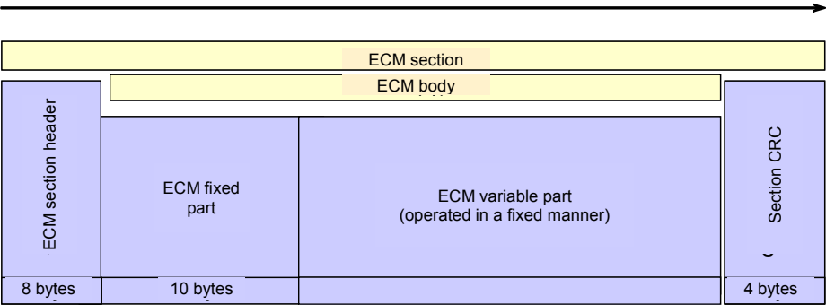
Figure 4-1 ECM-F1 section structure
