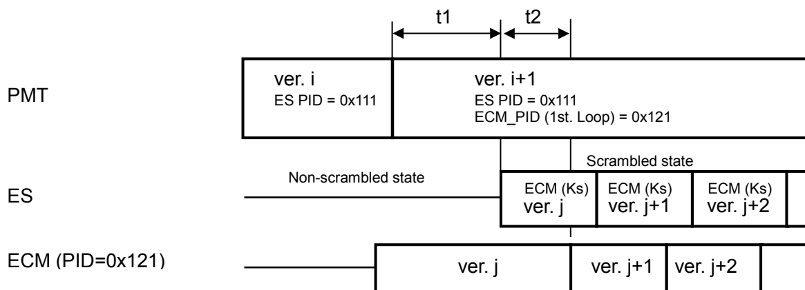
Figure 4-2 Start of scrambling
