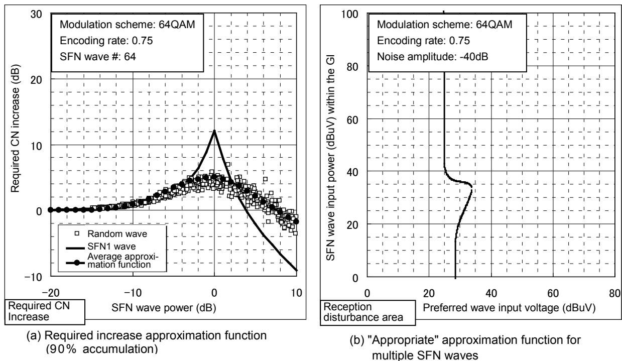
Figure A-17 Multiple SFN wave characteristics example (64QAM-3/4: Least square function)
