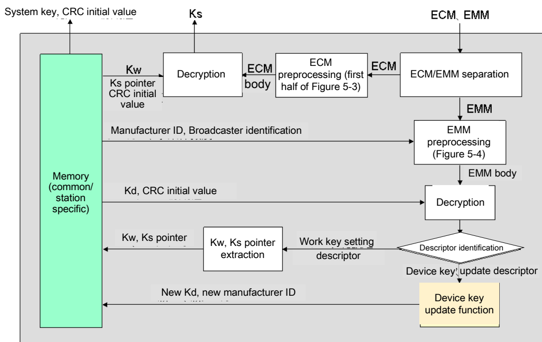
Figure A-1 RMP module function
