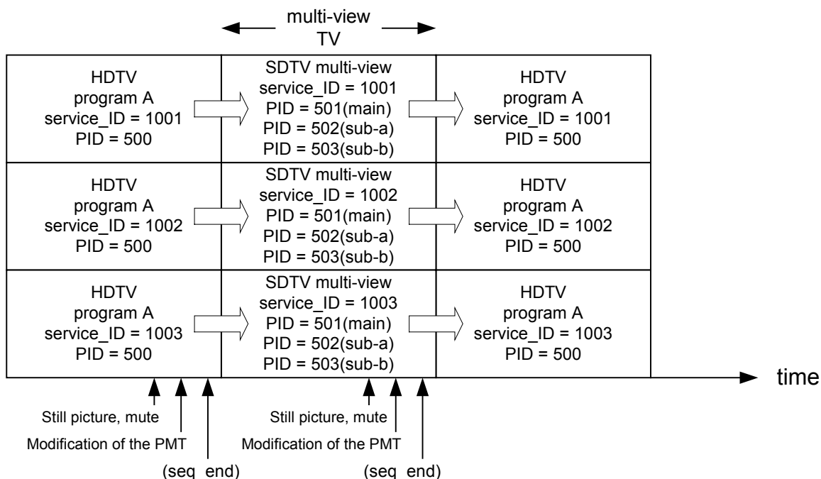
Figure 8-4 Coexistence of Multiple service identifier and MTV
