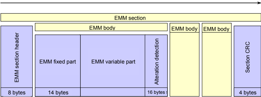
Figure 4-8 EMM section structure
