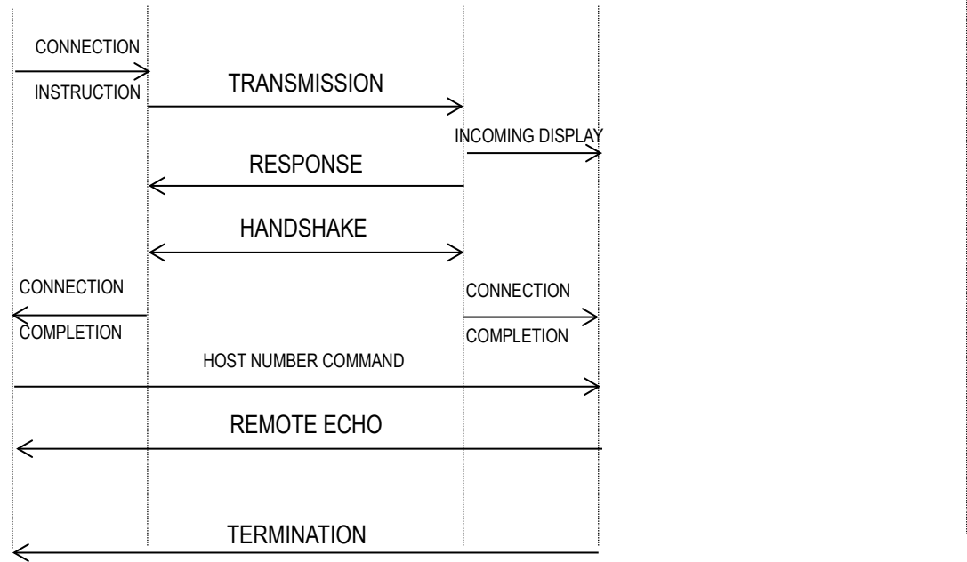
Figure 5-6 Abnormal sequence(Center call rejection)
