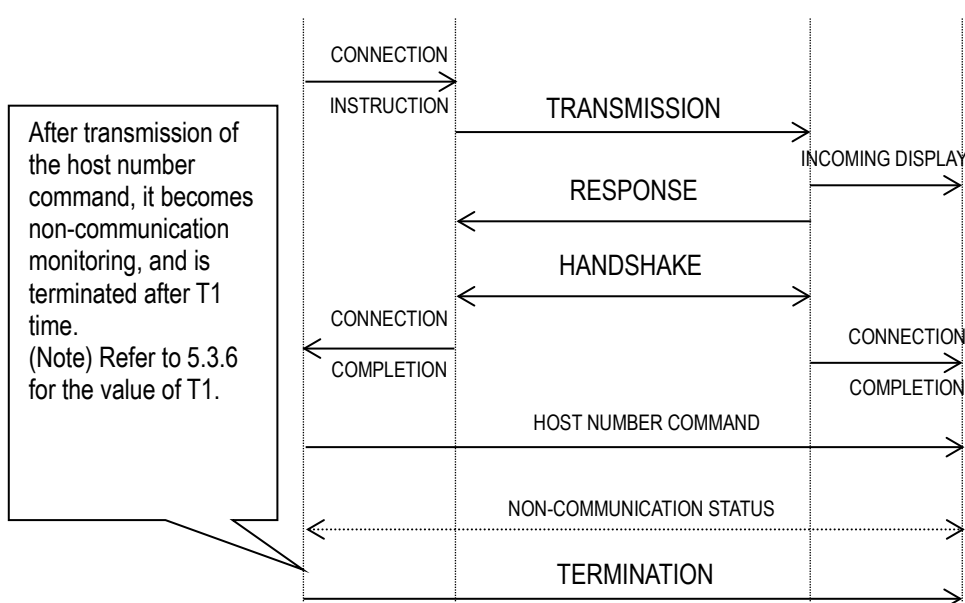
Figure 5-8 Abnormal sequence (receiverside time-out for the remote echo standby)
