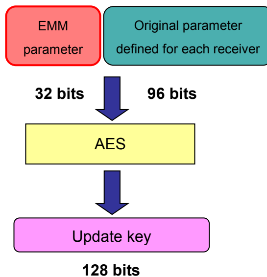
(a) AES encryption (ECB mode)
