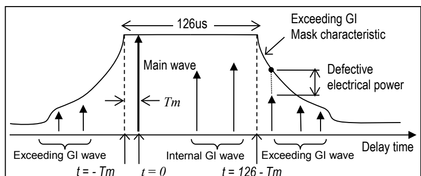
Figure A-29 FFT window optimal setting
