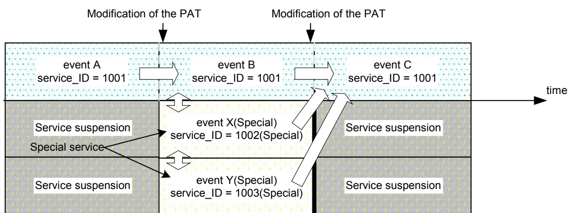
Figure 8-2 An Example of Broadcasting Special services (One Regular Service and Two Special services)
