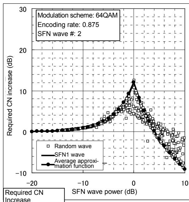
(a) Required CN increase approximation function (90 % Accumulation)
