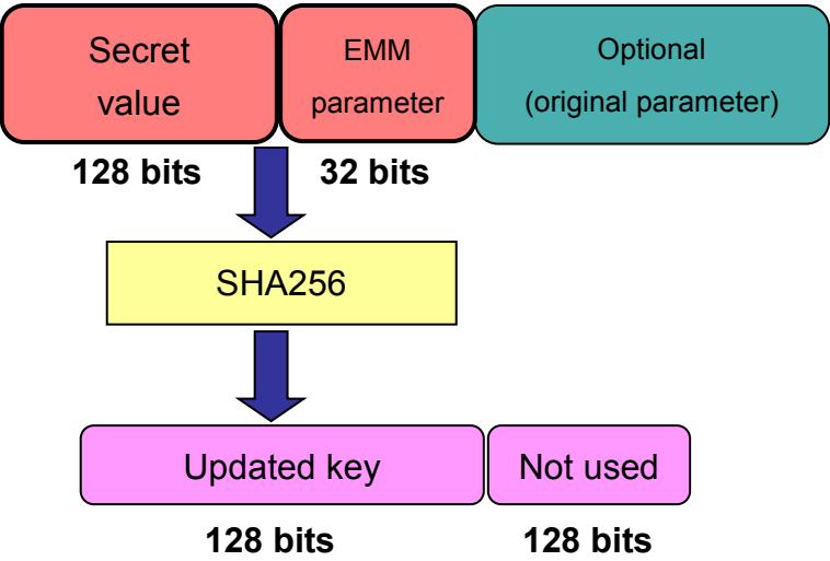
(b) Hash function (SHA256)
