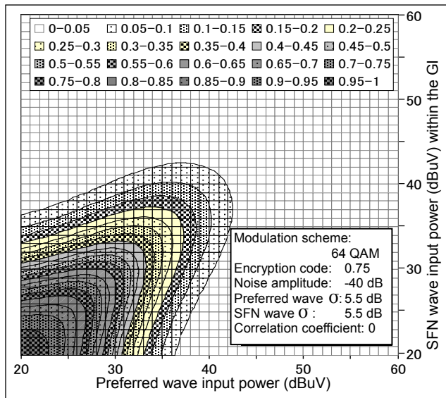
Figure A-7 SFN reception disturbance generation probability example(64QAM-3/4)
