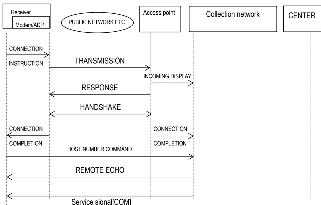
Figure 5-3 Normal sequence
