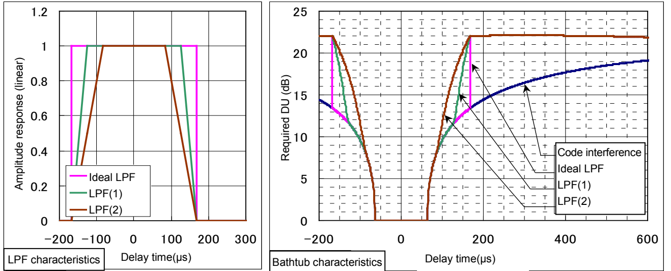
Figure A-25 Interpolation LPF characteristic and required DU characteristic (Depends on Equation (28) 64QAM-3/4 and Namp=-35dB)
