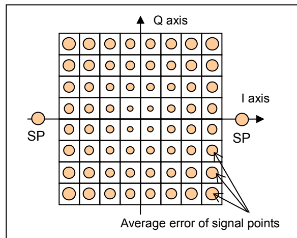
Figure A-23 Average error influence level with signal points
