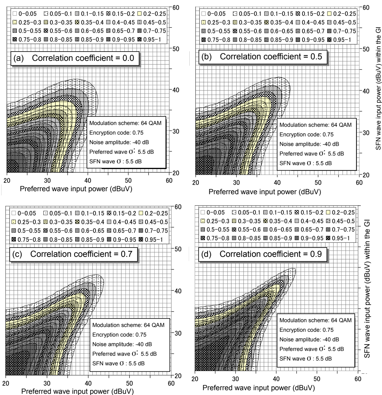
Figure A-9 Change in the reception disturbance generation probability according to cross-correlation coefficient of location dispersion
