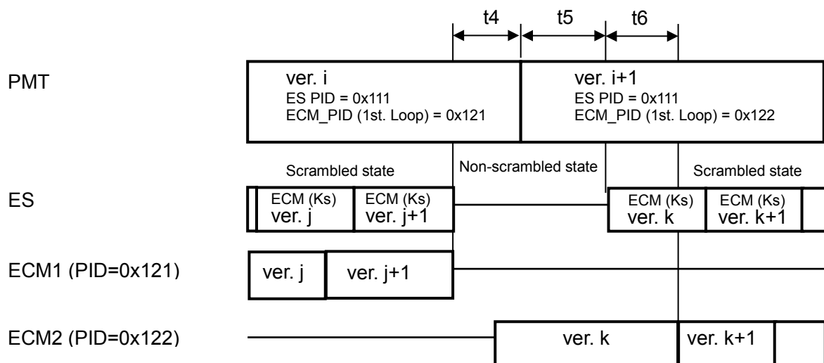
Figure 4-4 When ECM_PID is changed
