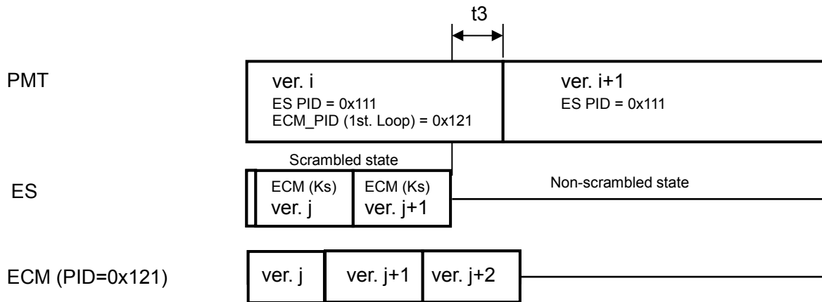
Figure 4-3 End of scrambling
