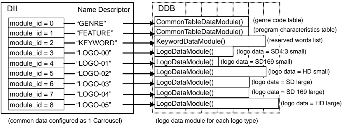
Figure 5-6 Sample common data Carrousel structure
