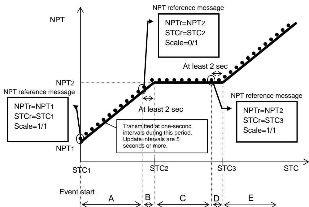
Figure 5-7 Transmission of NPT reference messages
