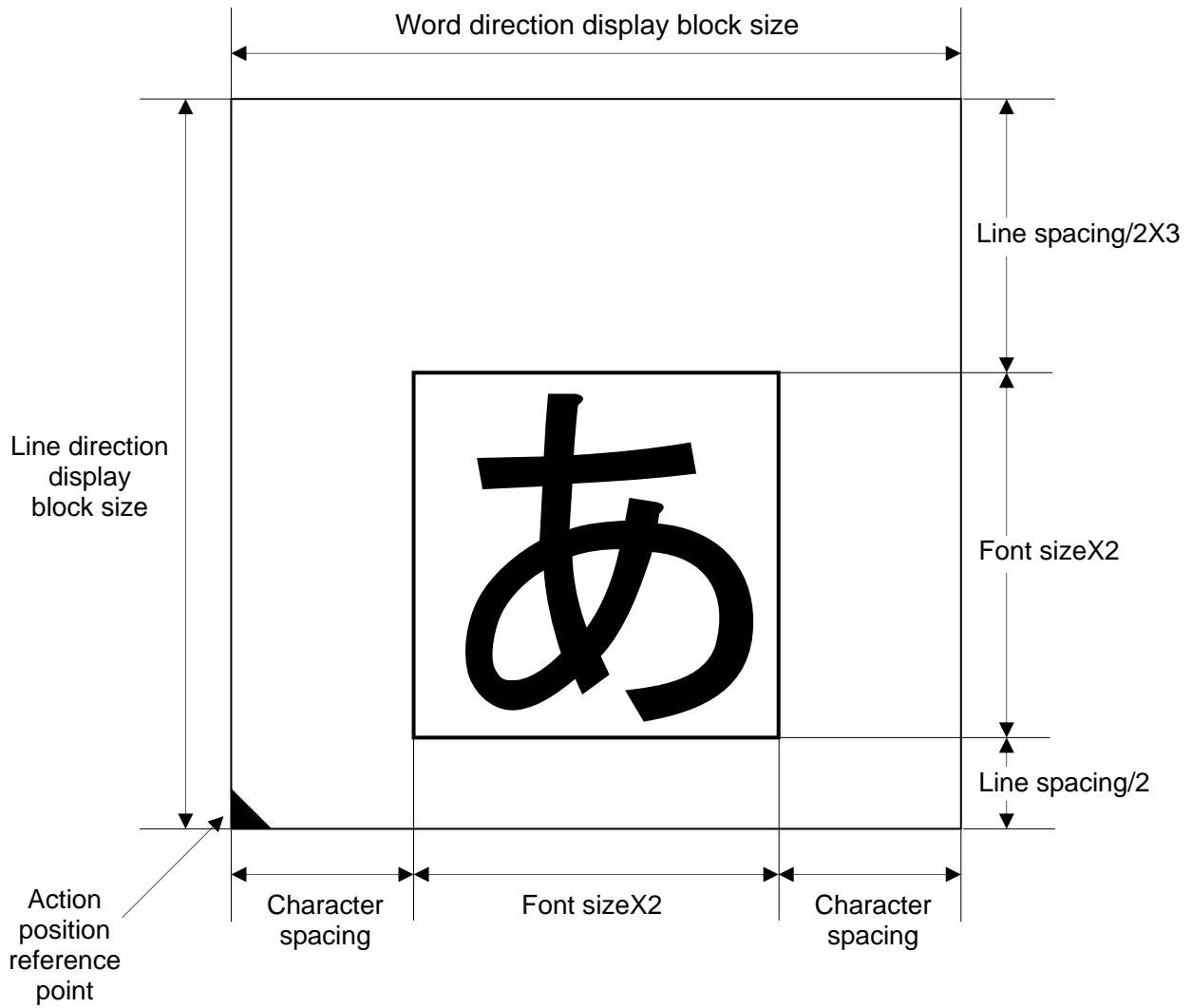
Figure 7-8 Relationships among display block, font size (double height, width), character spacing, and line spacing in horizontal writing
