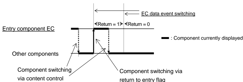
Figure 5-6 Entry component data_event_id updating and the return to entry flag
