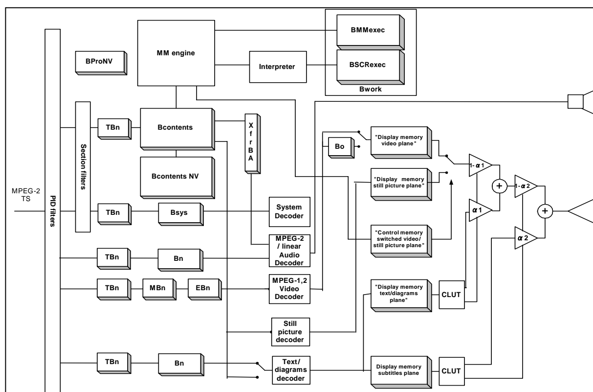
Figure 4-2 Basic receiver unit reference model
