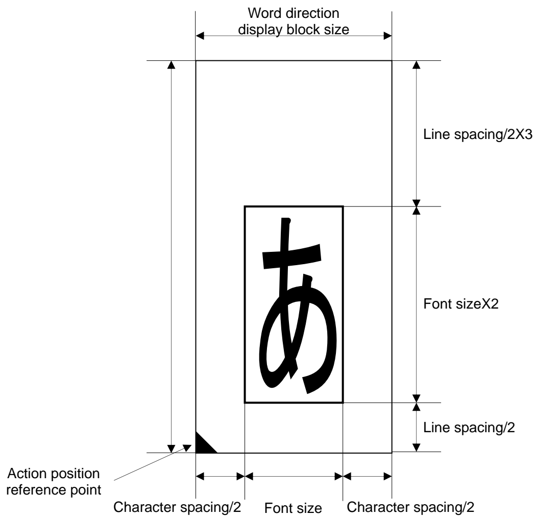
Figure 7-6 Relationships among display block, font size (double-height), character spacing, and line spacing in horizontal writing
