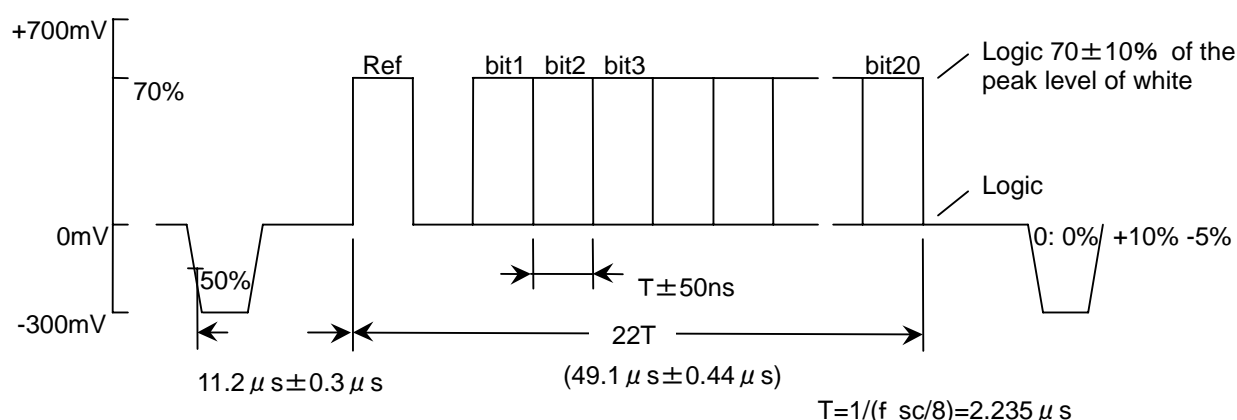
Figure 7-6 Identification signal waveform for a 480i component transmission
