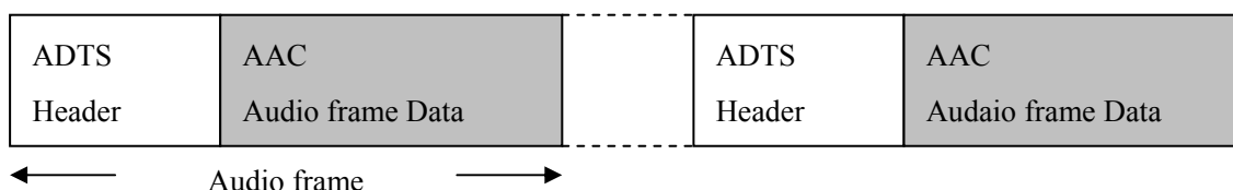
Figure 6-1 ACC audio file data format
