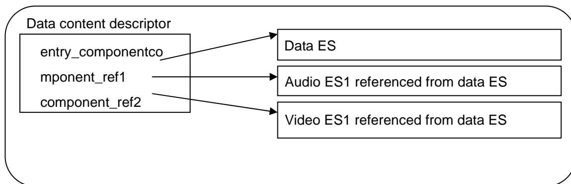
Figure 5-2 Content and ES structure
