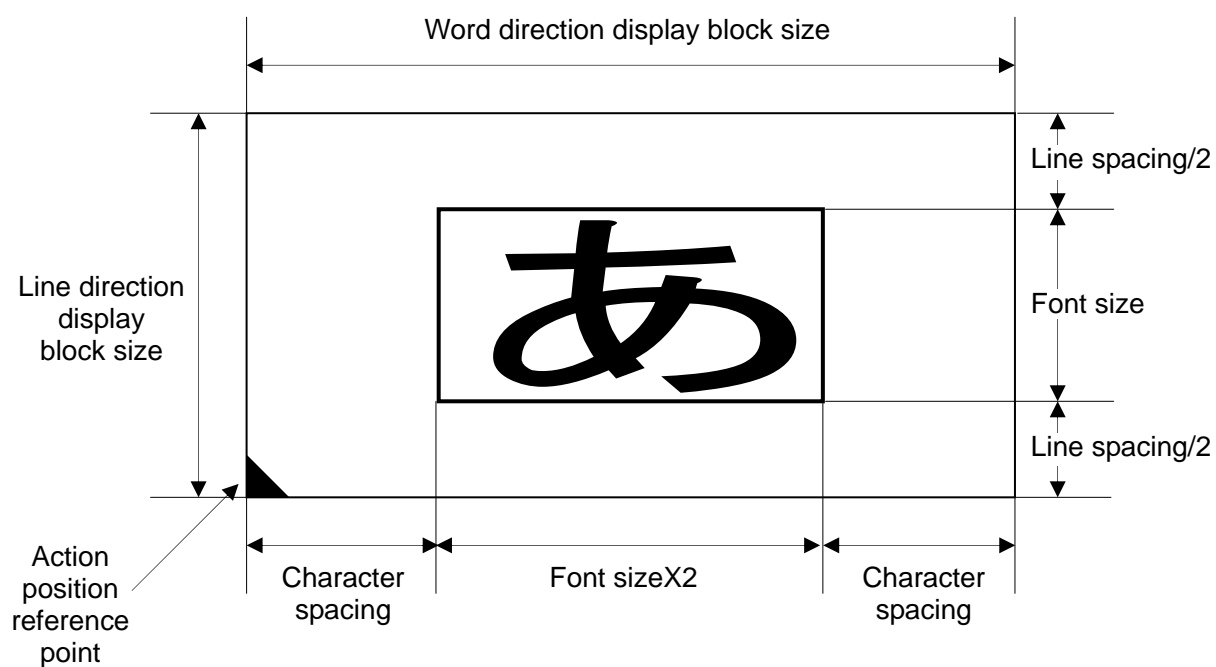
Figure 7-7 Relationships among display block, font size (double-width), character spacing, and line spacing in horizontal writing
