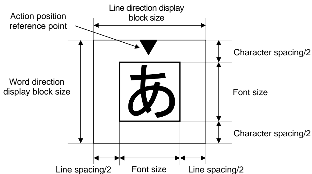
Figure 7-9 Relationships among display block, font size (standard), character spacing, and line spacing in vertical writing
