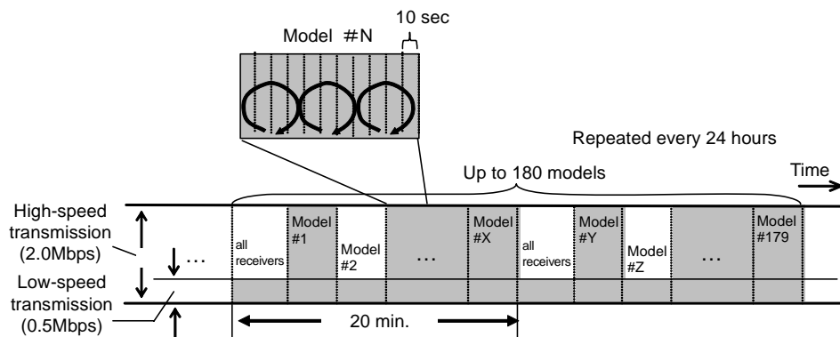
Figure 5-2 Reference model of download content transmission schedule (low transmission speed for data common to all receivers and models #2 and #Z, high transmission speed for all others)
