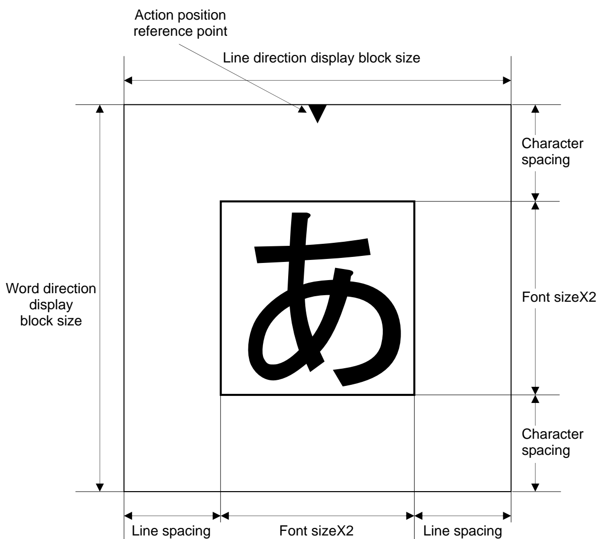
Figure 7-14 Relationships among display block, font size (double height, width), character spacing, and line spacing in vertical writing
