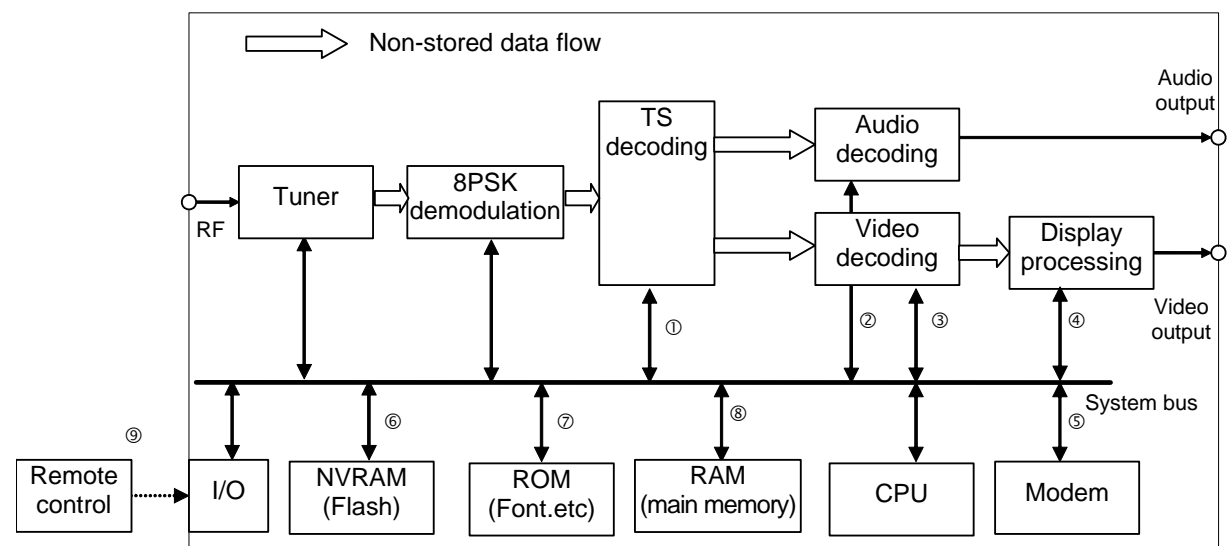
Figure 4-1 Hardware configuration for basic receiver unit
