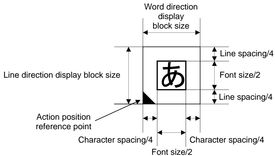
Figure 7-5 Relationships among display block, font size (small), character spacing, and line spacing in horizontal writing
