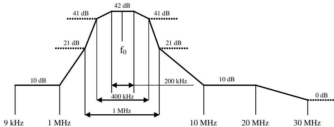
Figure 4.3.1.2.1: Modem attenuation
