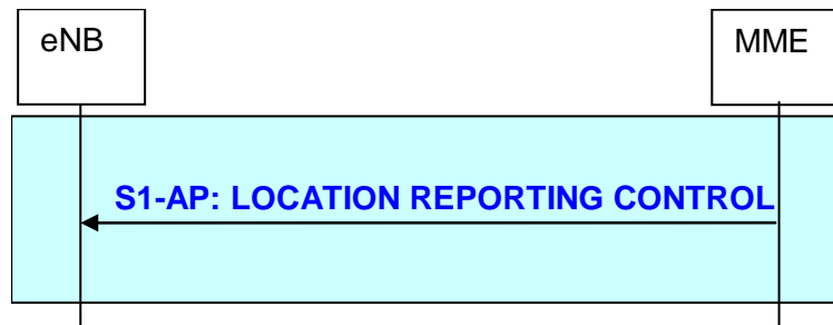
Figure 19.2.2.11.1-1: Location Reporting Control procedure
