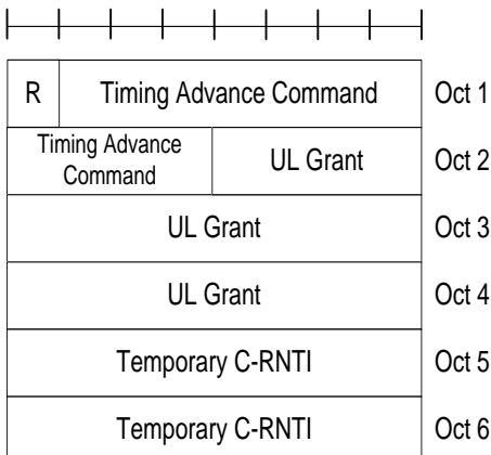
Figure 6.1.5-3: MAC RAR
