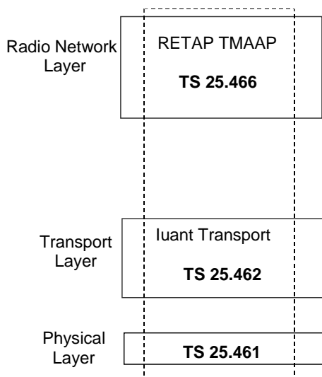
Figure 6.4.1: Iu-UTRAN Interface Technical Specifications
