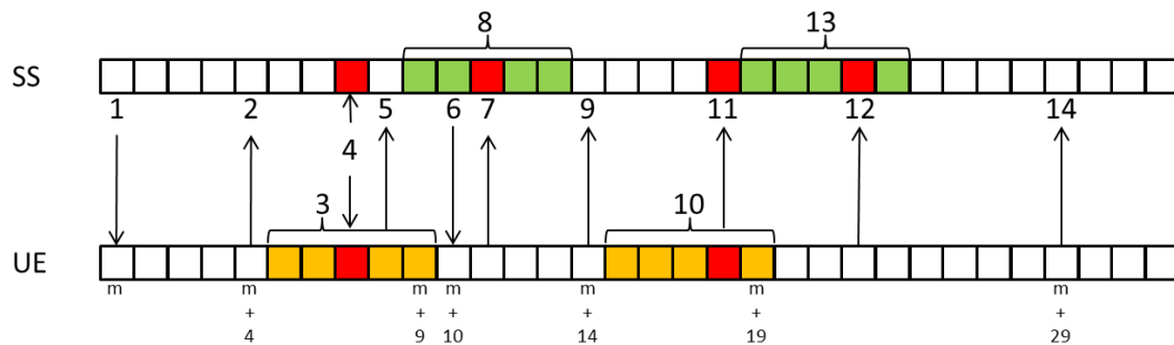
Figure: 8.16.37.5-2 Procedure derivation for Activation (the case where the band relation between PCC and SCells are inter-band)
