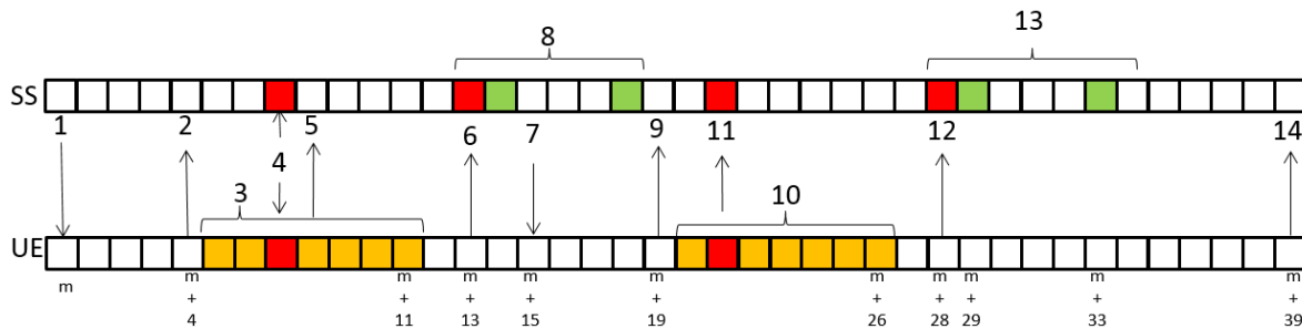
Figure 8.16.40.5-1: Procedure derivation for Activation (the case where the band relation between PCC and SCells are inter-band)
