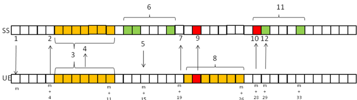
Figure 8.16.38.5-3: Procedure derivation for Activation (the case where the band relation between PCC and SCell1 is intra-band and SCell2 is inter-band)
