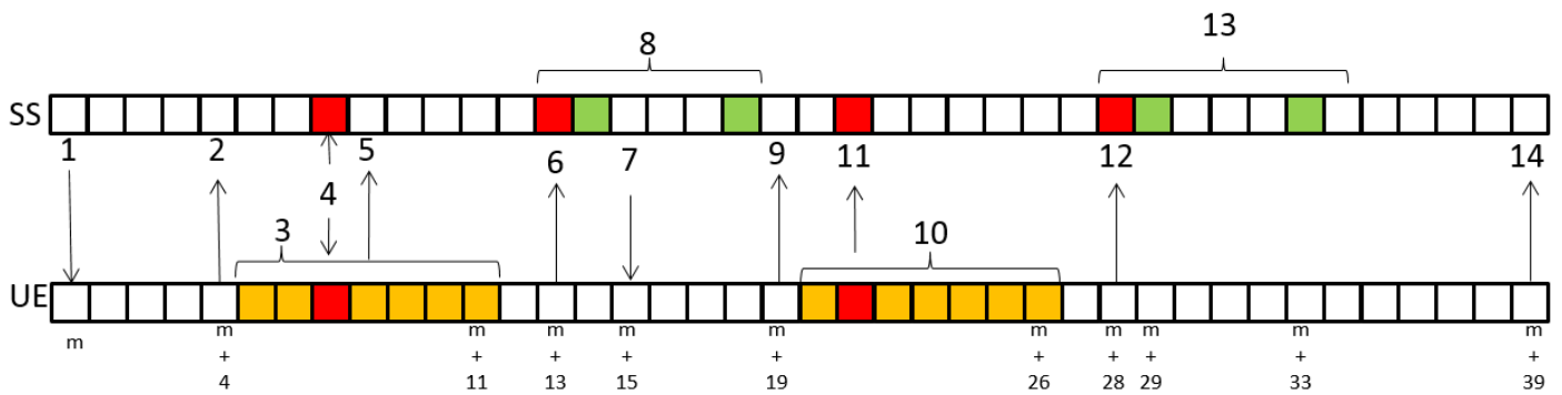
Figure 8.16.42.5-2: Procedure derivation for Activation (the case where the band relation between PCC and SCells are inter-band)
