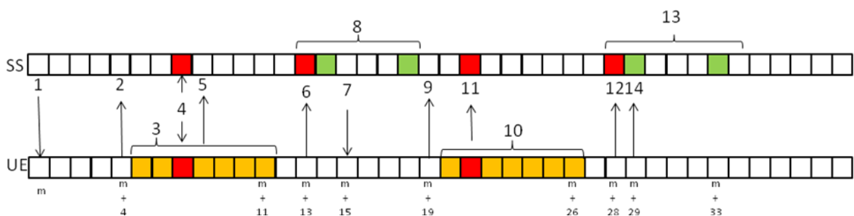
Figure 8.16.38.5-2: Procedure derivation for Activation (the case where the band relation between PCC and SCells are inter-band)
