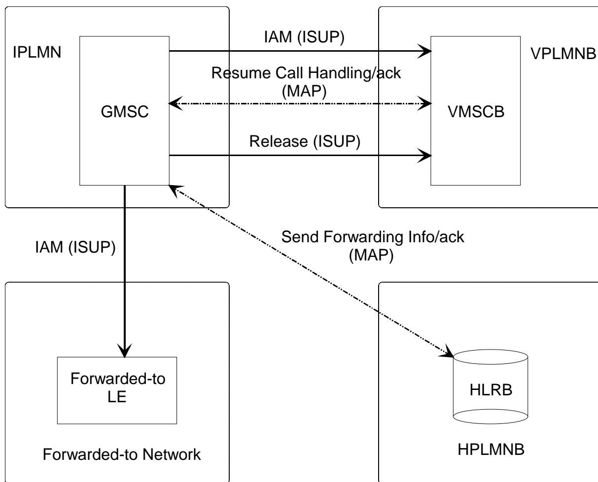
Figure 2: Architecture for optimal routeing of late call forwarding
