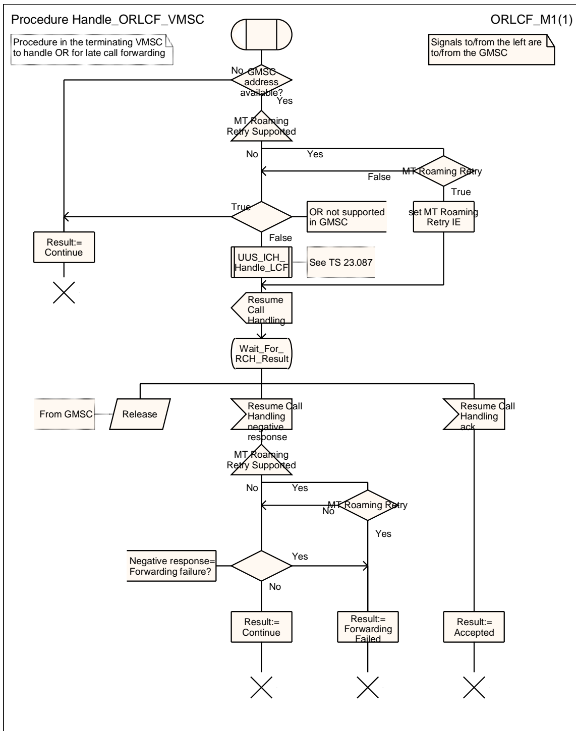
Figure 12: Procedure Handle_ORLCF_VMSC
