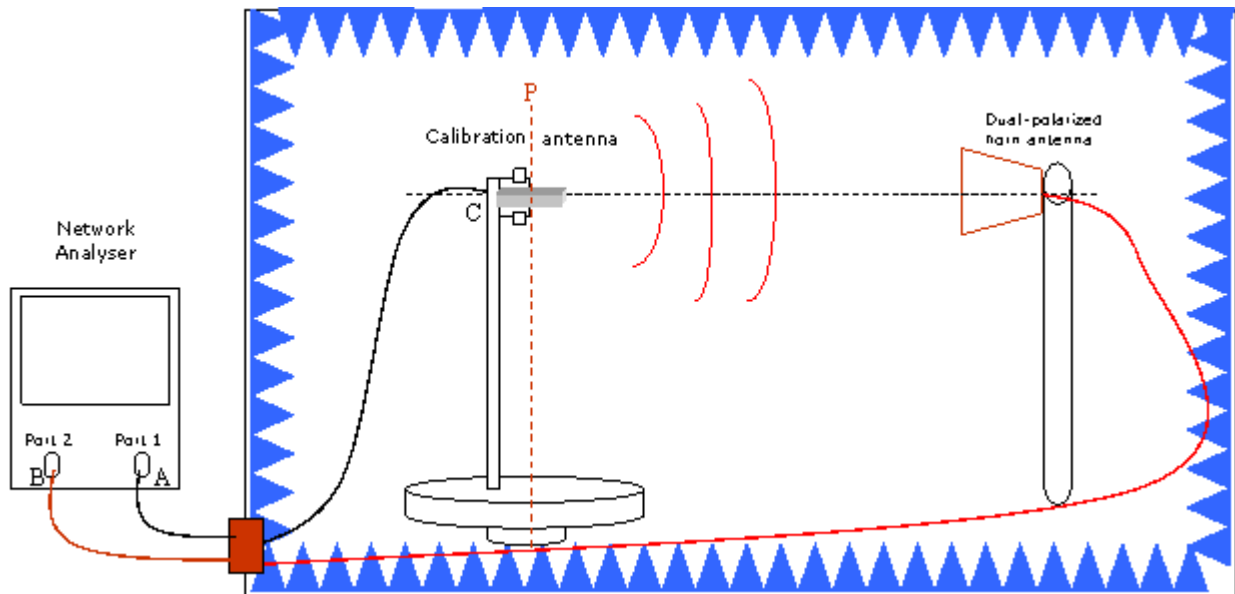
Figure B.1 Calibration/substitution procedures using a vector network analyser.
