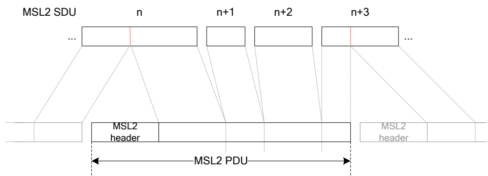
Figure 4.87: MSL2 PDU Structure
