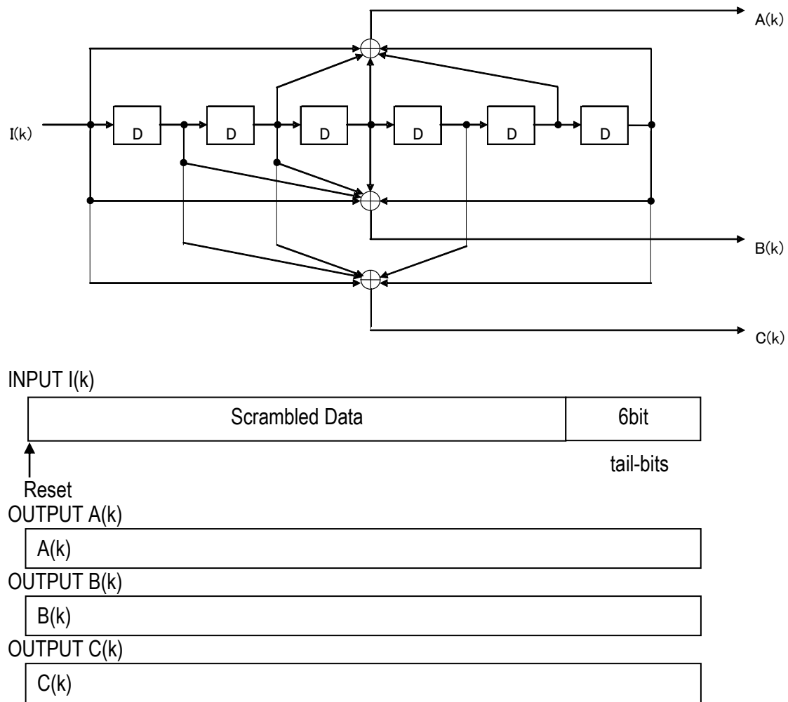
Figure 3.21 Generation Polynomial and Application Range of Convolutional Code
