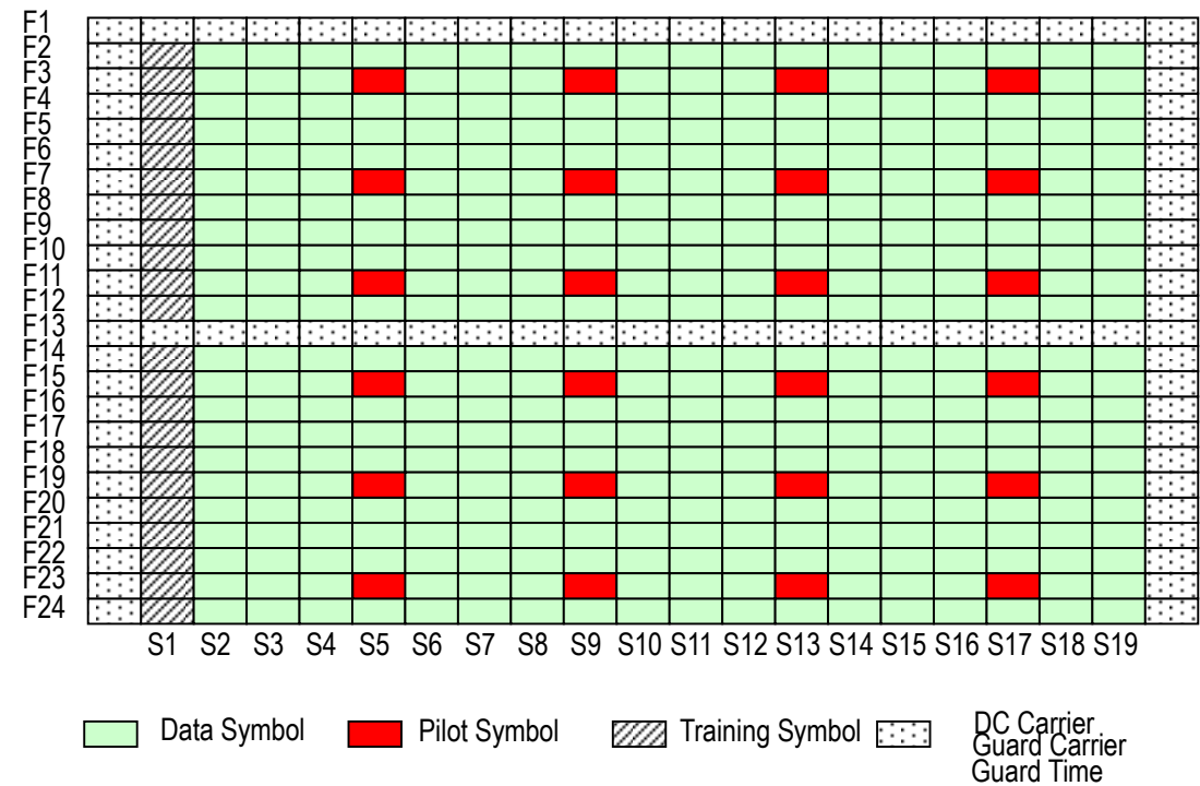
Figure 3.70 OFDM PRU Structure for EXCH format (a-1)
