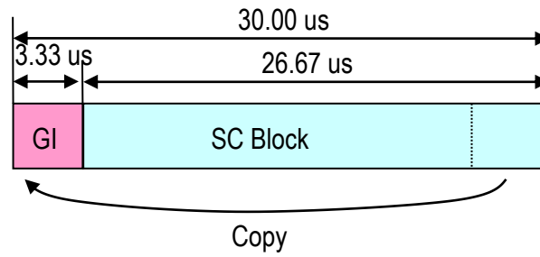
Figure 3.7 SC Block with Guard Interval (S2 – S19)
