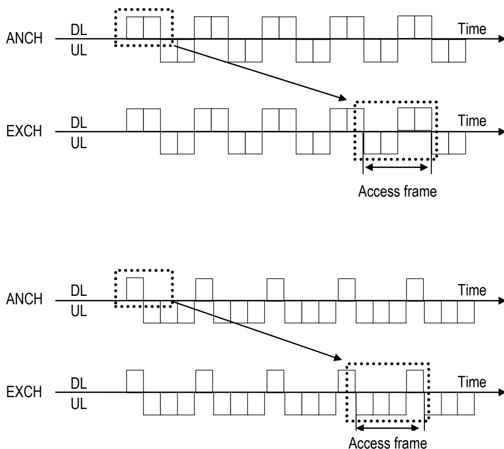
Figure 6.10 Timing 2 for 2.5ms frame
