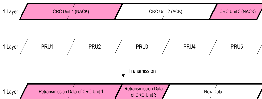
Figure 3.45 In case of Retransmission of except for EMB-MIMO(only 1 layer)
