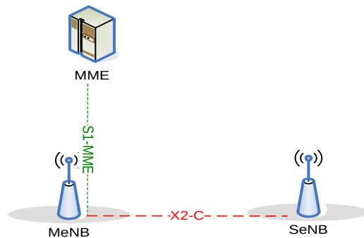
Figure 10.8.1.1.2-4 C-Plane connectivity of eNBs involved in Dual Connectivity [60]
