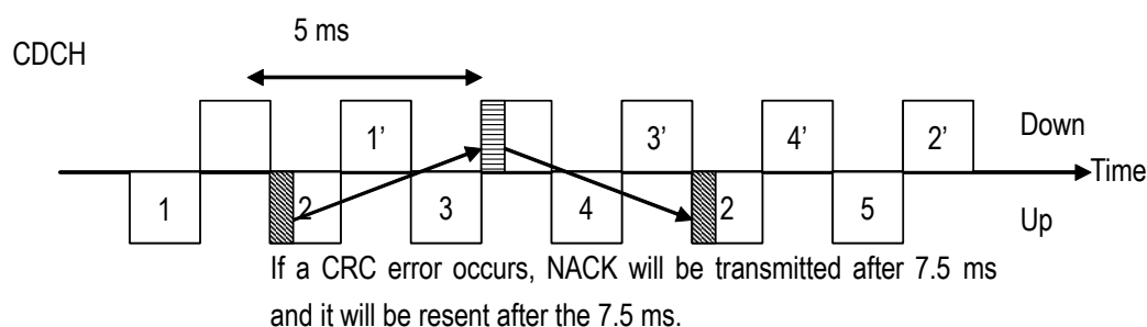
Figure 9.2 ARQ Retransmission Timing
