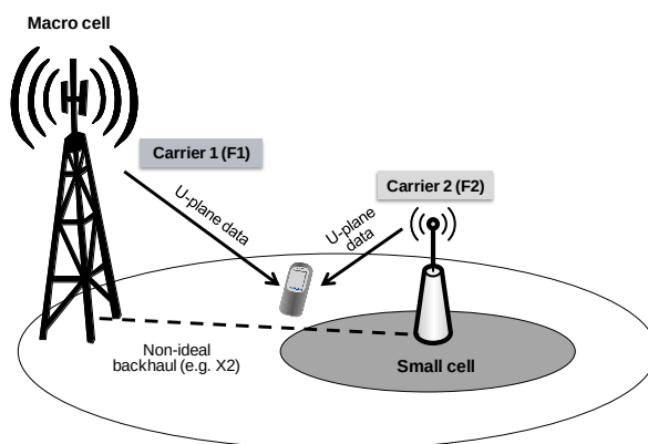
Figure 10.8.1.1.2-6 Inter-node radio resource aggregation [66]
