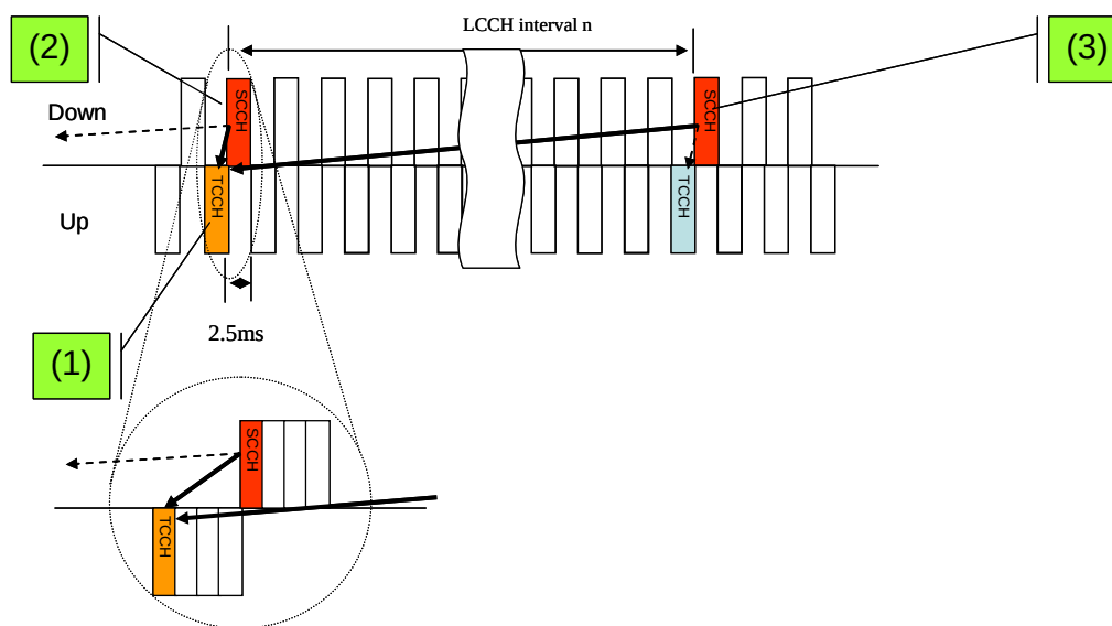
Figure 6.3 Relation between LCH Assignment Request (TCCH) and LCH Assignment (SCCH)
