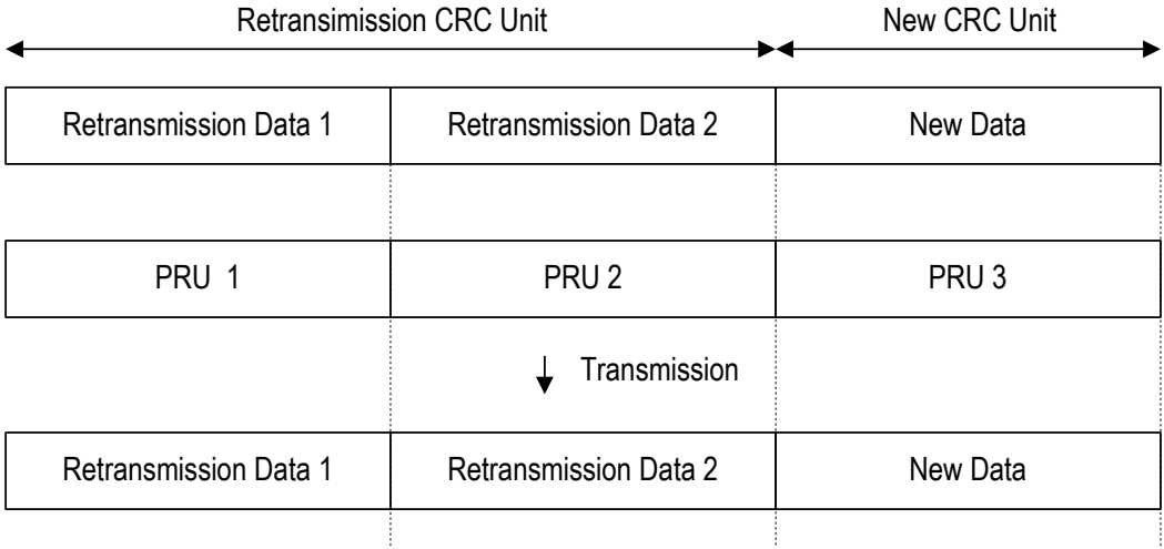
Figure 3.48 The case when Retransmission CRC Unit Size equals to Retransmission PRU Size (1)
