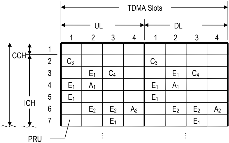
Figure 4.2 Example of ICH Usage
