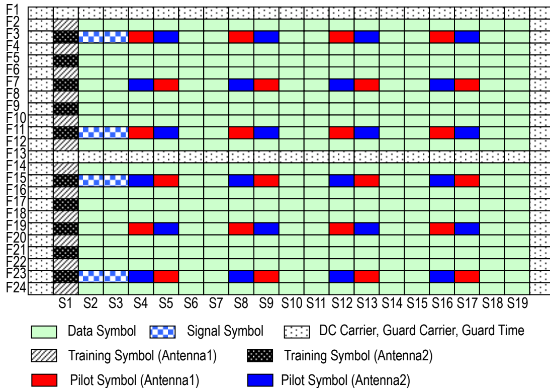
Figure 3.72 OFDM PRU Structure for EXCH format (a-3)
