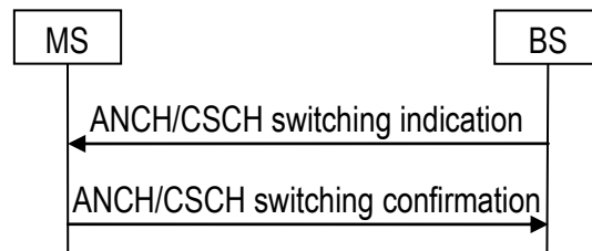
Figure 9.30 BS Origin ANCH/CSCH Scheduling Change
