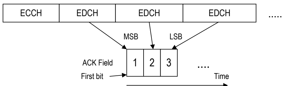
Figure 4.39 Correspondence between EDCH and ACK Field
