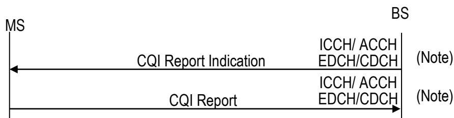
Figure 8.28 CQI Report Indication Sequence
