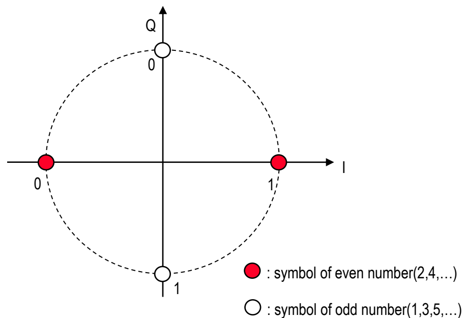
Figure B.2 \pi/2 -BPSK
