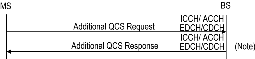
Figure 8.20 Additional QCS Sequence
