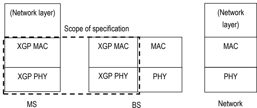
Figure 2.18 Protocol Stack for XGP
