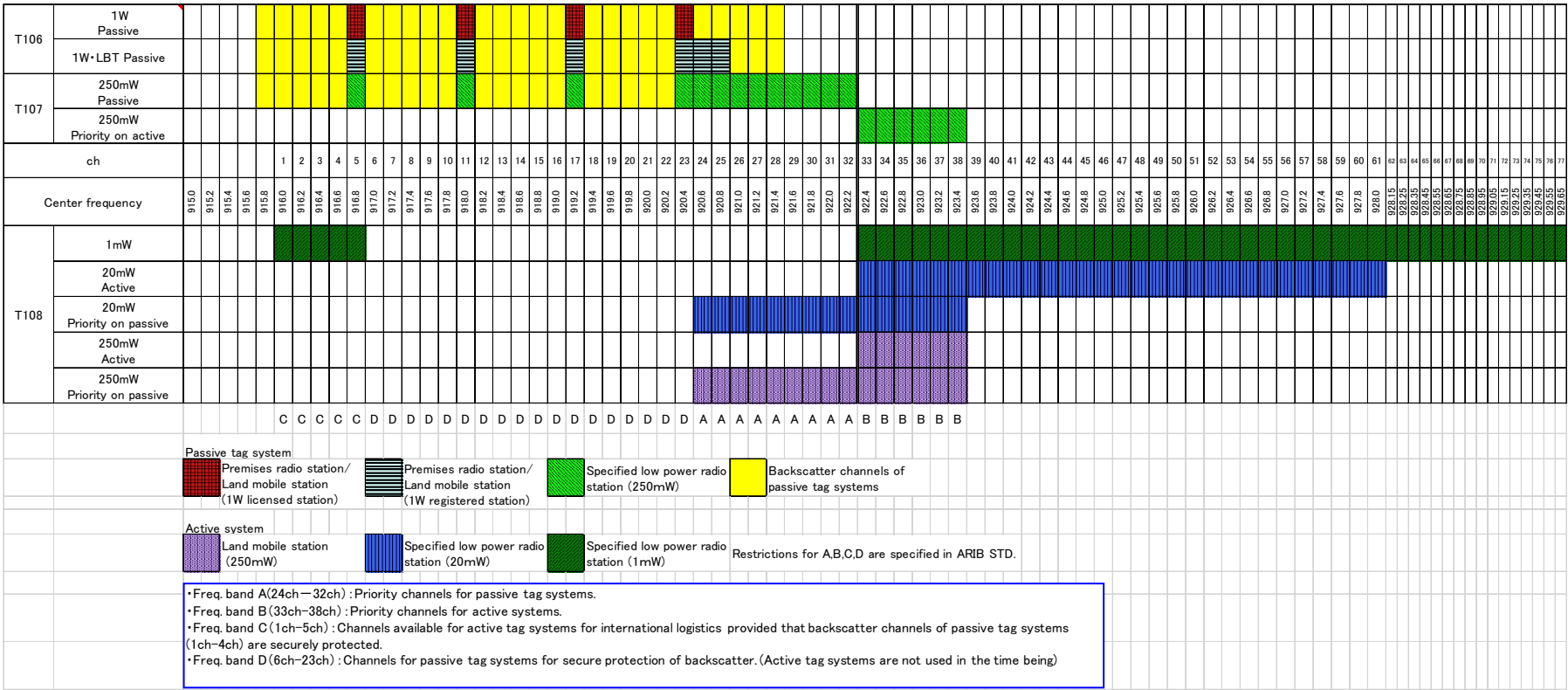
Figure S-5 Channel plan for 920MHz-band radio equipment
