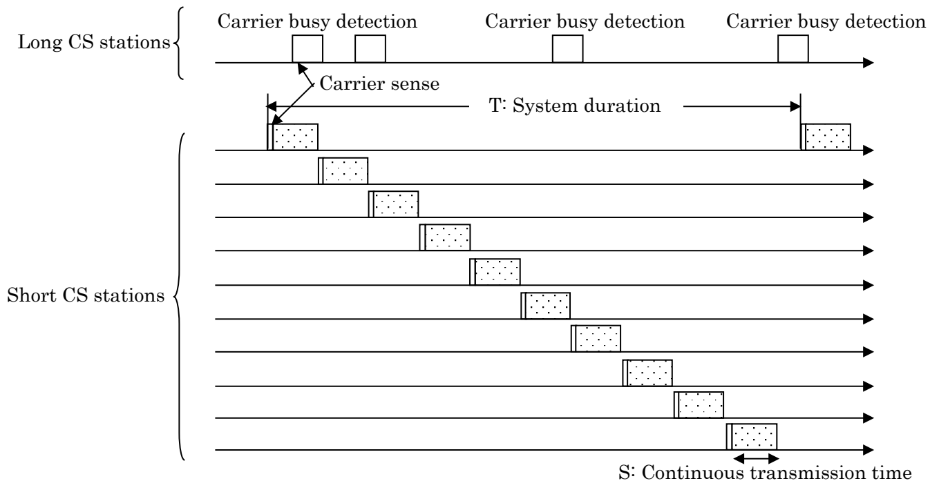
Figure S-1 Time sequence diagram for a case in which short CS stations within an interference range periodically repeat data transmissions and occupy a channel more than long CS stations.
