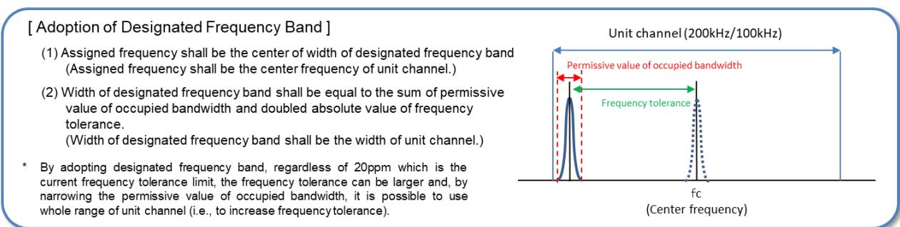
Figure S-2 Adoption of designated frequency band
