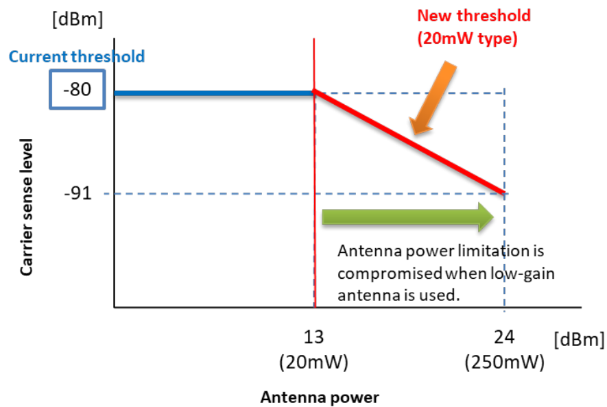
Figure S-4 Adjustment of carrier sense level
