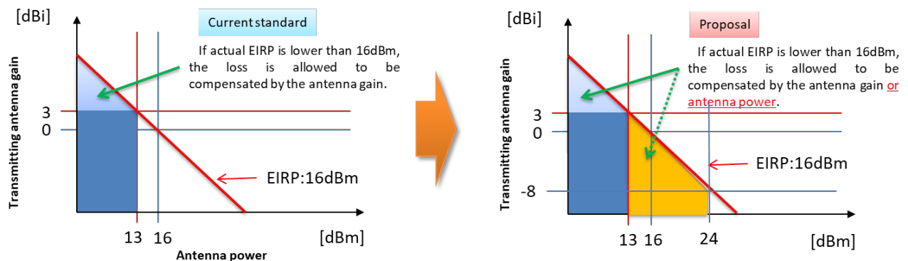
Figure S-3 Adoption of EIRP method
