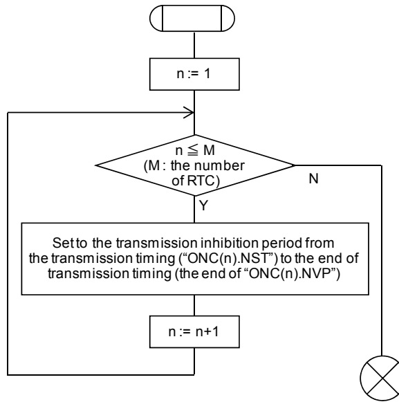
Figure C3-27 MAC sublayer (mobile station) SDL-13
