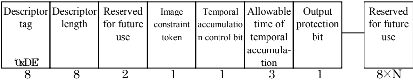
Figure 6-70 Data structure of content availability descriptor
