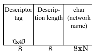
Figure 6-20 Data structure of Network name descriptor
