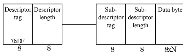
Figure L-1 Data construction of composite descriptor for tag value extension
