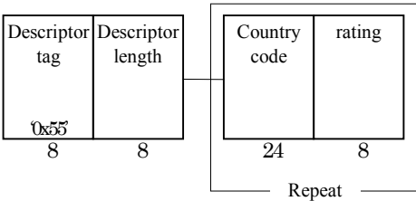
Figure 6-38 Data structure of Parental rating descriptor
