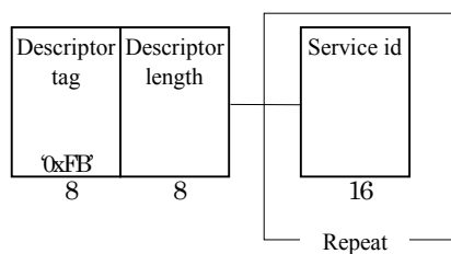
Figure 6-57 Data structure of Partial reception descriptor
