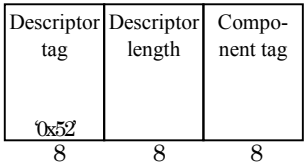
Figure 6-35 Data structure of Stream identifier descriptor
