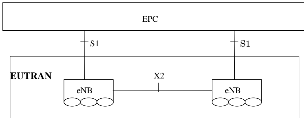
Figure 6.1-1 Overall architecture
