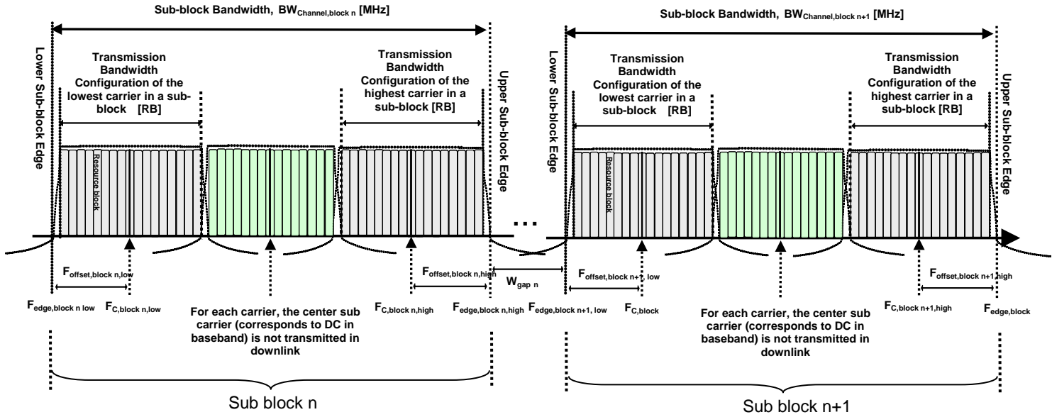
Figure 6.2.1.1-1 Non-contiguous intraband CA terms and definitions
