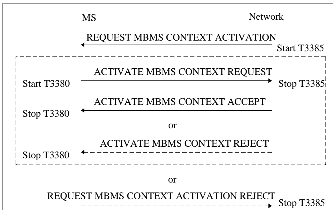
Figure 6.10/3GPP TS 24.008: MBMS context activation procedure
