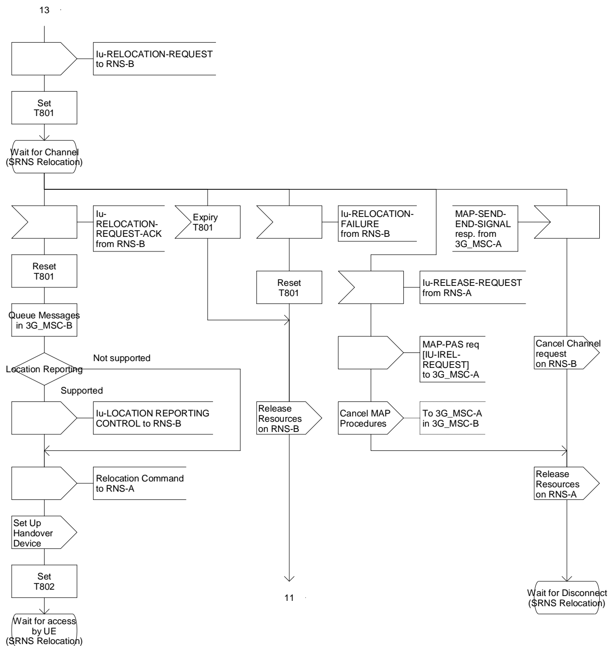
Figure 44 (sheet 44 of 54): Handover control procedure in 3G_MSC-B
