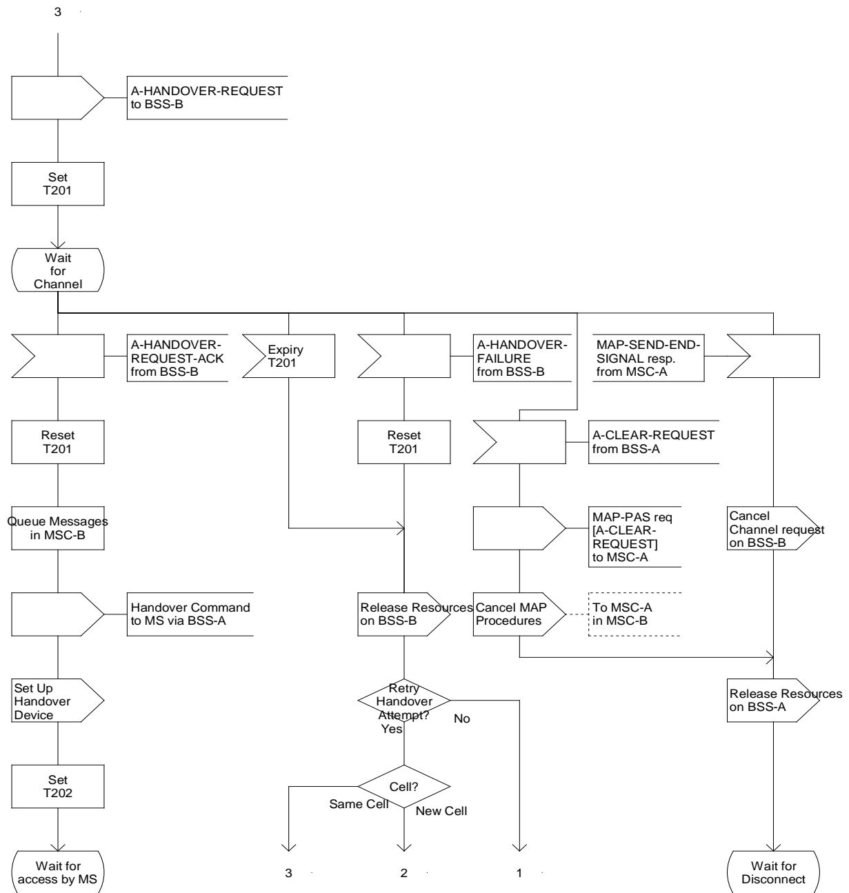
Figure 42 (Sheet 8 of 18): Handover control procedure in MSC-B
