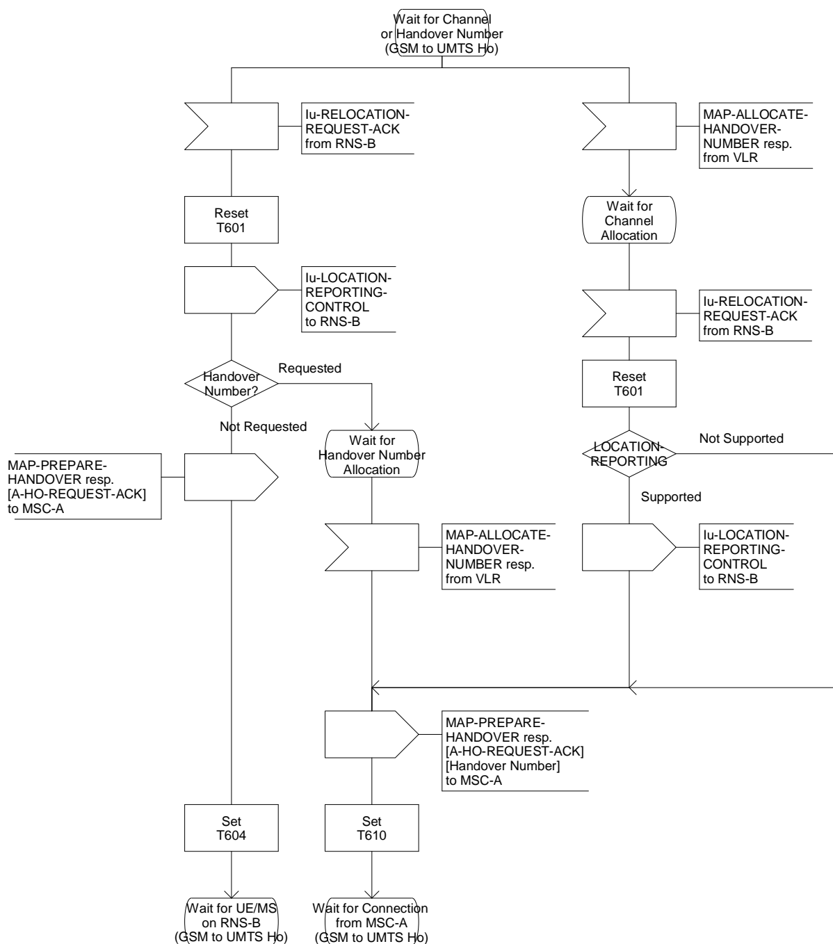
Figure 44 (sheet 2 of 54): Handover control procedure in 3G_MSC-B
