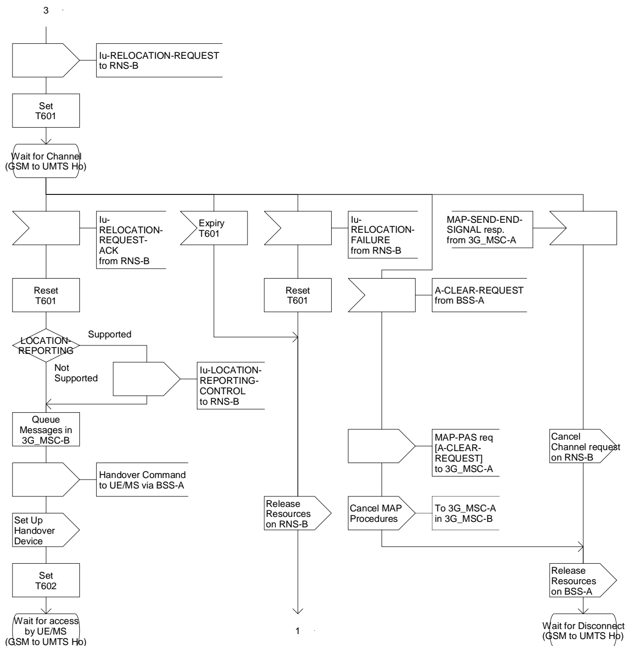
Figure 44 (sheet 8 of 54): Handover control procedure in 3G_MSC-B
