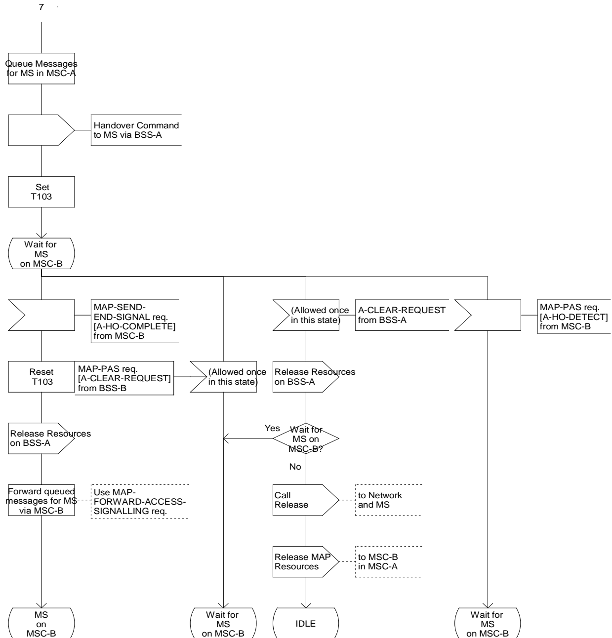
Figure 41 (Sheet 19 of 26): Handover control procedure in MSC-A
