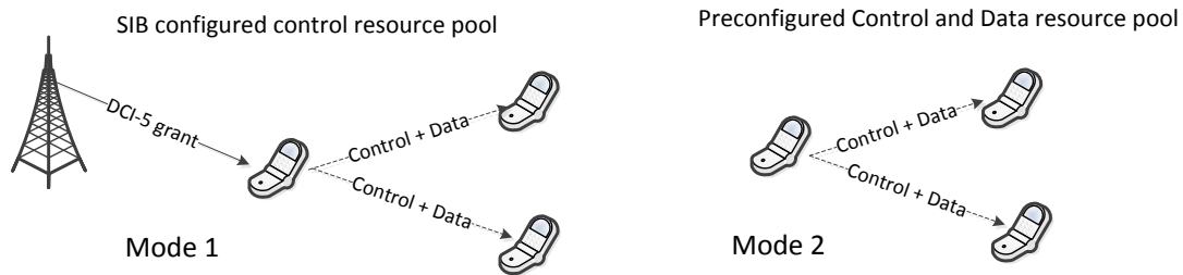
Figure 5.1.1.6.2.3-1 LTE-D operation
