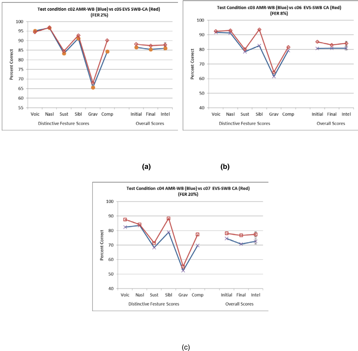
Figure 5.1.2.1-3 P-INTELL profile plots for test conditions (Red: EVS-SWB CA, blue: AMR-WB) (a) c02 vs c05 FER 2%, (b) c03 vs c06 FER 8%, and (c) c04 vs c07 FER 20%.
