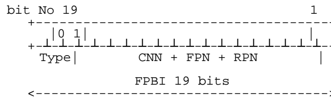
Figure 16: Structure of FPBI class B
