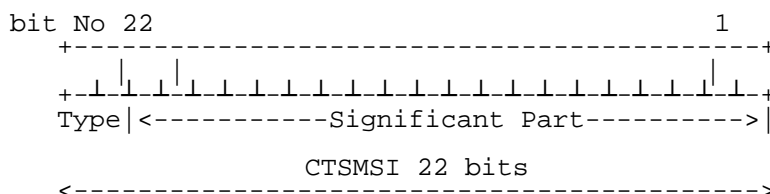
Figure 13: Structure of CTSMSI
