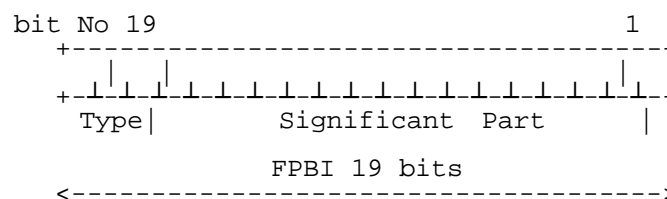
Figure 14: General structure of FPBI
