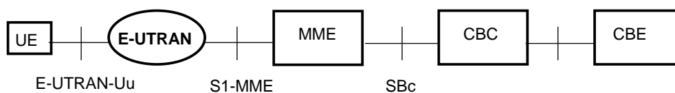
Figure 4.2.3-1: Warning System Architecture for E-UTRAN Access
