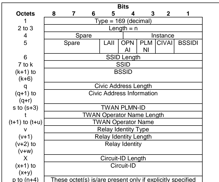
Figure 8.100-1: TWAN Identifier
