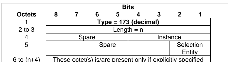
Figure 8.104-1: CN Operator Selection Entity
