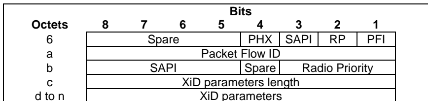
Figure 8.48-3: BSS Container
