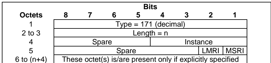
Figure 8.102-1: MBMS Flags
