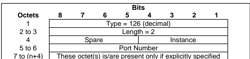
Figure 8.56-1: Port Number
