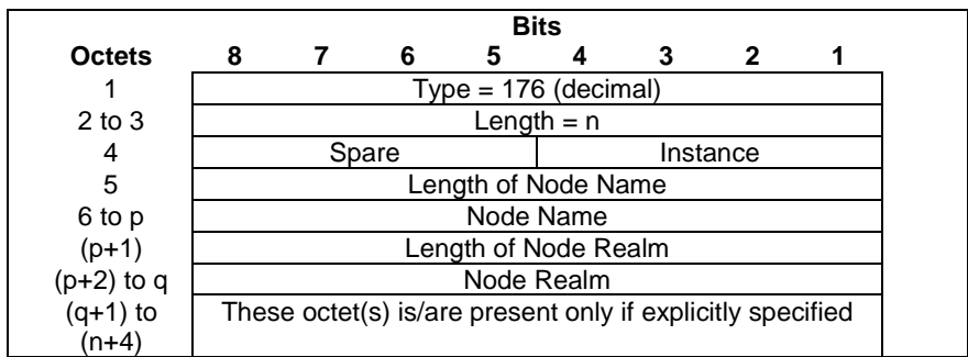
Figure 8.107-1: Node Identifier
