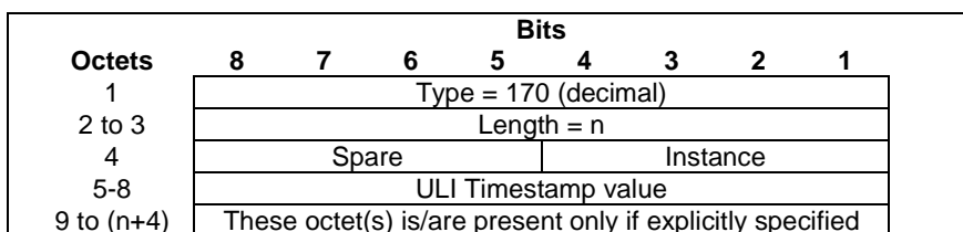
Figure 8.101-1: ULI Timestamp
