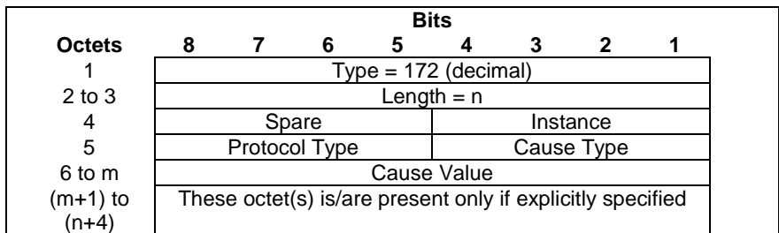
Figure 8.103-1: RAN/NAS Cause
