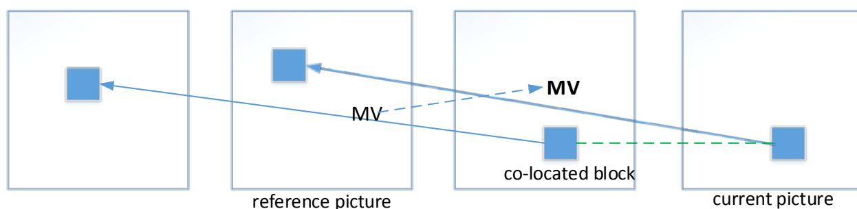
Figure 8: HEVC TMVP
