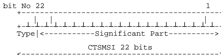
Figure 13: Structure of CTSMSI
