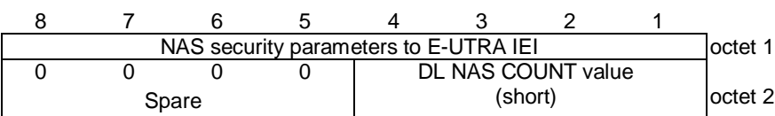
Figure 9.9.2.6.1: NAS security parameters from E-UTRA information element
