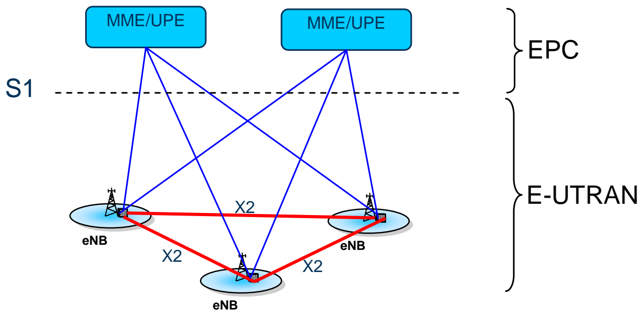
Figure 9.1: E-UTRAN architecture
