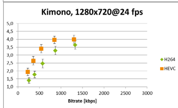
Figure 17: Quality vs. bit rate for Kimono
