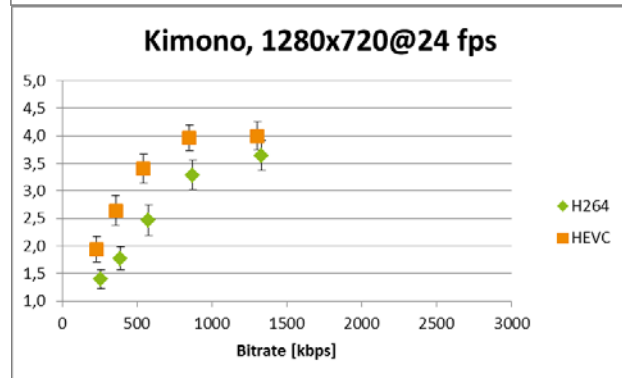
Figure 23: Quality vs. bit rate for Kimono
