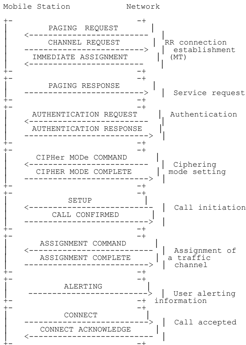
Figure 7.11a/3GPP TS 23.108: Mobile terminating: call establishment without OACSU (early assignment)
