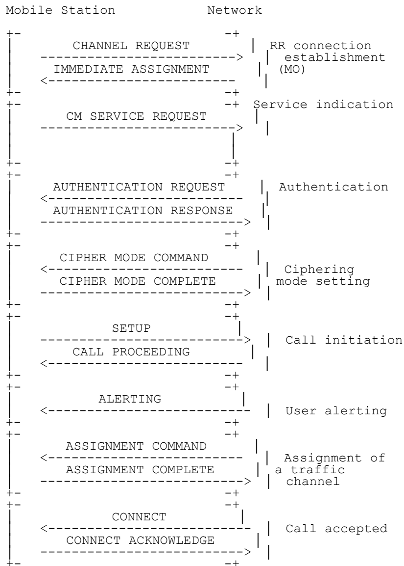
Figure 7.10b/3GPP TS 23.108: Mobile originating call establishment with OACSU (late assignment)
