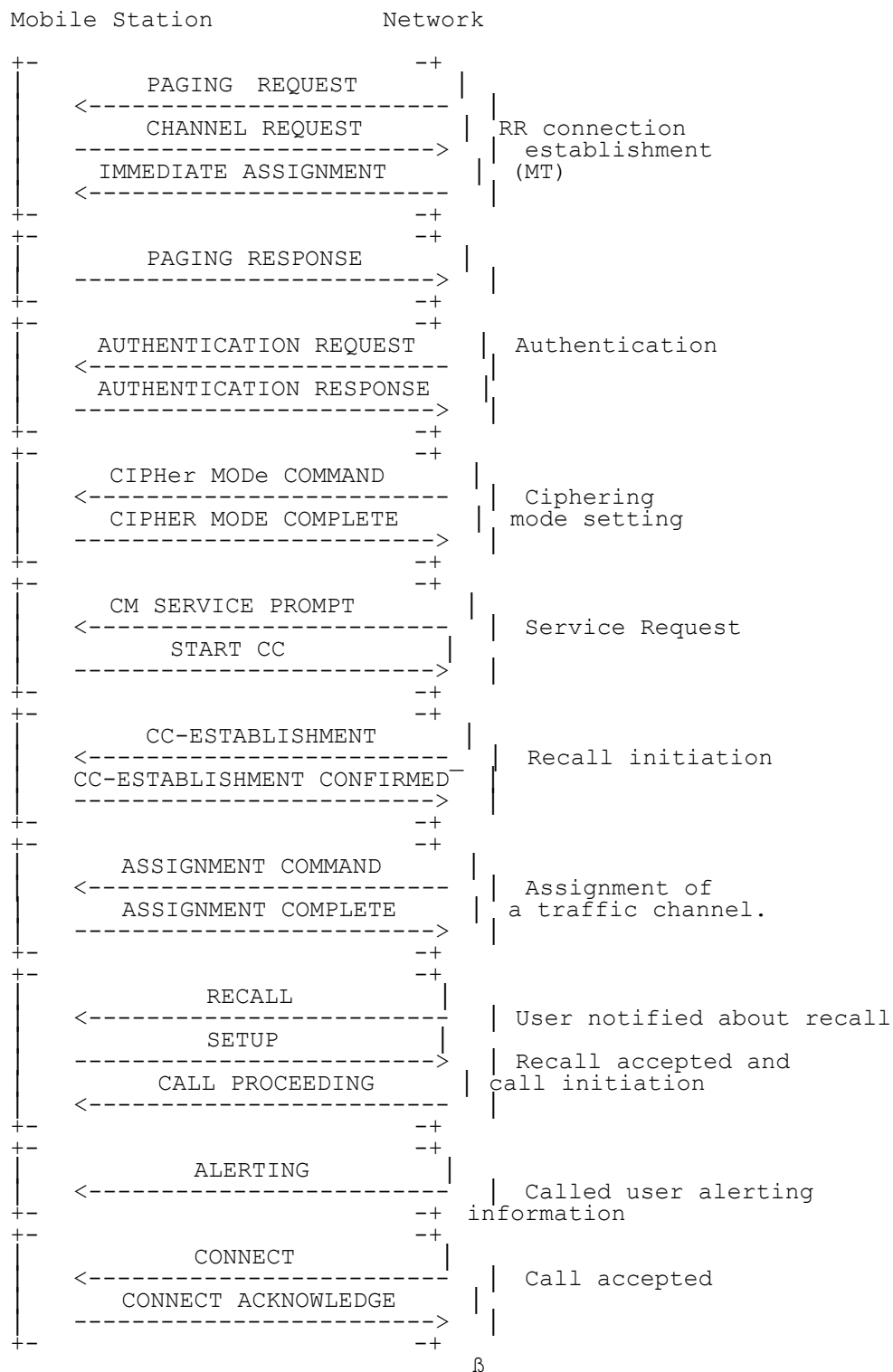
Figure 7.19/3GPP TS 23.108: Network initiated mobile originating call establishment with assignment before A party alerting
