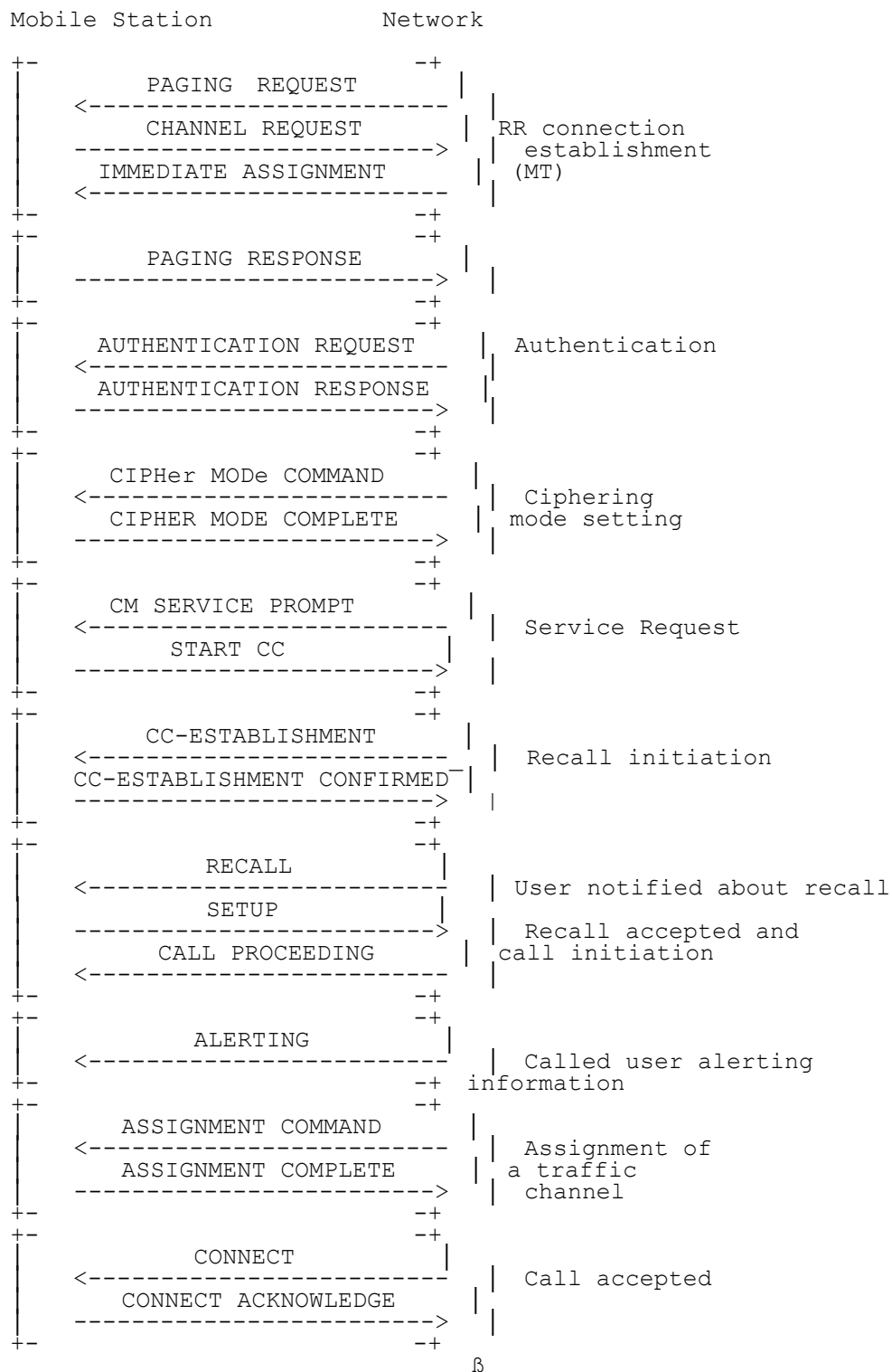
Figure 7.21/3GPP TS 23.108: Network initiated mobile originating call establishment with assignment after A and B party alerting
