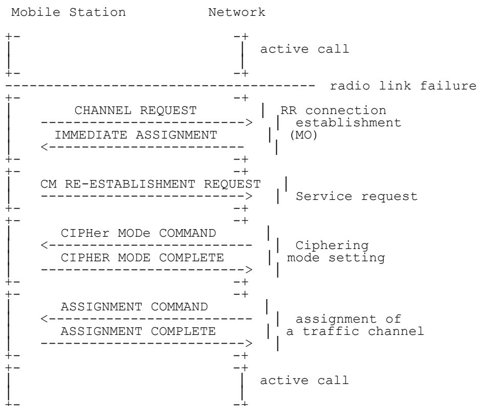
Figure 7.18/3GPP TS 23.108: Call re-establishment
