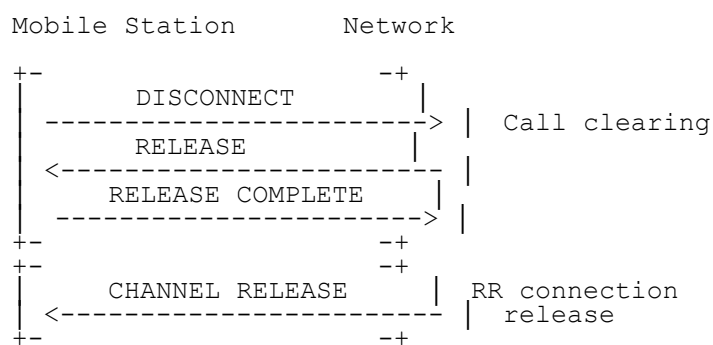
Figure 7.12b/3GPP TS 23.108: Call clearing
