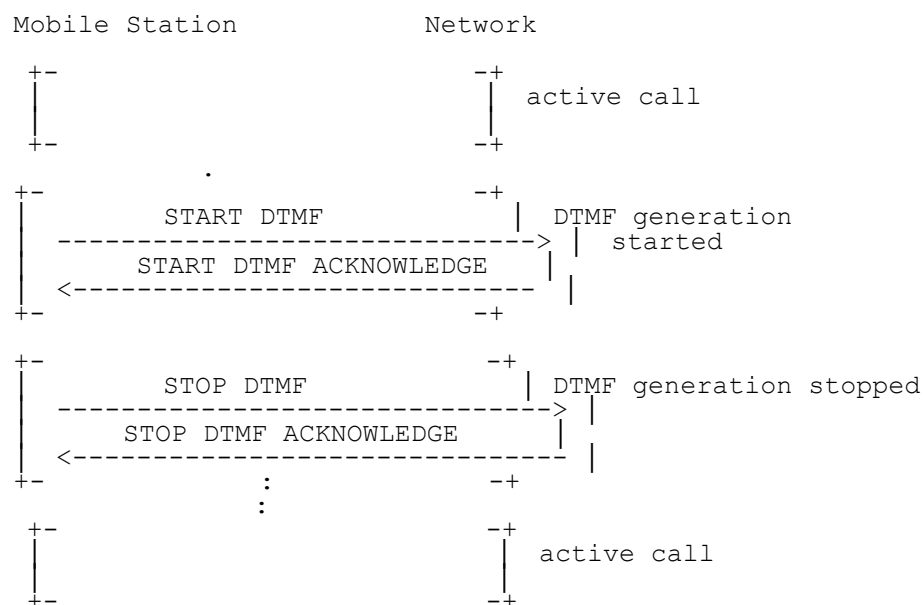
Figure 7.13/3GPP TS 23.108: DTMF protocol control
