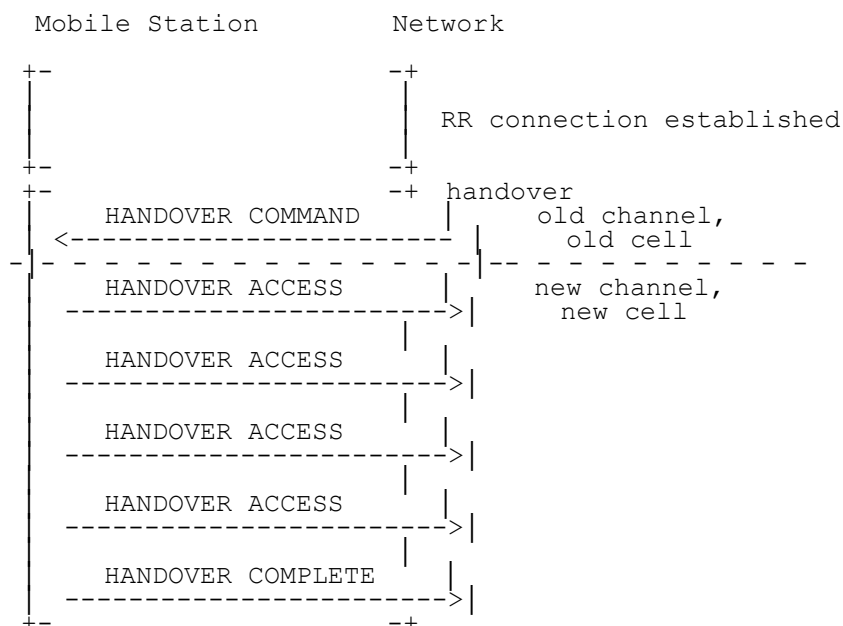
Figure 7.14/3GPP TS 23.108: Handover to a finely synchronized cell, successful case
