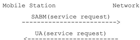
Figure 7.4/3GPP TS 23.108: Service request and contention resolution
