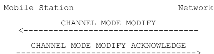
Figure 7.7/3GPP TS 23.108: Channel mode change
