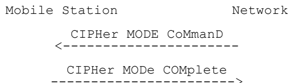
Figure 7.6/3GPP TS 23.108: Ciphering mode setting
