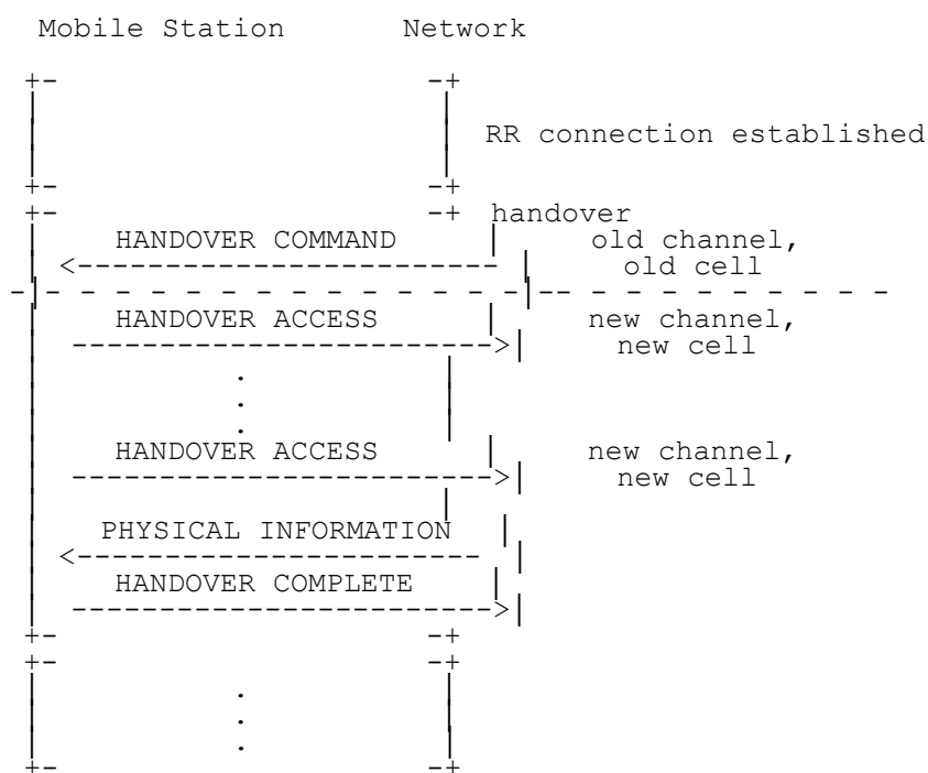
Figure 7.15/3GPP TS 23.108: Handover to a non-synchronized cell, successful case
