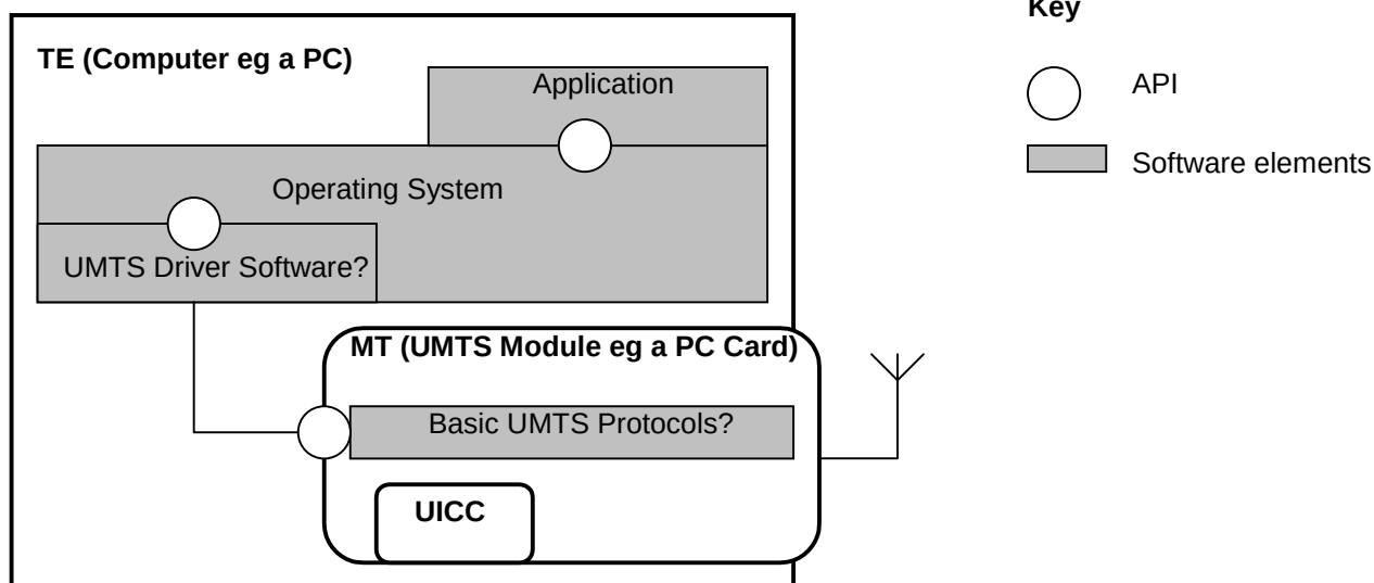
Figure 3: Assumed Topology
