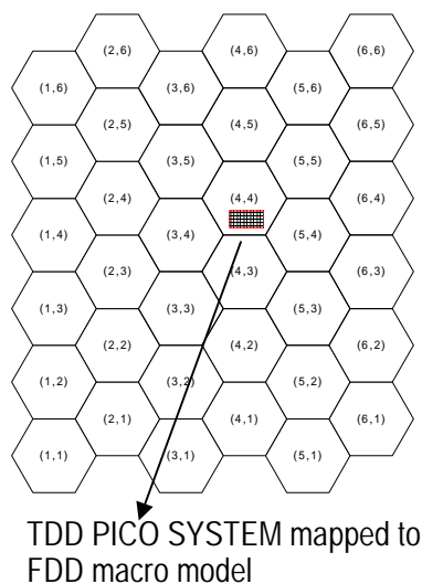
Figure 31D: TDD pico and FDD Macro evaluation layout; pico model chosen from [31]
