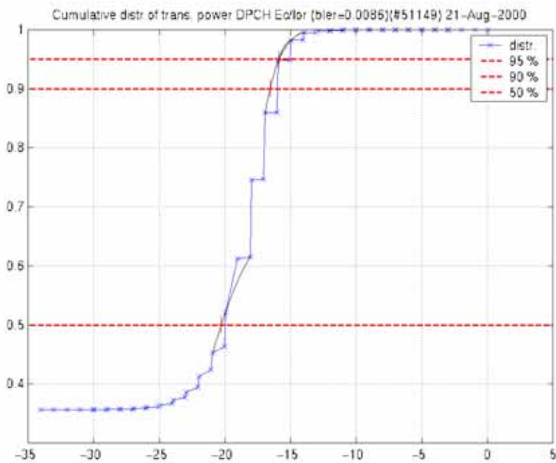
Figure 56: Cumulative distribution of transmission power DPCH_Ec/Ior when compressed mode is on. TGL = 4 slots
