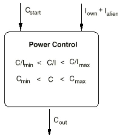
Figure 11: C/I based Power Control algorithm
