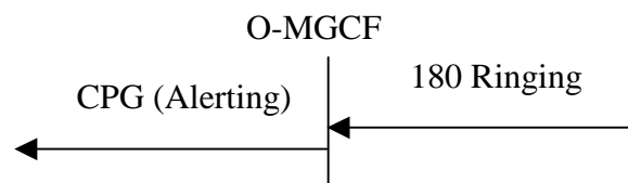
Figure 18: Sending of CPG(Alerting)
