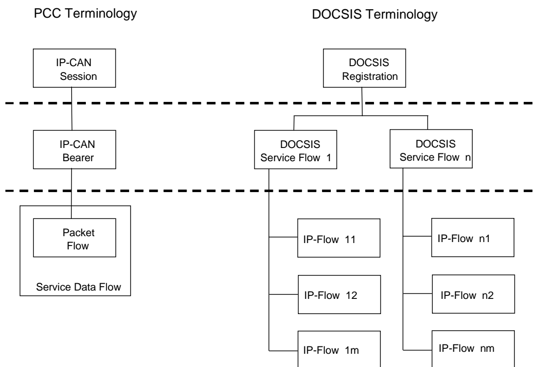
Figure D.1.2: PCC to DOCSIS terminology mapping
