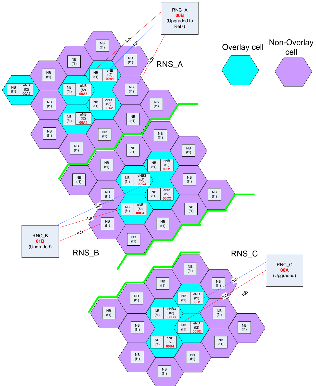
Figure 7.4.4-1: Valid RNC ID Configuration Example
