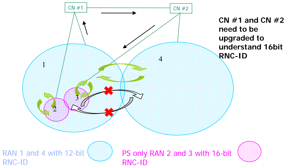
Figure 7.4.3-2: Configuration example for Rule 1 and 2.
