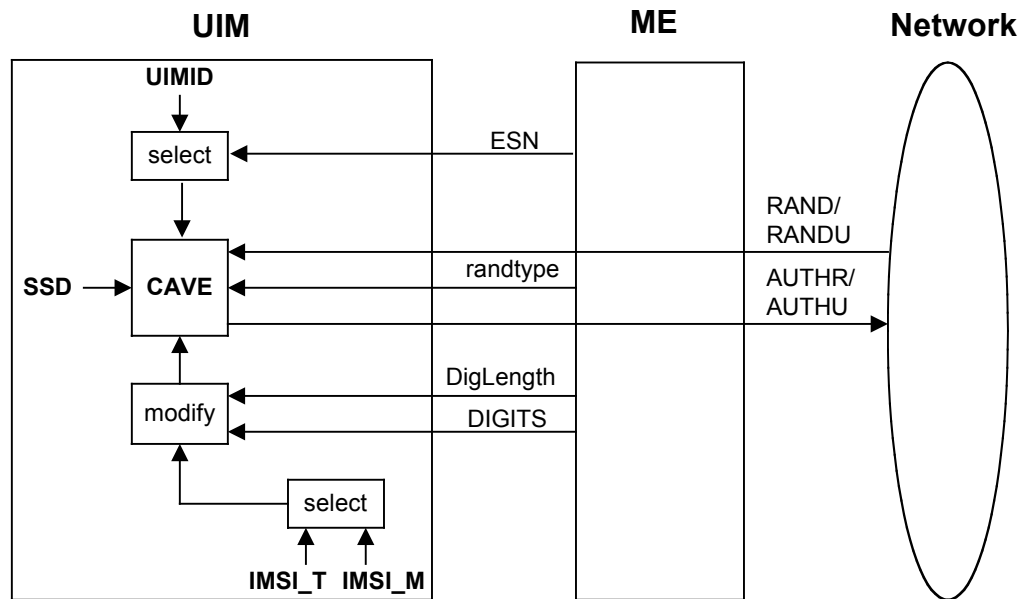
Figure 4.2.2-1. Run CAVE Function
