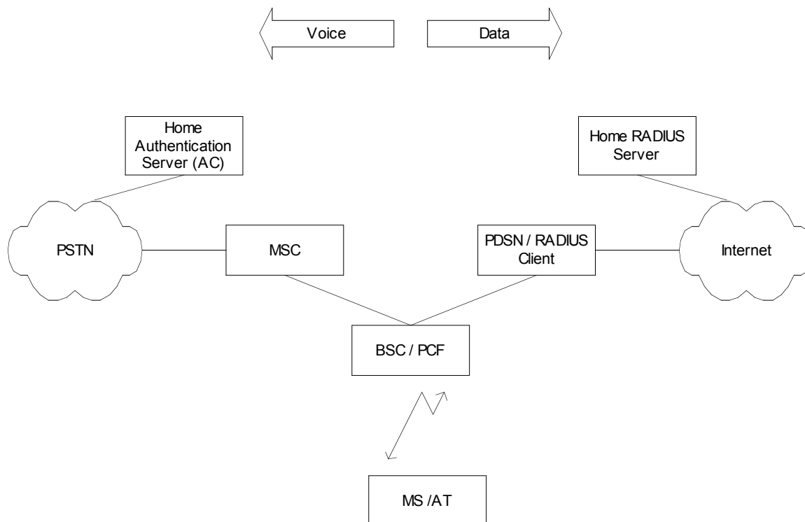
Figure 4.7-1. Authentication Models
