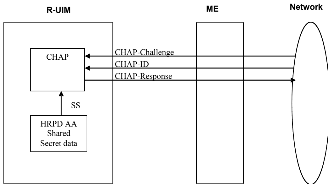
Figure 4.7.4-1. HRPD Access Authentication Command
