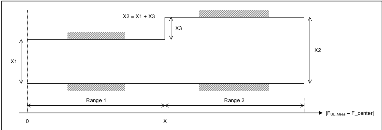
Figure 6.4.2.5-1: The limits for EVM equalizer spectral flatness with the maximum allowed variation. F_{center} denotes the center frequency of the allocated block of PRBs.
