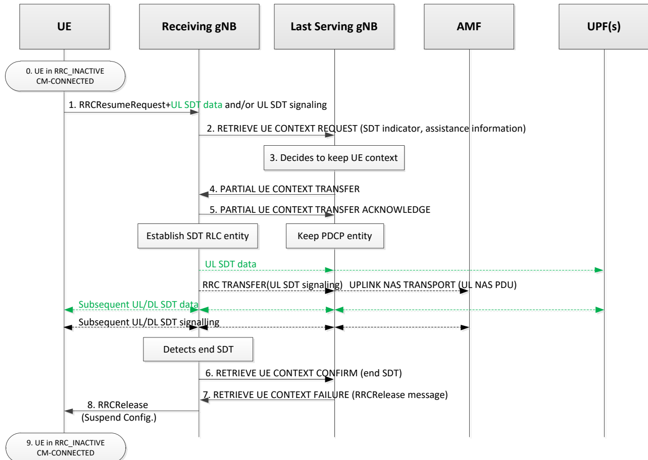
Figure 18.3-1. RA-based SDT without UE context relocation
