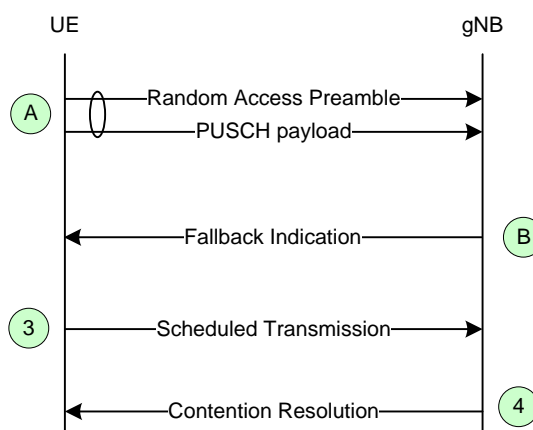
Figure 9.2.6-2: Fallback for CBRA with 2-step RA type
